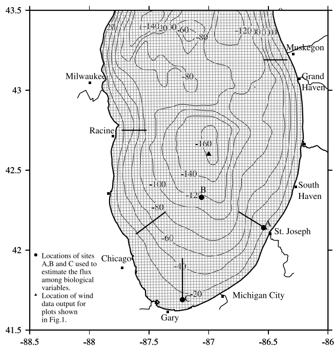
Figure 2. Bathymetry (thin solid curved lines) and model grids in southern Lake Michigan. Heavy solid straight lines represent the cross-isobath transects near the Muskegon, St. Joseph, Gary, Chicago, and Racine. Heavy solid curved lines indicate the river path terminated around the lake. Solid dots are the locations of sites A, B, and C used to estimate the flux among biological variables in the food web, and solid triangles are location of the wind data output for the plots shown in Figure 1.
