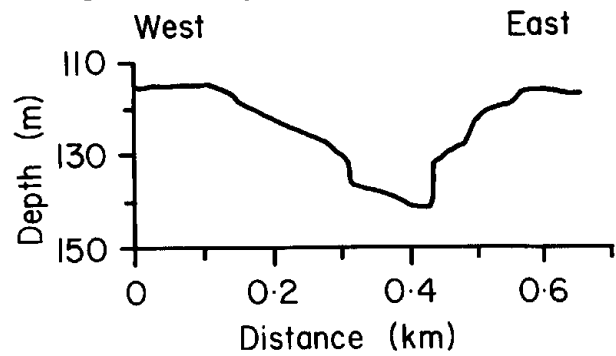
Fig. 2. Line drawing of acoustic profile of axial channel. Vertical exaggeration is 10X. See Fig. 1 for location.
