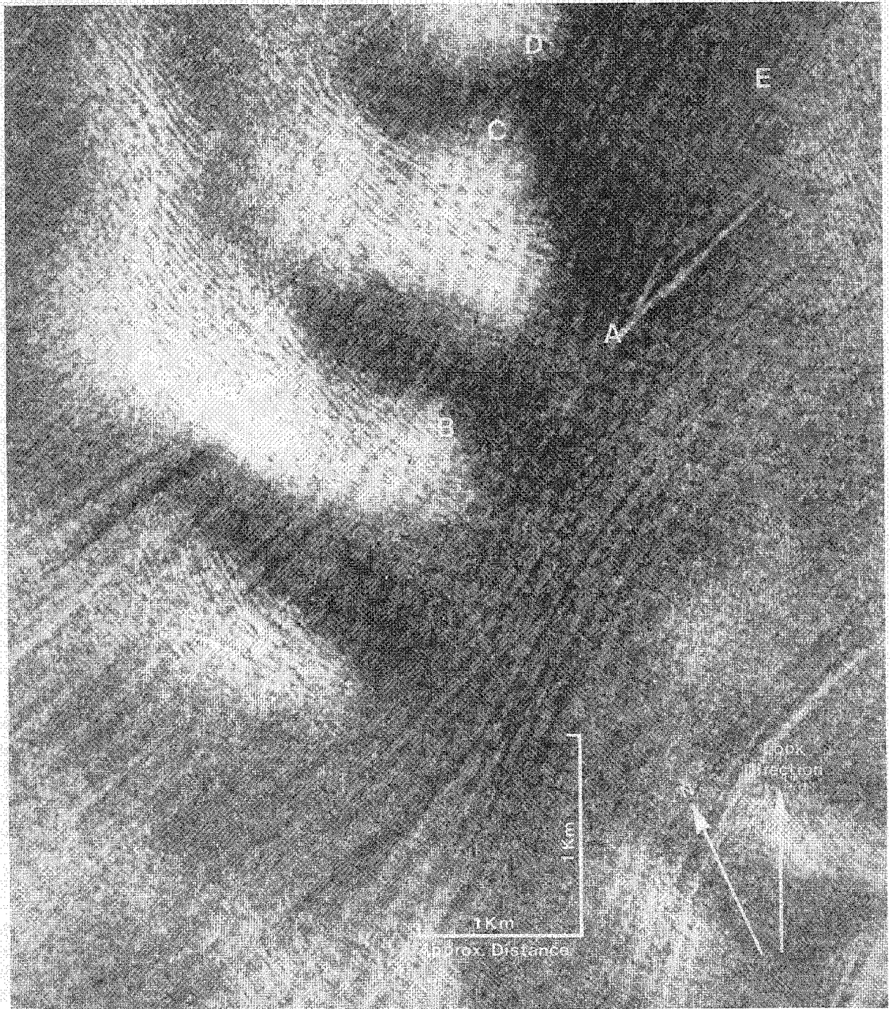
Fig. 2. An enlargement of the area outlined in the rectangle in Figure 1. The tip of the moraine (A) was the base station for a doppler geociever and served as the starting point for four planetable/alidade profiles across (A to B, C, and D) and along (A to E) the northeast trending swale. This swale, seen as a dark area on the image because of low radar backscatter, had a relief of more than 40 m. The four dark, elliptical, cirque-like patterns on the left flank of the swale are bounded by bright-return topographic highs. The swales are zones with few crevasses, while the highs are characterized by an extensive crevasse network. The scales parallel and perpendicular to the look direction are different due to SLAR imaging anomalies.
