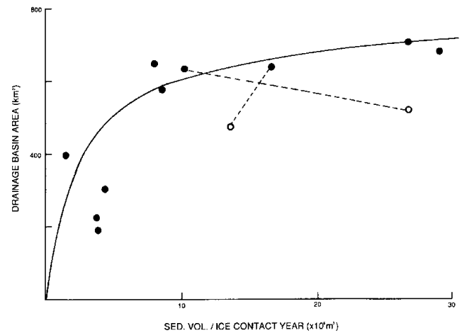
Fig. 3. Sediment volume in ice-proximal basins estimated from seismic profiles (from Molnia et al. 1984) averaged over the period of time Muir Glacier remained in or at the head of each basin, plotted against the successive areas of Muir Glacier's drainage basin (determined from Brown et al. 1982). The plot shows the relationship during recent retreat of the glacier.
