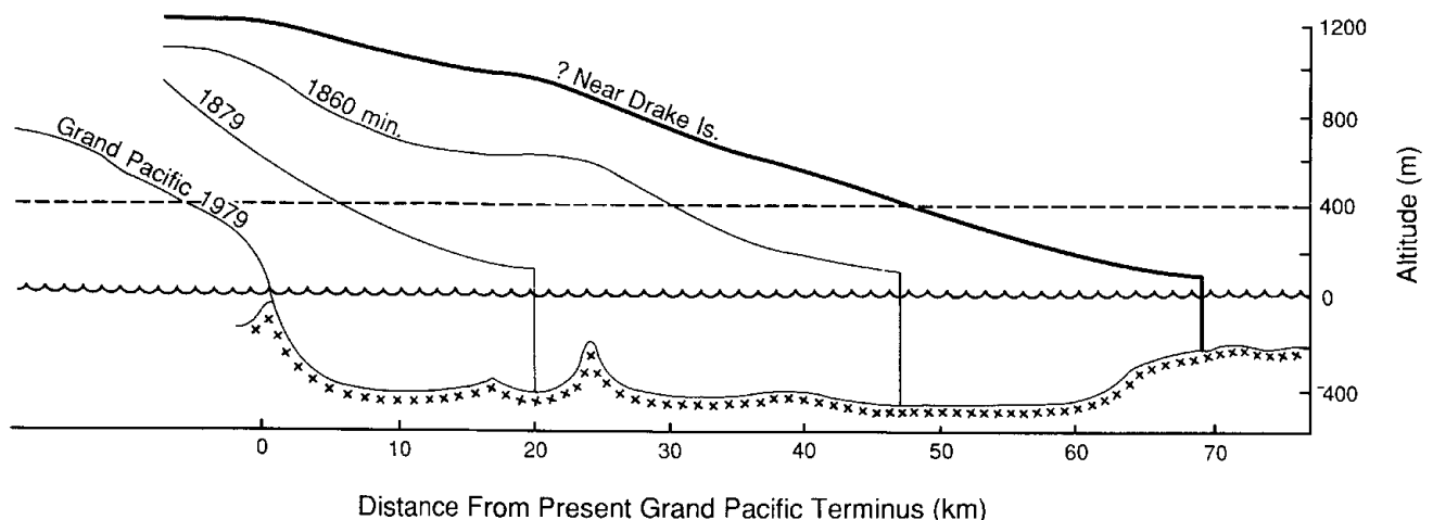
Fig. 2. A series of longitudinal surface profiles and assumed bed profiles (from seismic reflection) of the west arm of Glacier Bay since glacial retreat from near Tlingit Point. The dashed line is an equilibrium line at 400 m altitude, and surface area of the glacier below that line changes during retreat without moving the ELA. Profiles based on Brown et al. (1982).
