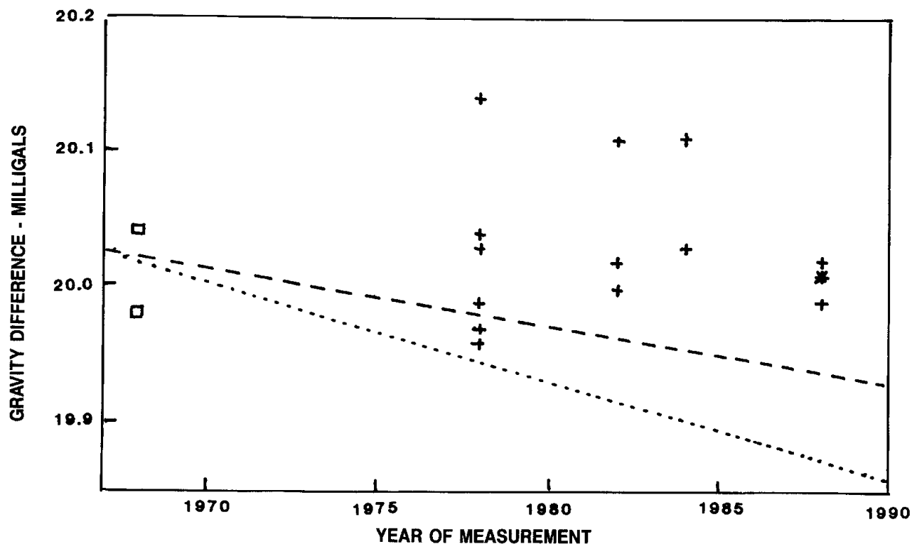
Fig. 3. Graph of measurements of the gravity difference between Juneau and Gustavus airports as a function of year of measurement. Dotted line indicates expected free-air gravity change (no addition of mass beneath uplifted station) of 2.35 cm/year for Gustavus relative to Juneau airport. Dashed line indicates expected Bouguer gravity change with addition of underlying infinite slab of mantle material having a density of 3.10 gm/cm 3 .
