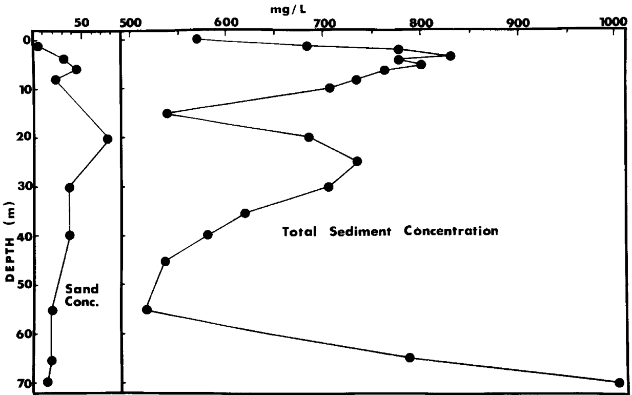
Fig. 3. Suspended sediment concentrations and sand concentrations at a station 400 m from McBride Glacier on July 12, 1986.
