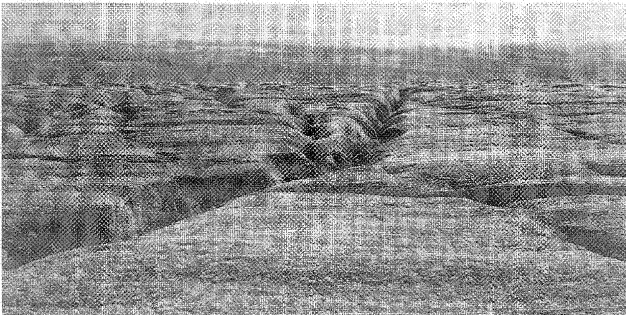
Fig. 6. Photograph looking approximately east up the slope of a topographic high located near the second (C) from the west shown in Fig. 1. The direction of glacier flow is toward the observer. A rectilinear pattern of crevasses is present on many of the slopes of the topographic highs.
