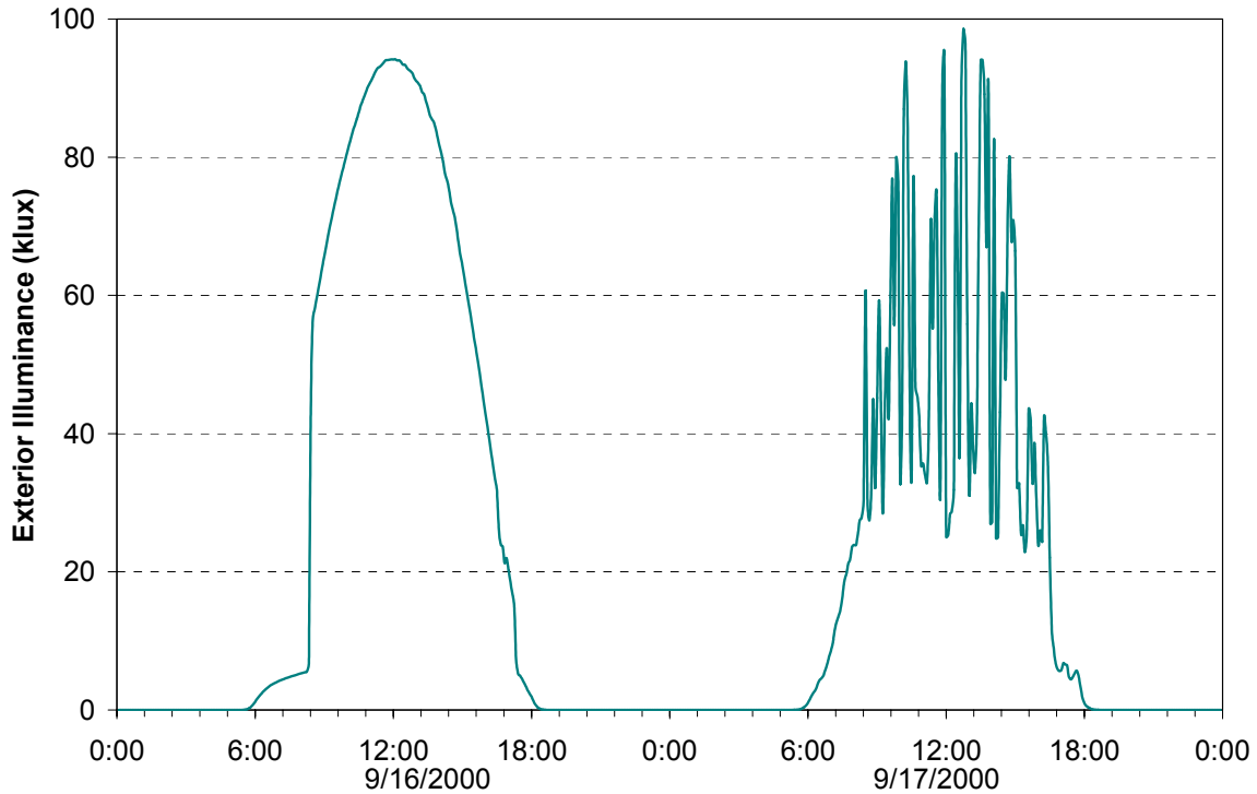
Figure 7-11 Exterior illuminance for September 16 and 17, 2000
