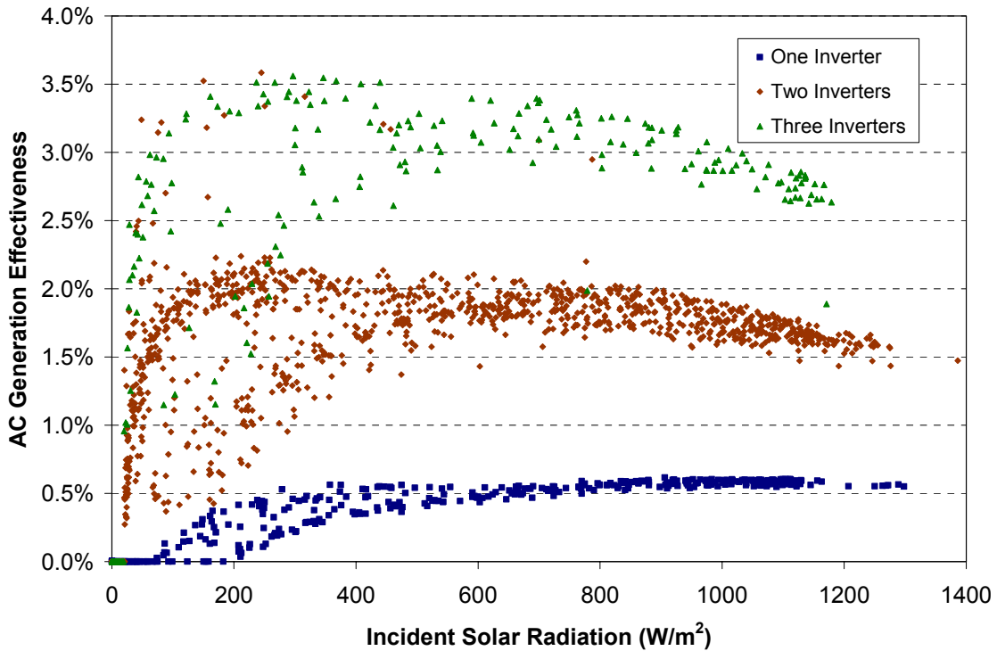
Figure 7-22 AC Generation Effectiveness for June 2003 with 1, 2, or 3 inverters operating
