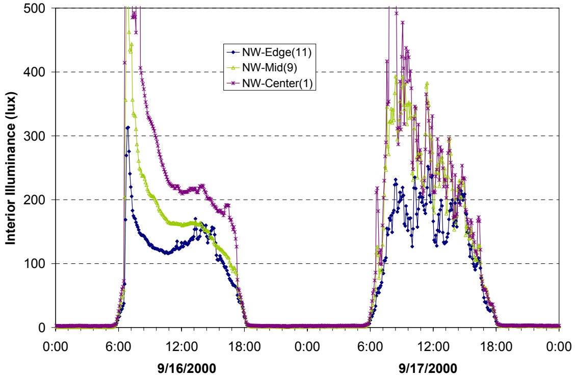
Figure 7-13 Daylight levels on the north side of the retail area for clear and partly cloudy autumn days (September 16 and 17, 2000)
