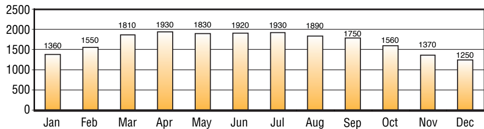
Average incident solar radiation data for San Juan, Puerto Rico (Btus/square foot/day)
