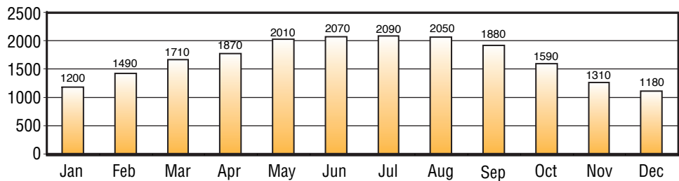
Average incident solar radiation data for Honolulu, Hawaii (Btus/square foot/day)
