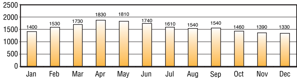
Average incident solar radiation data for Guam (Btus/square foot/day)
