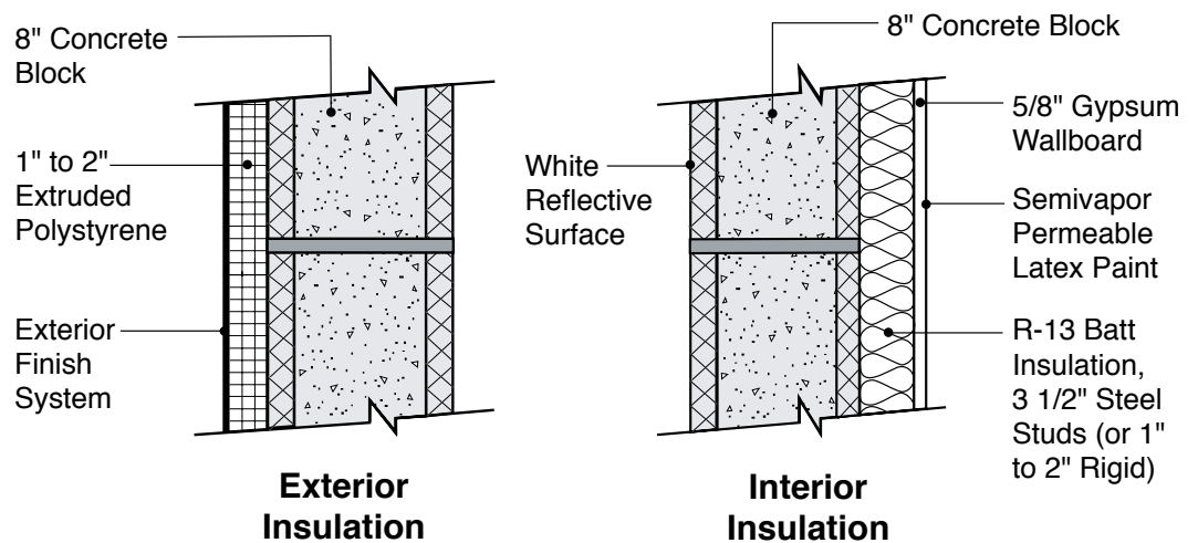
Wall Sections
