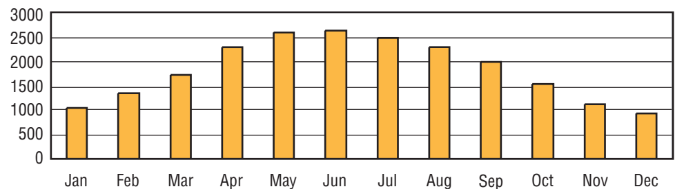
Average Incident Solar Radiation in Phoenix (Btus/Square Foot/Day)
