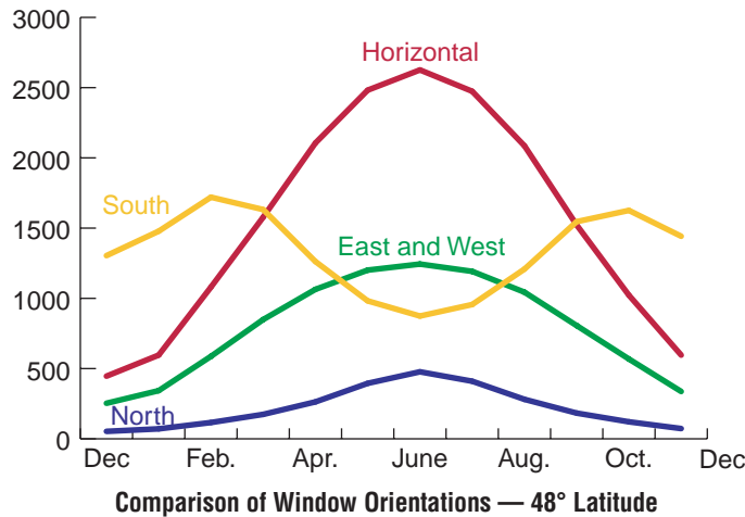
The amount of solar radiation striking windows varies with the surface orientation.
