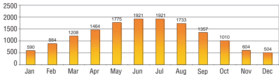
Average Incident Solar Radiation in Boston (Btus/Square Foot/Day)
