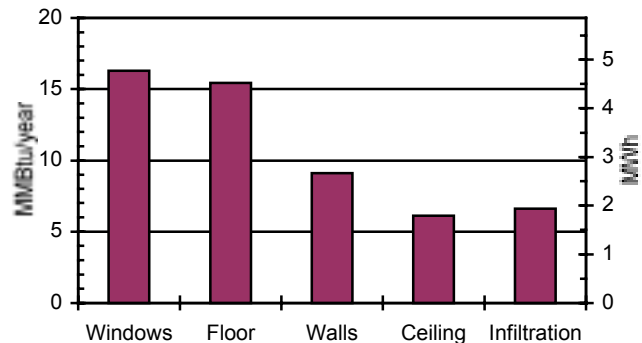
Fig. 7: Primary heat loss paths in improved design simulation.
