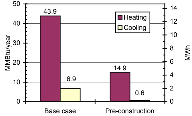
Fig. 1: Base-case and pre-construction model energy load comparison.
