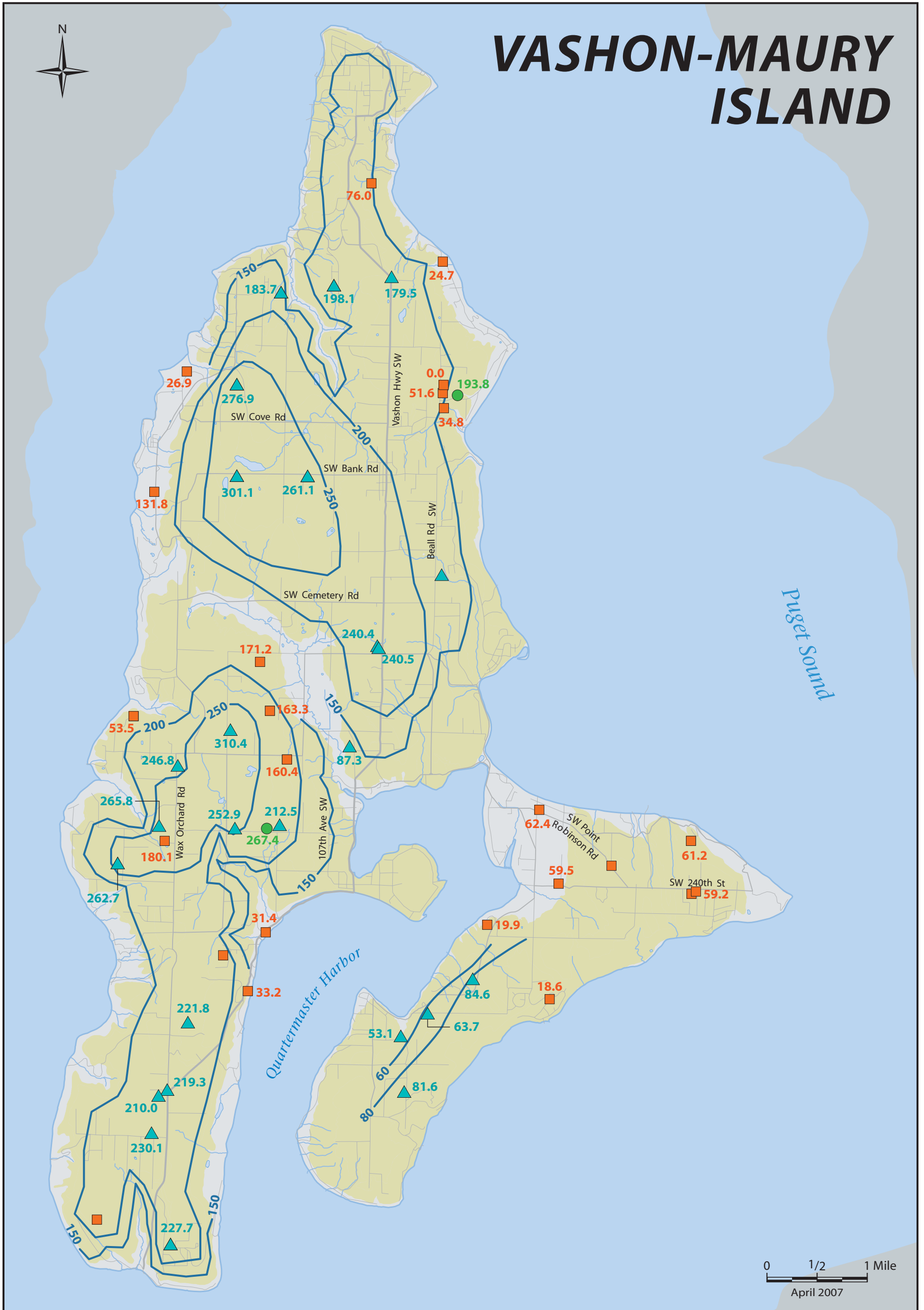
Figure 19 Groundwater Elevations in Vashon Advance Outwash Aquifer
