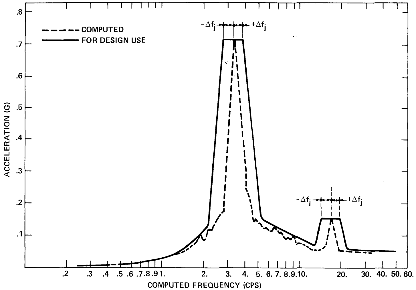
Figure 1 Response Spectrum Peak Broadening and Smoothing
