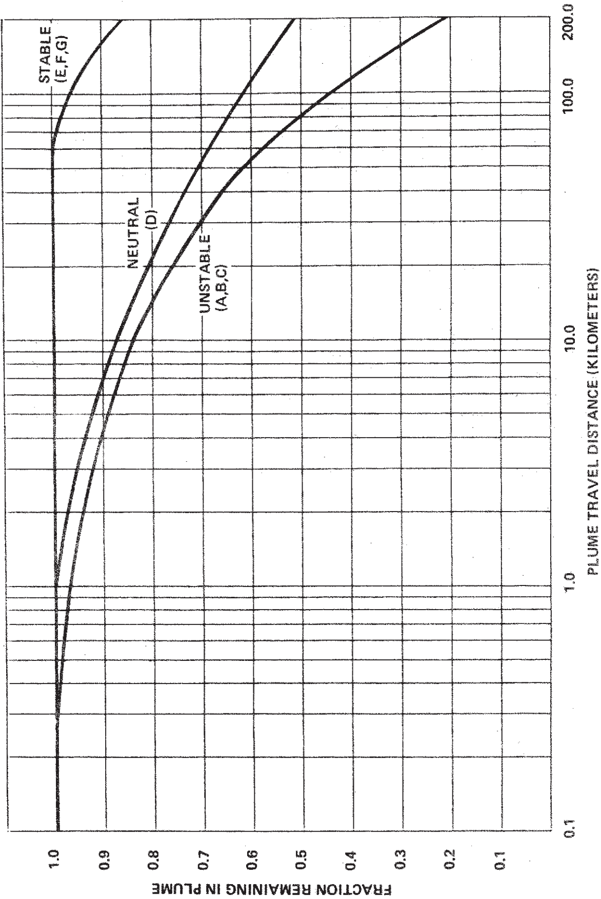
Figure 5. Plume Depletion Effect for 60m Releases (Letters denote Pasquill Stability Class)
