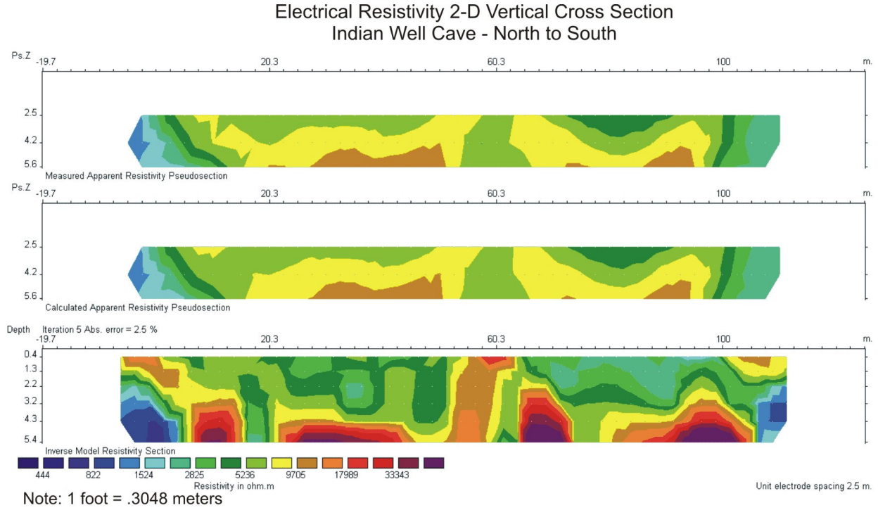
Figure 107. Cross Section. Electrical Resistivity Vertical 2-D.
