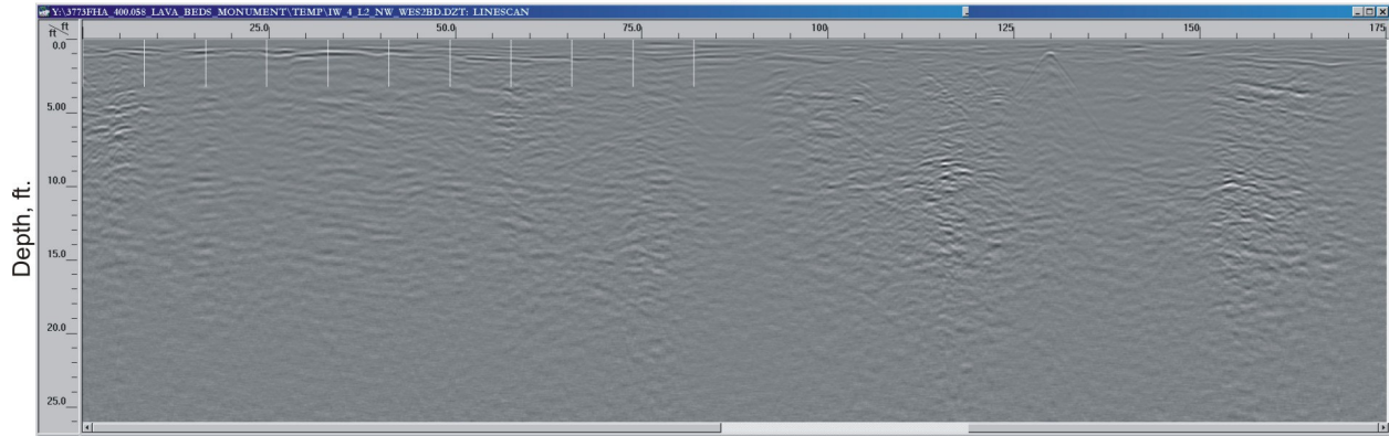
Processed GPR Data 400 MHz Antenna - Line 2 Indian Well Cave Distance, ft.
