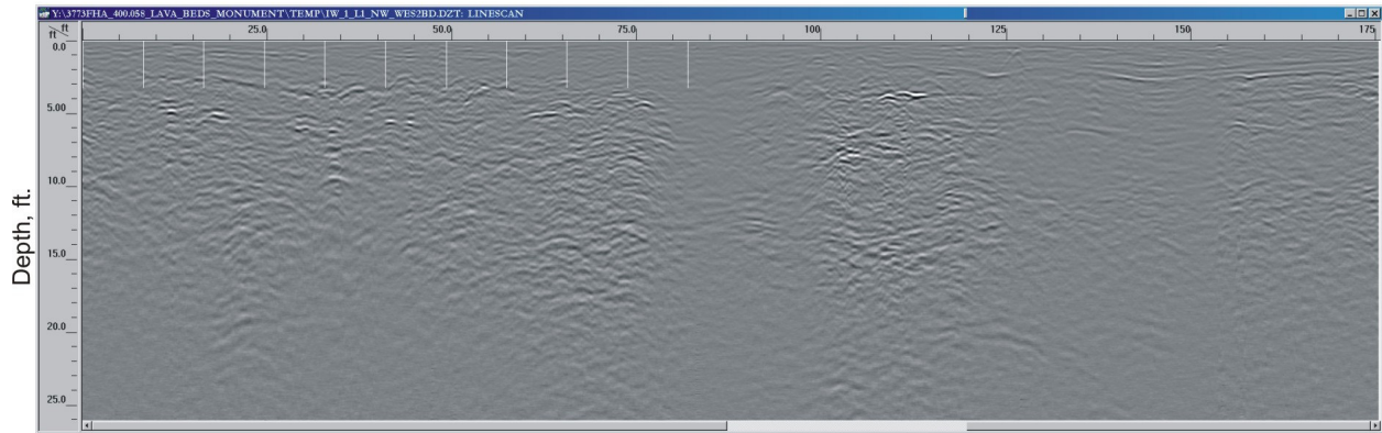
Processed GPR Data 400 MHz Antenna - Line 1 Indian Well Cave Distance, ft.
