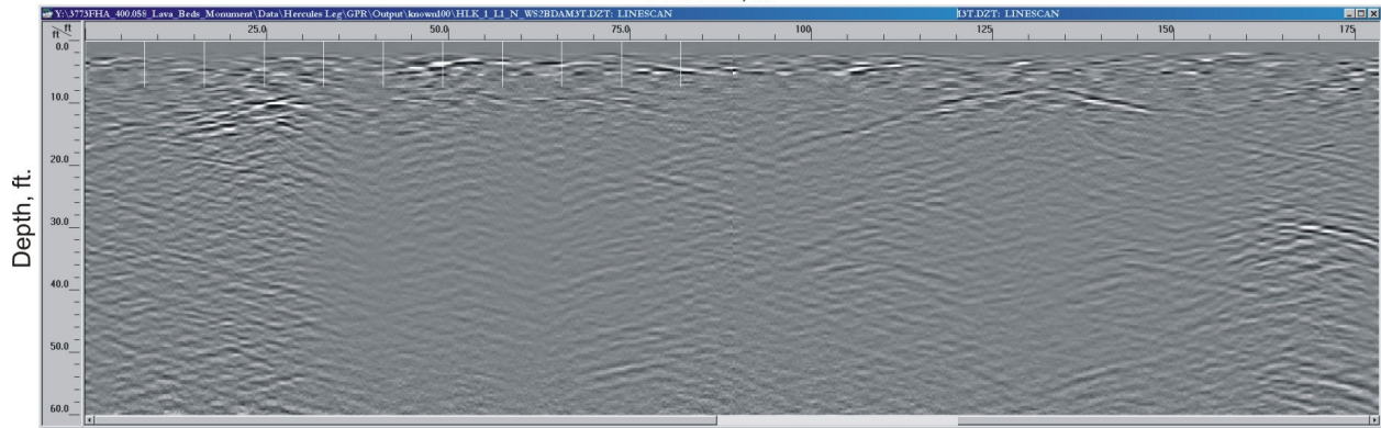
Processed GPR Data 100 MHz Antenna - Line 1 Hercules Leg Cave - Part 1 Distance, ft.
