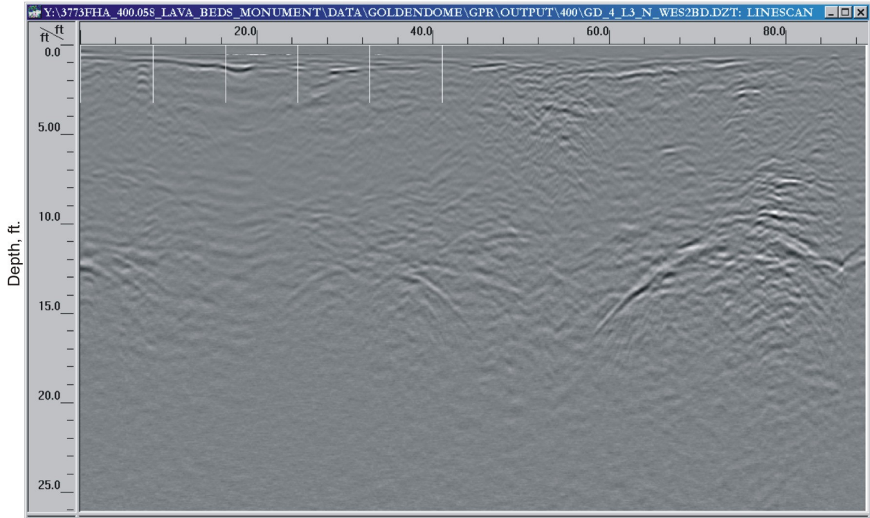
Processed GPR Data 400 MHz Antenna - Line 3 Golden Dome Cave Distance, ft.
