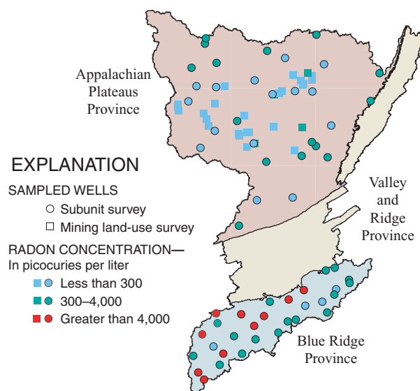
Figure 21. Radon concentrations vary greatly among physiographic provinces.
