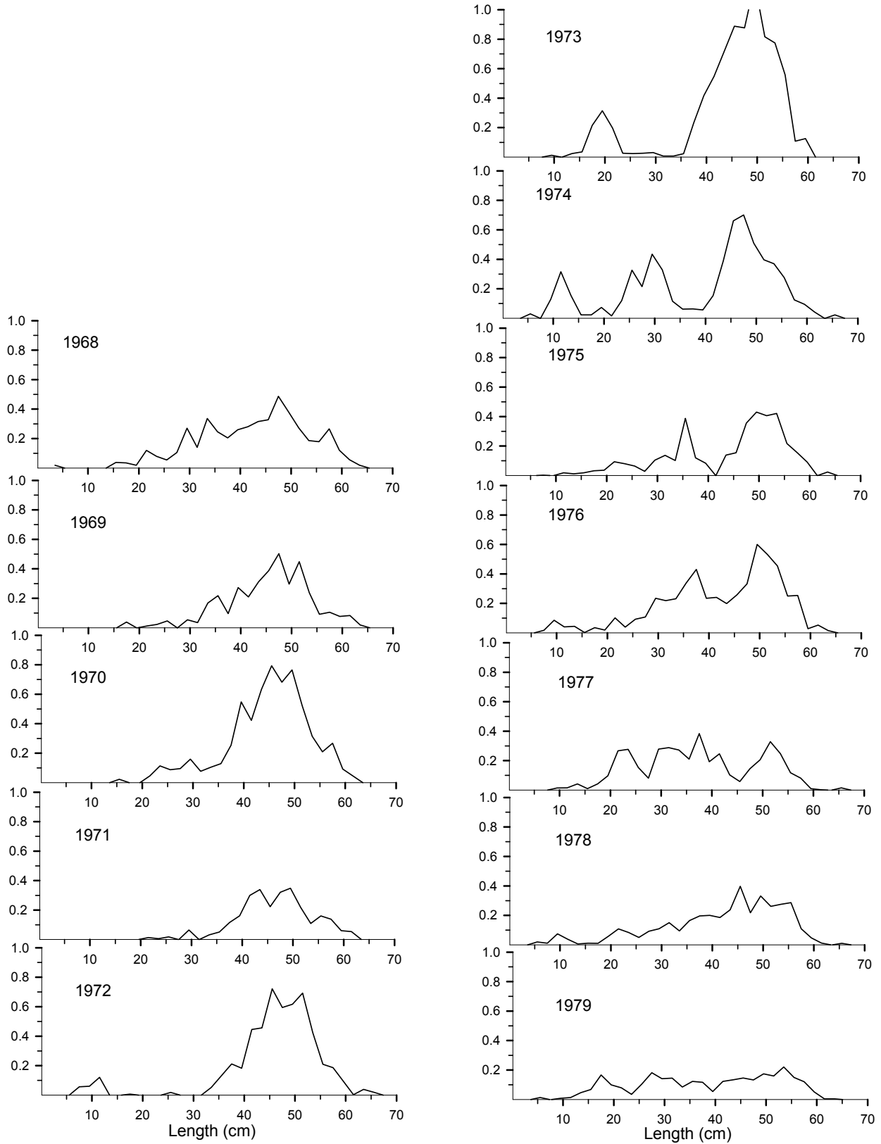
Figure 29. Stratified mean number per tow at length of witch flounder in the NEFSC spring bottom trawl survey, 1968 – 2003.
