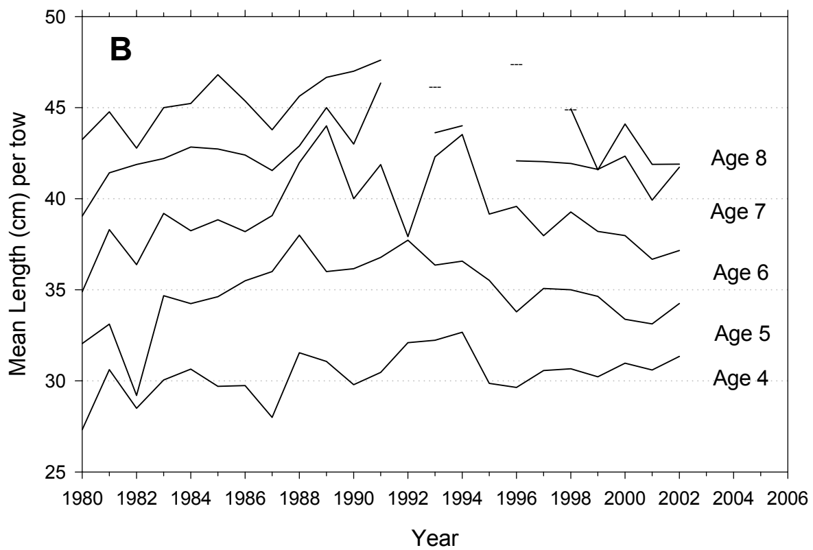
Figure 35. Mean length (cm) at age of witch flounder, age groups 4 -8, in spring (A) and autumn (B) NEFSC bottom trawl surveys, 1980 – 2002, preliminary spring 2003.
