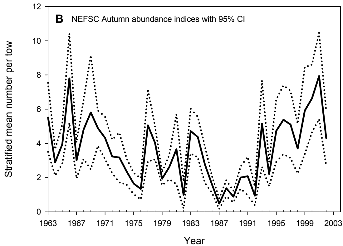
Figure 24. Stratified mean number per tow, with 95% confidence limits, of witch flounder in the NEFSC spring (A) and autumn (B) bottom trawl survey, 1963 – 2003.
