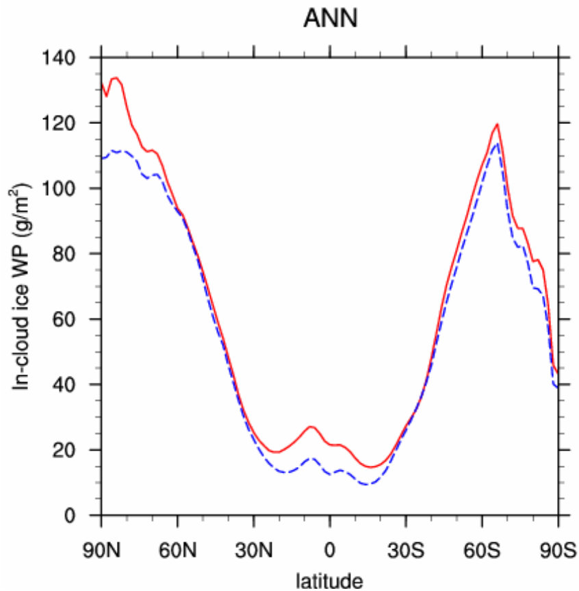
Figure 5. Zonal mean IWP for the tropical (red) and mid-latitude (blue) simulations.
