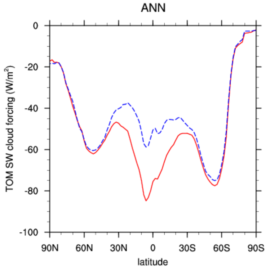
Figure 8. Zonal mean SWCF for the tropical (red) and mid-latitude (blue) SD CAM runs.
