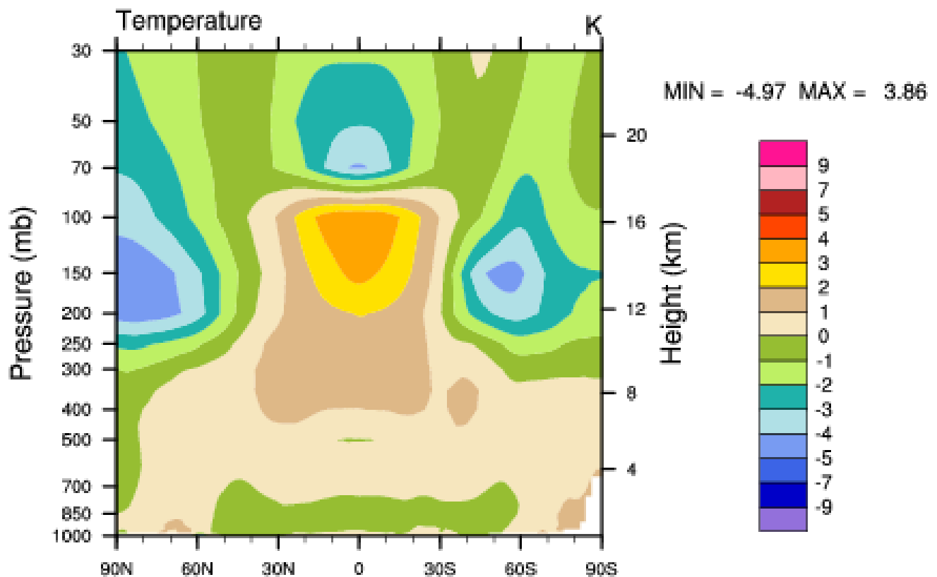
Figure 11. Temperature differences between tropical anvil and mid-latitude SD simulations.
