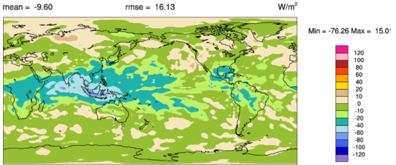
Figure 7. SWCF for the tropical anvil SD run minus SWCF for the mid-latitude SD.
