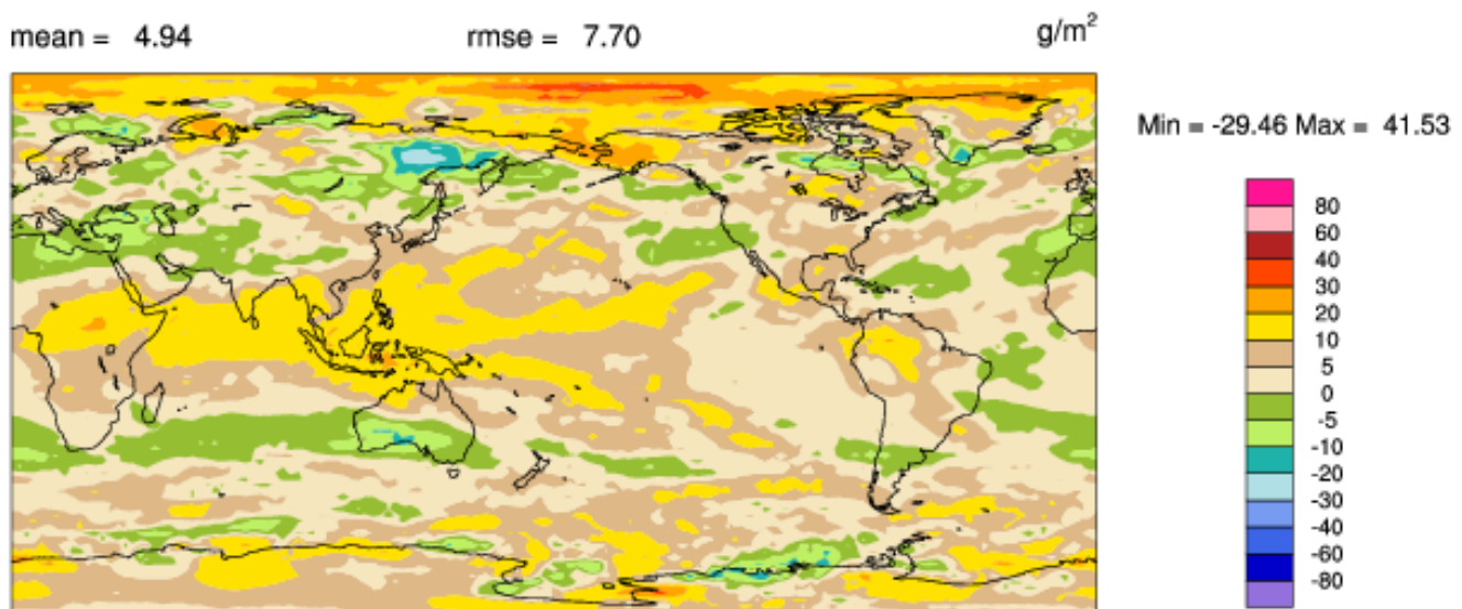
Figure 4. The annual average in-cloud IWP for the tropical SD run minus the mean in-cloud IWP for the mid-latitude SD run.
