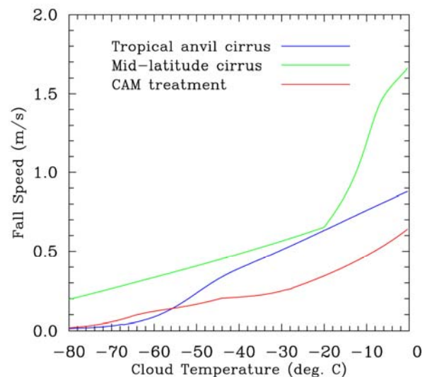
Figure 3. Comparison of ice mass sedimentation rates for tropical anvil and mid-latitude cirrus clouds and the sedimentation rates currently predicted by the CAM.
