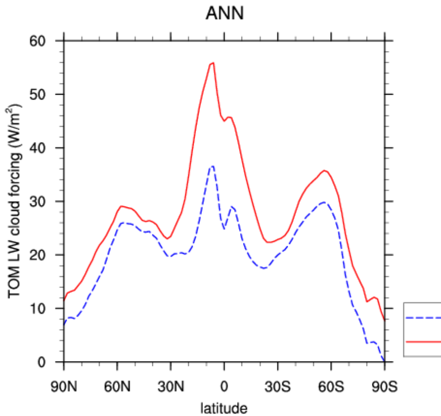
Figure 10. Zonal mean LWCF for the tropical (red) and mid-latitude (blue) CAM runs.
