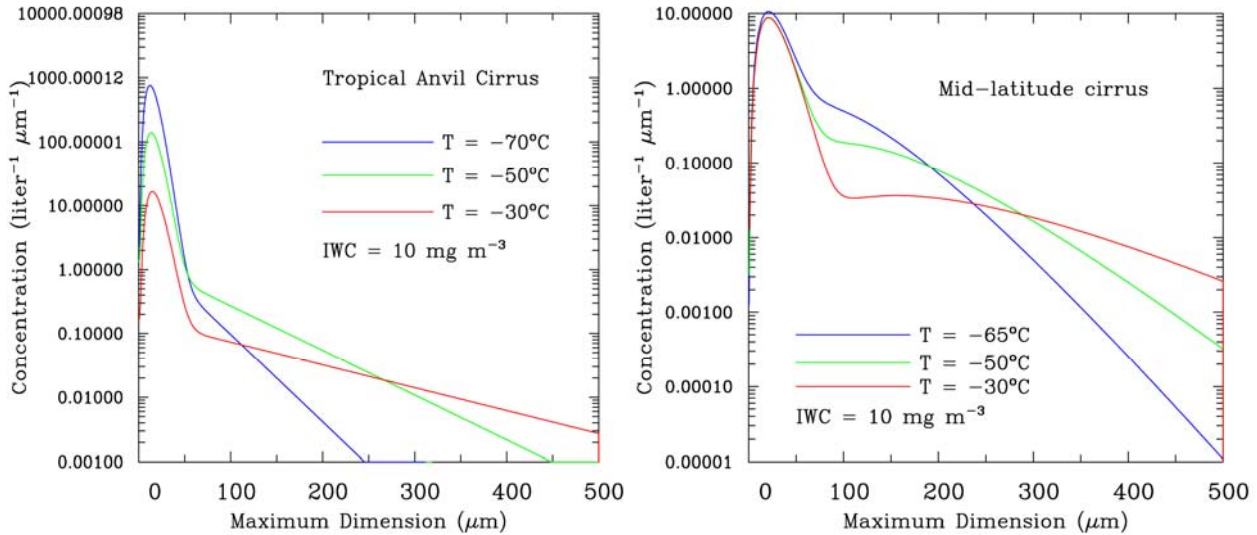
Figure 1. Examples of particle size distribution (PSD) from the mid-latitude cirrus and the tropical anvil cirrus schemes, which are diagnosed as a function of temperature and ice water content.
