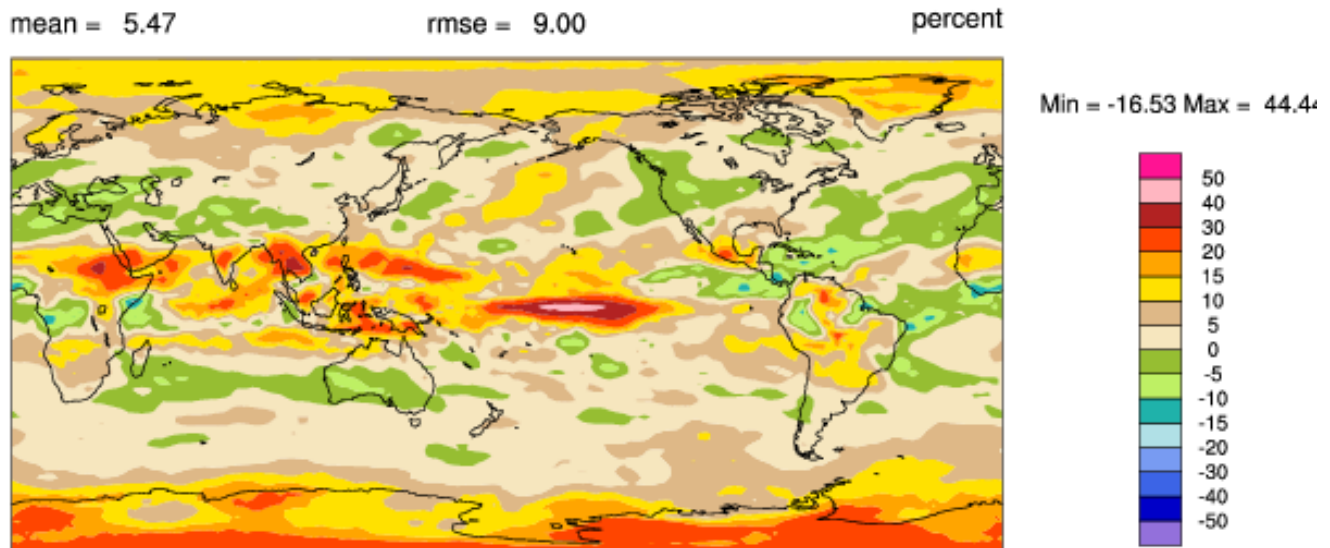
Figure 6. Annual average cirrus cloud coverage for the tropical SD simulation minus that for the mid-latitude SD simulation, SD shown as percent difference.
