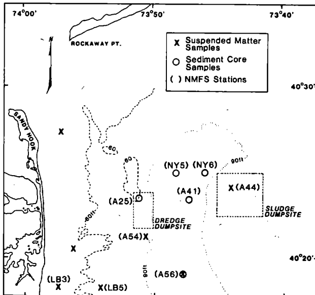
Figure 13. Sampling locations occupied in 1987 for suspended matter and long core samples. The Hudson Shelf Valley lies within the 90-ft (30-m) contours. NOAA stations are shown in parentheses. X = suspended matter; O = sediment core samples.
