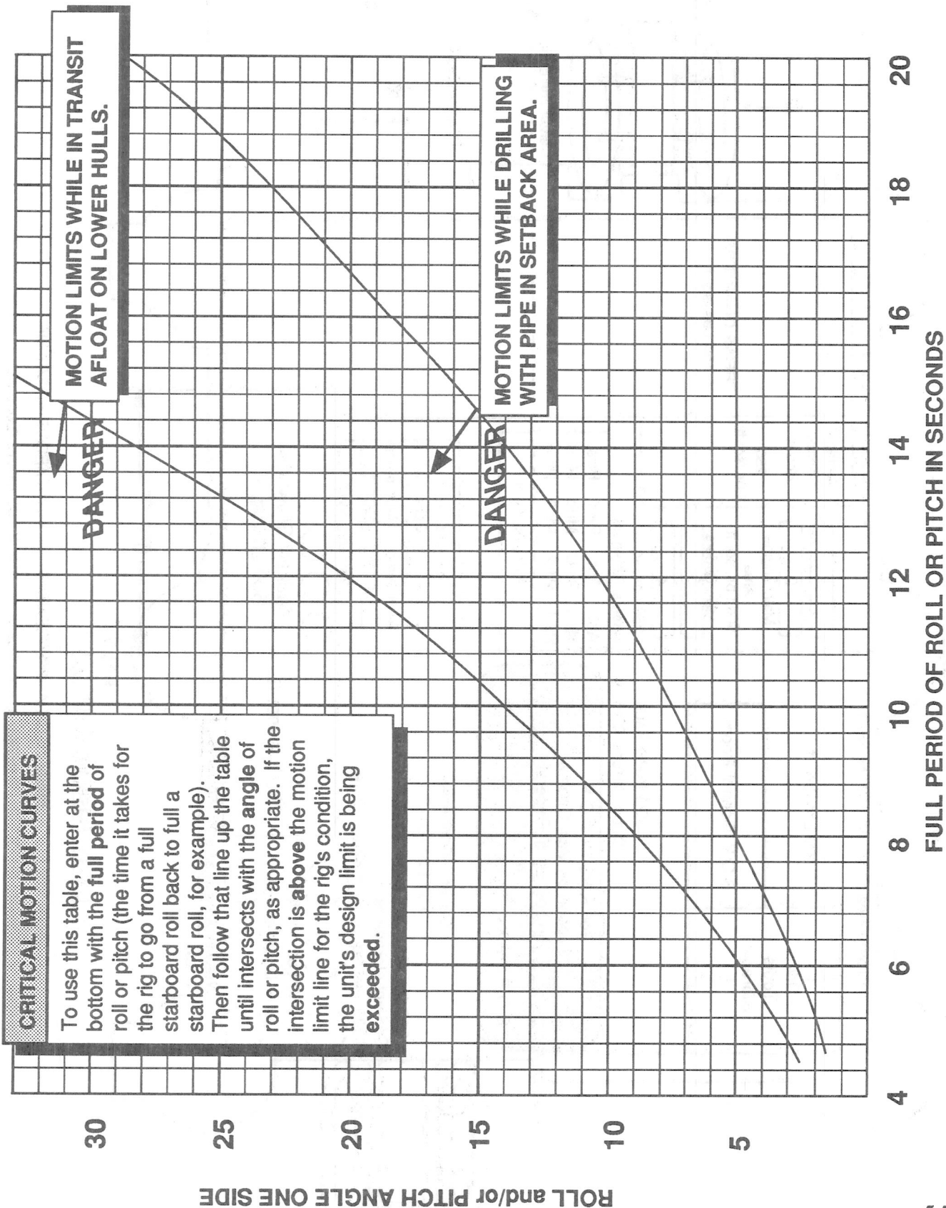
Figure 5 CRITICAL MOTION CURVES
