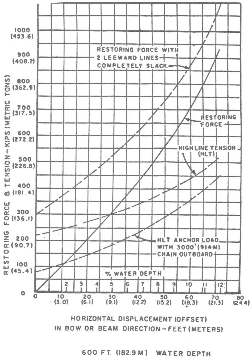
Figure 19 Mooring Analysis - 600 foot water depth
