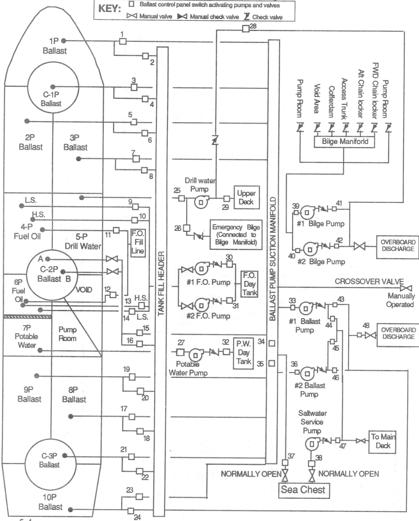
Figure 3a - Ballast Control Panel Mimic Diagram - Port
