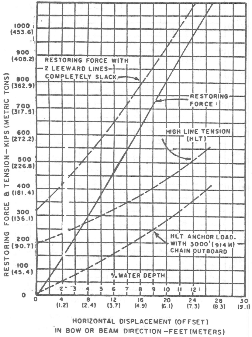
Figure 17 Mooring Analysis - 200 foot water depth
