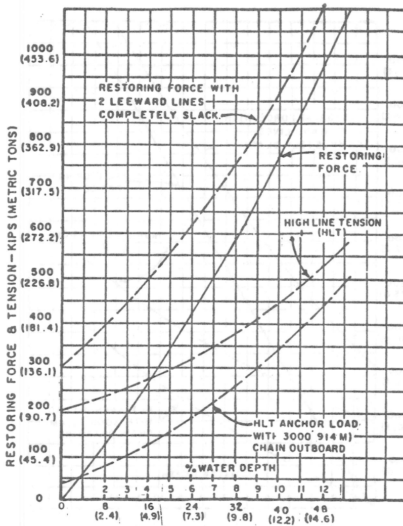
Figure 18 Mooring Analysis - 400 foot water depth
