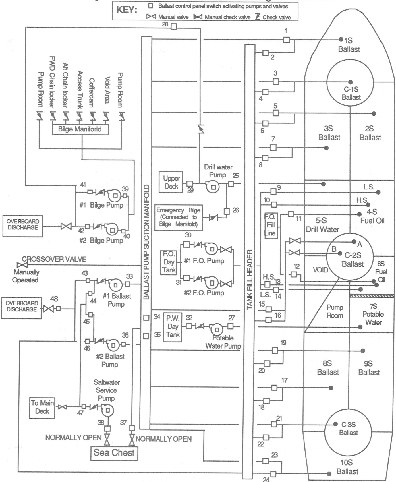
Figure 3b - Ballast Control Panel Mimic Diagram - Starboard
