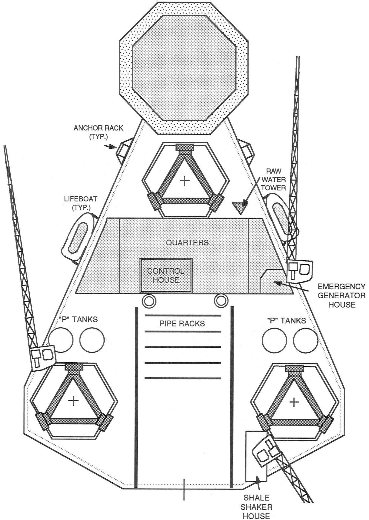
Figure 2 Main Deck - Coastal Driller
