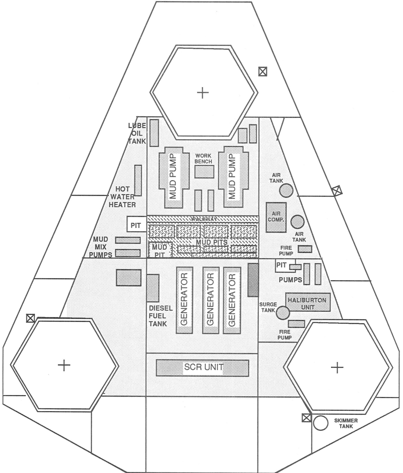
Figure 4 MACHINERY DECK LAYOUT
