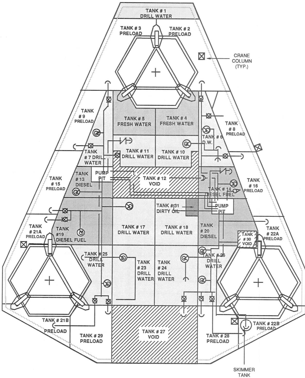
Figure 3 INNER BOTTOM TANK LAYOUT BILGE SUCTION PIPING
