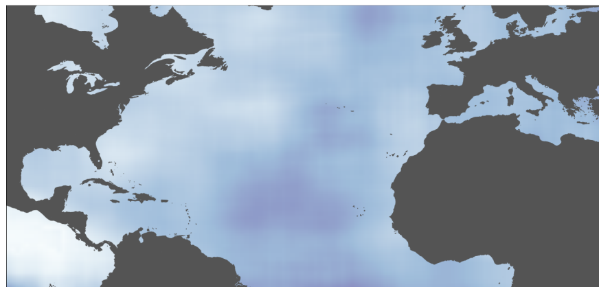
Cloud Top Pressure (millibar)
