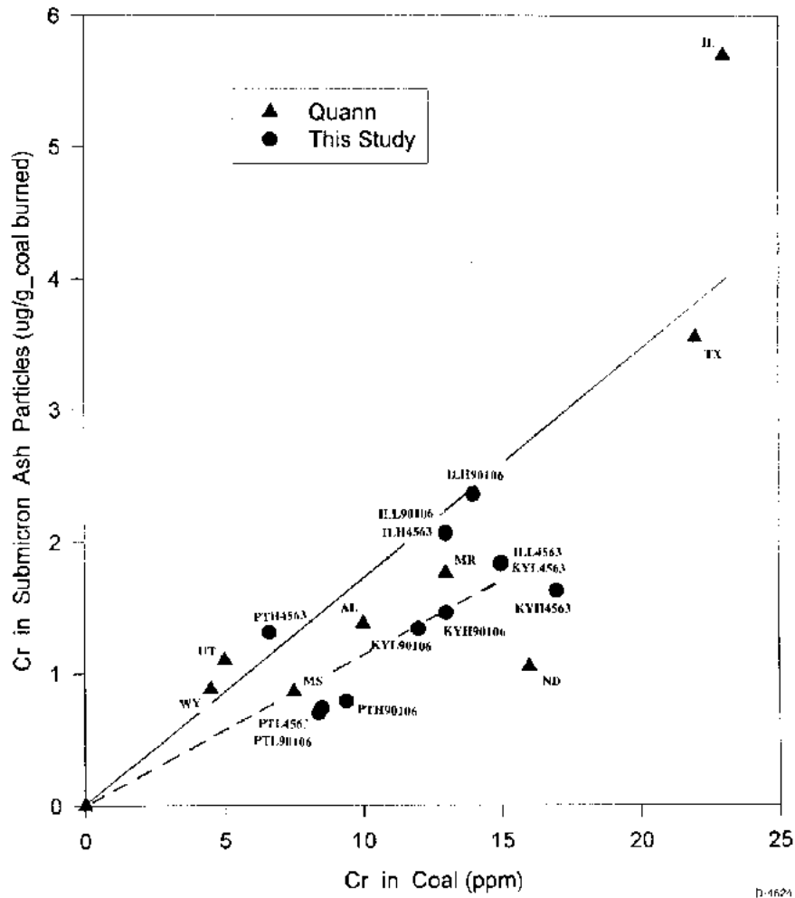
Figure 3-17. Effect of Cr concentration in coal on the total Cr collected in submicron ash.
