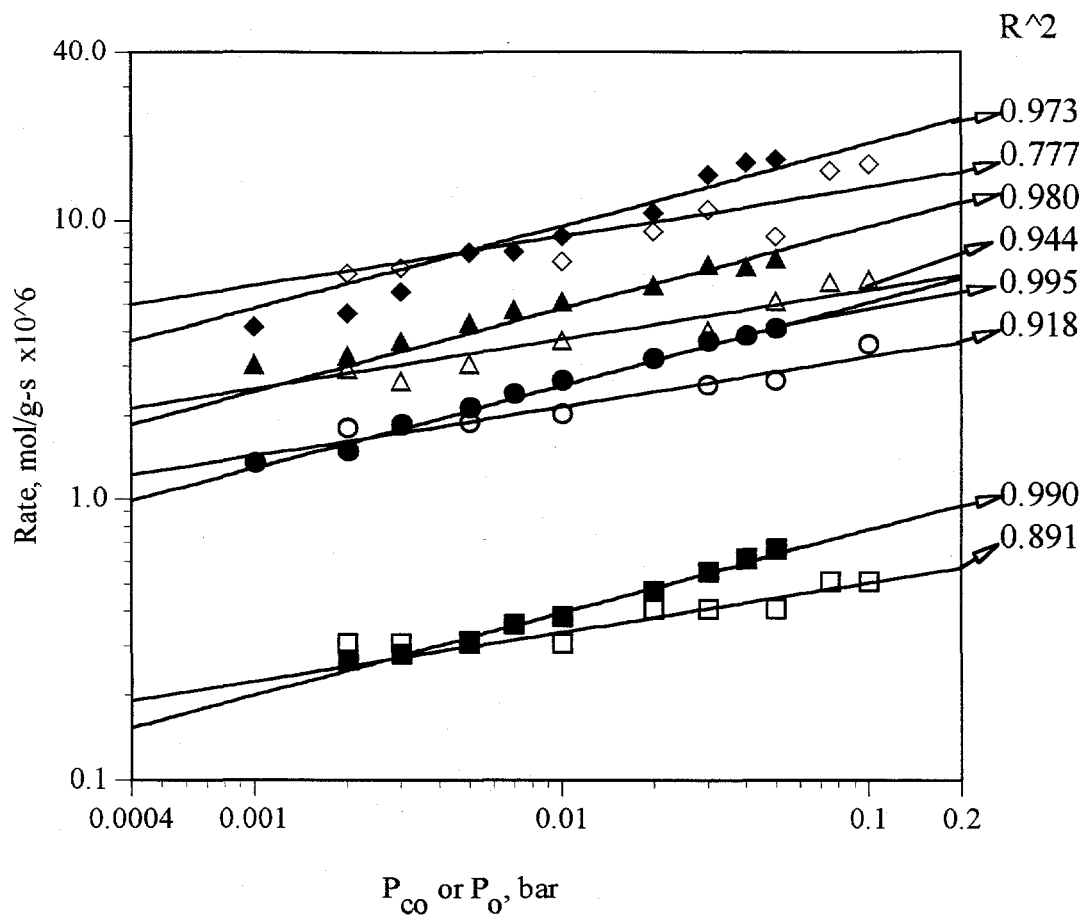
Figure 6.6 Variation of CO Oxidation Rate over the Au_{0.05}[Ce(La)]_{0.95}O_x Catalyst with Partial Pressure of Oxygen and CO. Filled symbols for P_{CO} under P_O=0.05 and the open ones for P_O under P_{CO}=0.01 . ■ 10°C ● 25°C ▲ 43°C ◆ 54°C.
