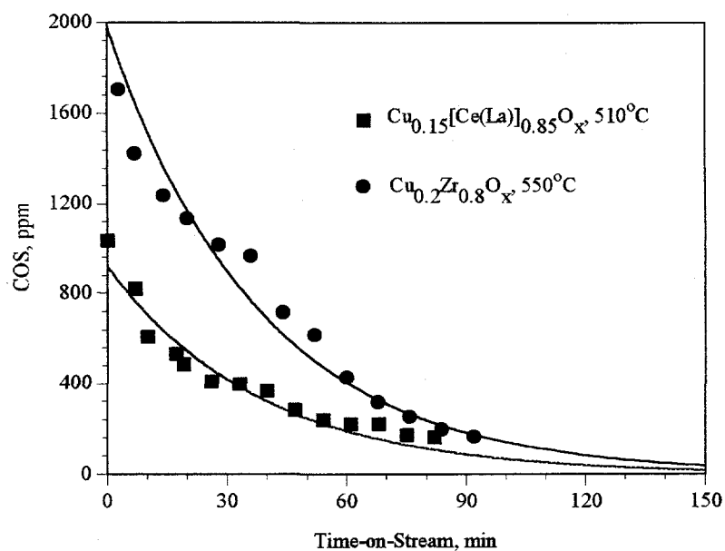
Figure 4.20 \text{COS} Evolution Profile During 2% \text{CO}/\text{He} Scavenging of Spent Catalysts.
