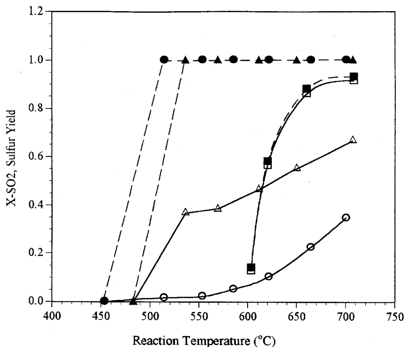
Figure 3.1 Elemental Sulfur Yield and \text{SO}_2 Conversion on Bulk \text{CeO}_2 Catalyst ( R_{\text{CO}} = [\text{CO}]/[\text{SO}_2] ; 1% \text{SO}_2 , 0.017 s·g/cc(STP)). R_{\text{CO}} = 4 : \circ \bullet ; R_{\text{CO}} = 3 : \blacktriangle \triangle ; R_{\text{CO}} = 1.9 : \blacksquare (filled symbols for \text{SO}_2 conversion, unfilled ones for sulfur yield).
