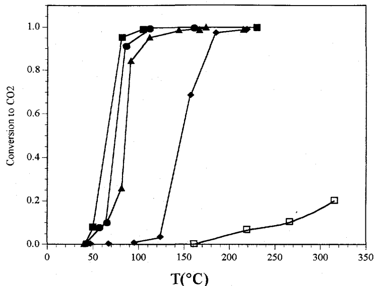
Figure 5.7 Activity Enhancement for CO Oxidation from Combination of CeO 2 and CuO (100 sccm: 2 % CO, 16 % O 2 ). ■ Cu 0.15 [Ce(La)] 0.85 O x , 30 m 2 /g, ● 15 at % CuO x /CeO 2 , 22.4 m 2 /g, ▲ 15 at.% CuO+CeO 2 prepared by 1 h heating in air at 300°C, 18.6 m 2 /g, ◆ bulk CuO, 1.64 m 2 /g, □ CeO 2 , 28m 2 /g.
