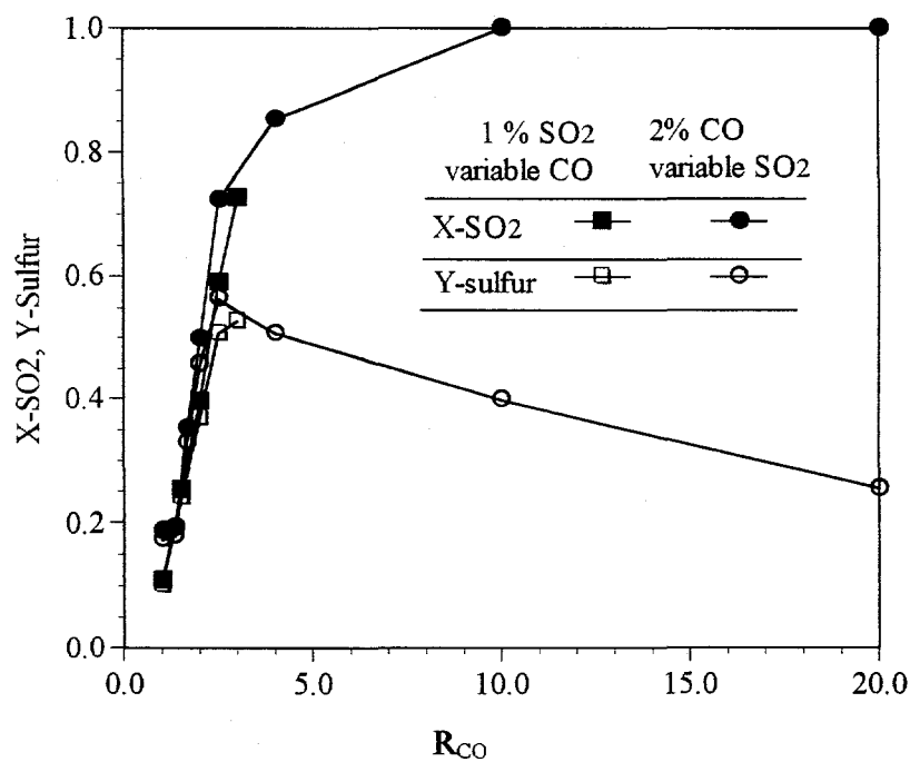
Figure 4.8 Product distribution over Cu 0.15 [Ce(La)] 0.85 O x catalyst versus R CO (0.0113 s.g/cc, 470°C).
