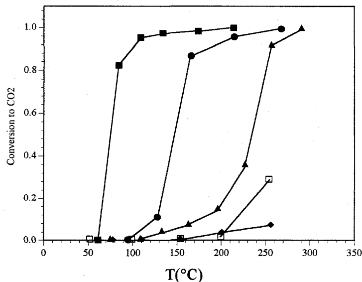
Figure 5.8 Effect of Copper Dispersion on CO Oxidation Activity (100 sccm: 2% CO, 16% O 2 ). ■ Cu 0.15 [Ce(La)] 0.85 O x , 50 mg, 30 m 2 /g ● CuO, 1000 mg, 1.64 m 2 /g ▲ 14 at.% CuO/γ-alumina, 150 mg, 137 m 2 /g ◆ 3.2 at.% Cu-ZSM-5, 150 mg, 400 m 2 /g □ 3.1 at.% Ce, 1 at.% Cu, Ce-Cu-ZSM-5, 150mg, 400 m 2 /g.
