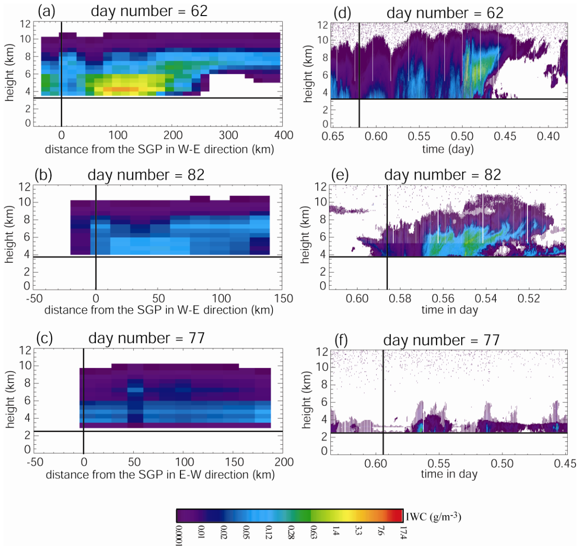
Figure 2. Vertical IWC structures retrieved from (a-c) AMSU-B TBs along the West-East cross section located in Figure 1 and (d-f) MMCR along the time cross section on each day number. The vertical solid lines in (a-c) and (d-f) represent, respectively, the SGP site in space and the AMSU-B satellite observation time at the SGP site.
