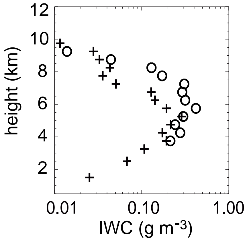
Figure 3. Mean MMCR- (crosses) and AMSU-B-based (circles) IWC profiles. The MMCR time window and AMSU-B search range are 90-minutes and 0.25°, respectively.
