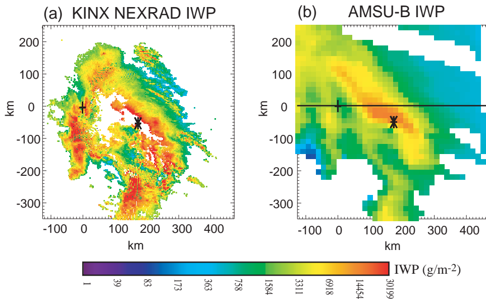
Figure 1. Horizontal IWP distribution from (a) the NEXRAD and (b) the AMSU-B retrievals on 2 March 2000. Cross and asterisk in each panel represent the SGP site and KINX site, respectively. In the NEXRAD IWP, white pixels within echoes denote radar reflectivity greater than 30 dBZ within their cloud column.
