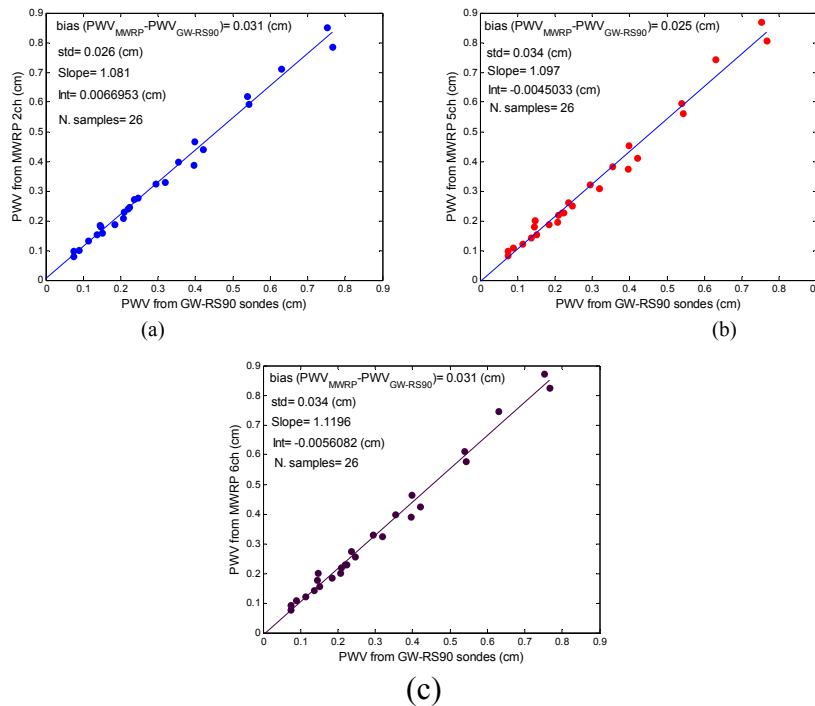
Figure 26. PWV from the MWRP compared with PWV from the GW-RS90 sondes: (a) comparison for the MWRP 2-channel retrieval, (b) for the 5-channel retrieval, (c) for the 6-channel retrieval.
