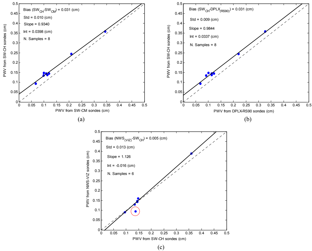
Figure 12. Comparison of PWV from the SW-CH: (a) with the PWV from the SW-CM, (b) with the PWV from the DPLX-RS90, (c) with PWV from the NWS-VIZ radiosonde.
