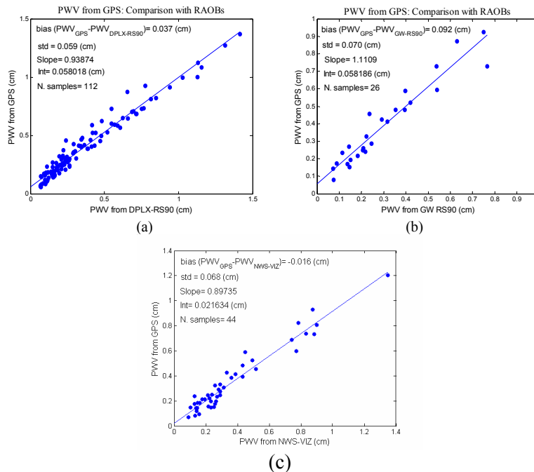
Figure 19. PWV from the radiosondes compared with GPS: (a) PWV from GPS compared with the DPLX-RS90, (b) PWV from GPS compared with the GW-RS90, (c) PWV from GPS compared with the NWS-VIZ radiosondes.
