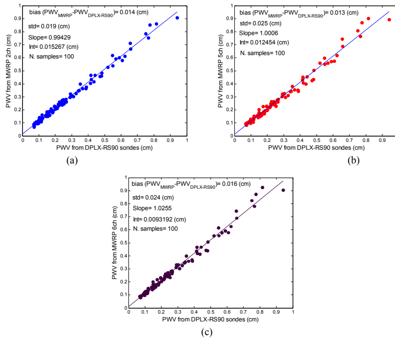
Figure 25. PWV from the MWRP compared with PWV from the DPLX-RS90 sondes: (a) comparison for the MWRP 2-channel retrieval, (b) for the 5-channel retrieval, (c) for the 6-channel retrieval.
