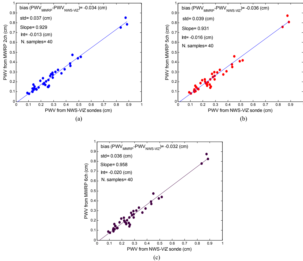
Figure 27. PWV from the MWRP compared with PWV from the NWS-VIZ sondes: (a) comparison for the MWRP 2-channel retrieval, (b) for the 5-channel retrieval, (c) for the 6-channel retrieval.
