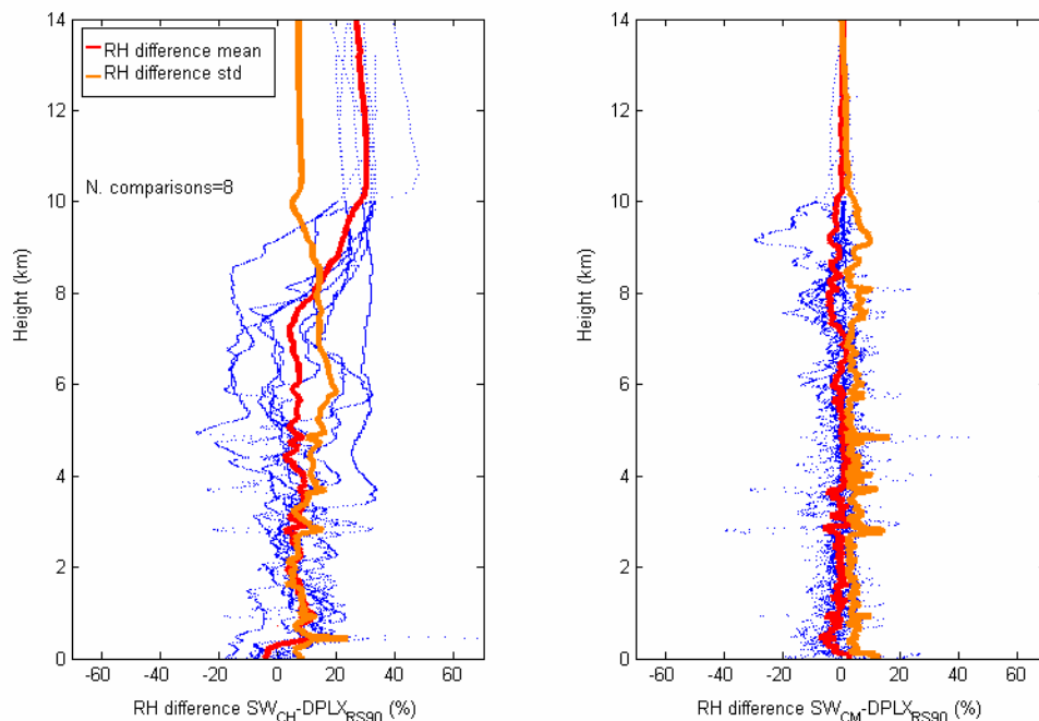
Figure 8. RH difference profiles between the NASA sensors SW-CH (left), SW-CM (right), and the Vaisala RS90 H-Humicap operated at the Duplex.
