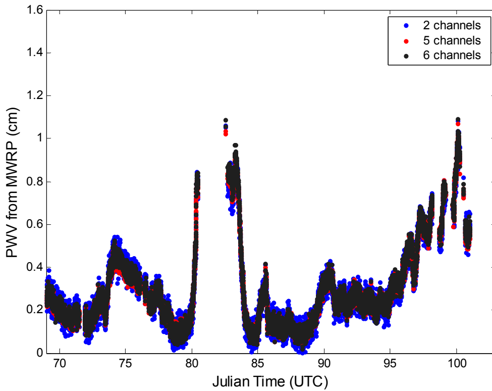
Figure 22. PWV time series from the MWRP, by using two-channel retrieval (blue dots), five-channel retrieval (red dots), and 6-channel retrieval (black dots).
