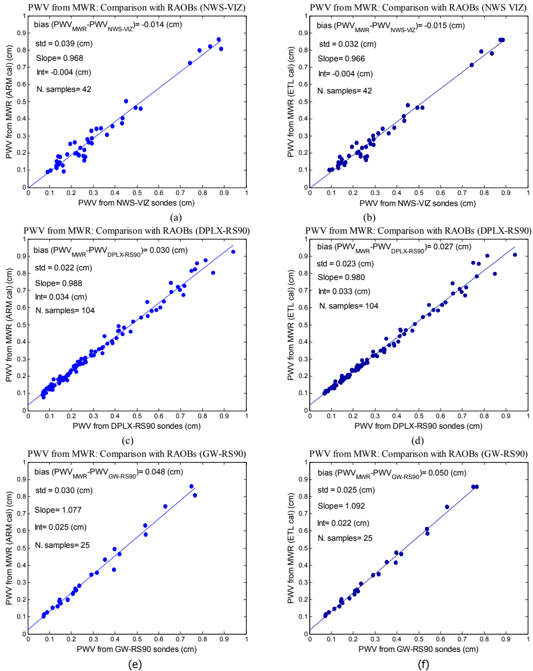
Figure 20. PWV from MWR compared with PWV from the radiosondes: (a) MWR (ARM calibration applied) compared with the NWS-VIZ radiosondes, (b) MWR (ETL calibration applied) compared with the NWS-VIZ radiosondes, (c) MWR (ARM calibration applied) compared with the DPLX-RS90, (d) MWR (ETL calibration applied) compared with the DPLX-RS90, (e) MWR (ARM calibration applied) compared with the GW-RS90, (f) MWR (ETL calibration applied) compared with the GW-RS90.
