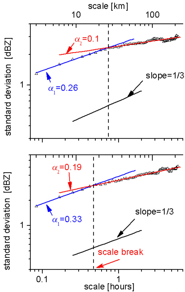
Figure 3a. Scale dependence of ensemble-average standard deviation for boundary layer clouds. The first (second) scaling range is denoted by the blue (red) line. Corresponding power exponents are also shown and summarized in Table 2. The Kolmogorov line (black) is given as a reference.
