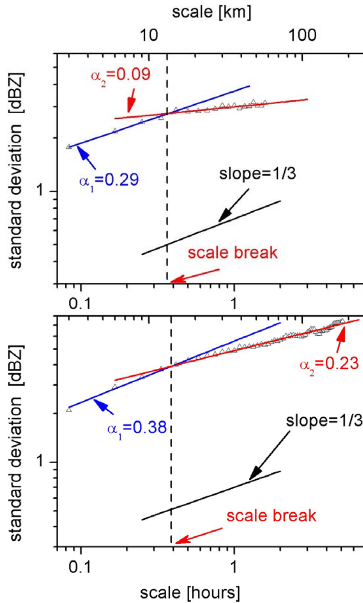
Figure 3b. Scale dependence of ensemble-average standard deviation for low altitude clouds. The notation is the same as on Figure 3a.
