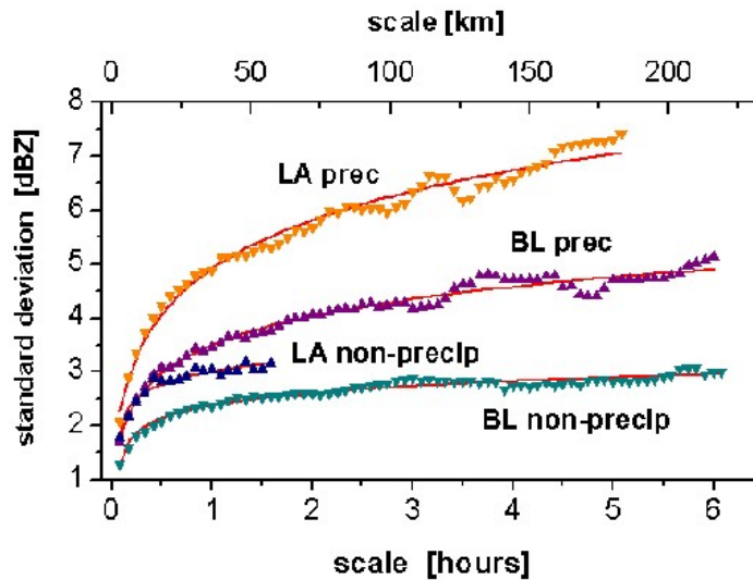
Figure 2. Dependence of variability (defined as an ensemble-averaged standard deviation) on subsample length for boundary layer (BL) and low altitude (LA) clouds, separated into non-precipitating (non-precip) and precipitating (prec) categories. Red lines show best fit curves.
