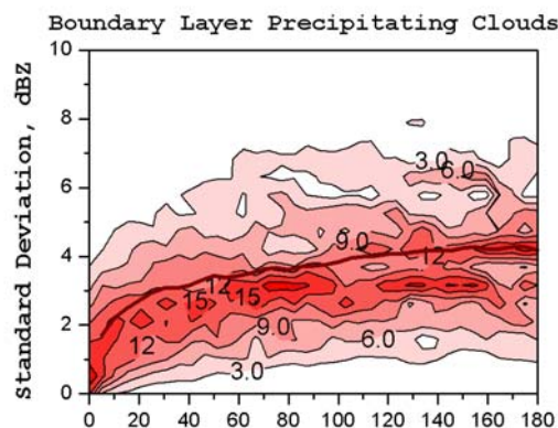
Figure 1. Isolines of reflectivity standard deviation PDFs for precipitating boundary layer clouds. Thick line shows the ensemble-averaged standard deviation.
