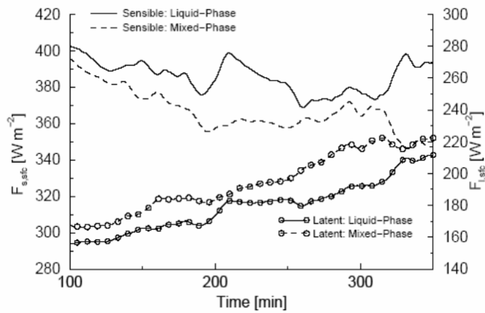
Figure 6. Time-series of sensible and latent heat fluxes.
