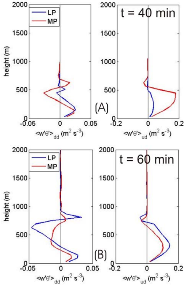
Figure 5. pdraft and downdraft buoyancy fluxes for LP and MP cases at (a) t = 40 minutes and (b) t = 60 minutes.
