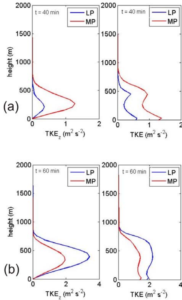
Figure 4. Vertical and Total TKE profiles for LP and MP cases at (a) t = 40 minutes and (b) t = 60 minutes.
