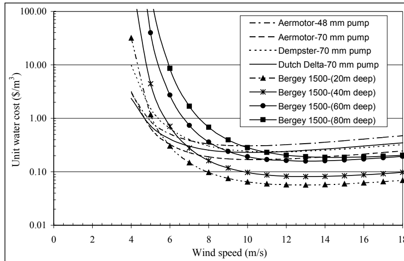
Figure 6-2. Sensitivity analysis of mechanical and electrical wind pumps, based on average flow rate and wind speed data using Weibull distribution coefficient of k = 2 .
