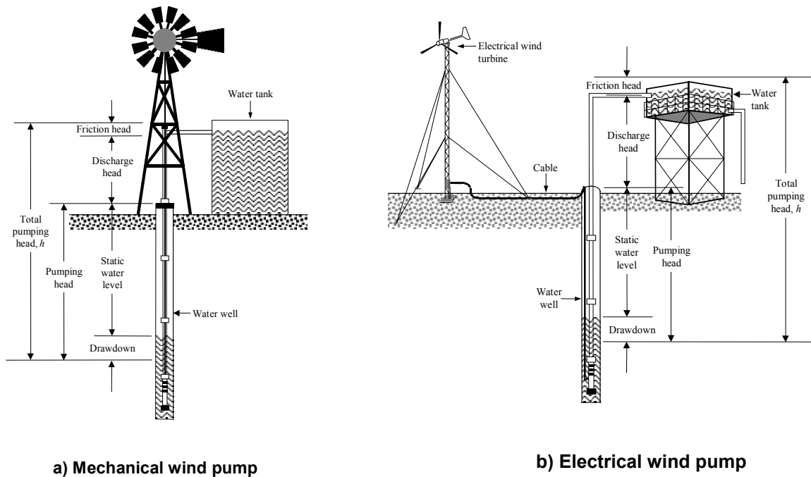
Figure 5-13. Schematic diagram of typical wind pumps.
