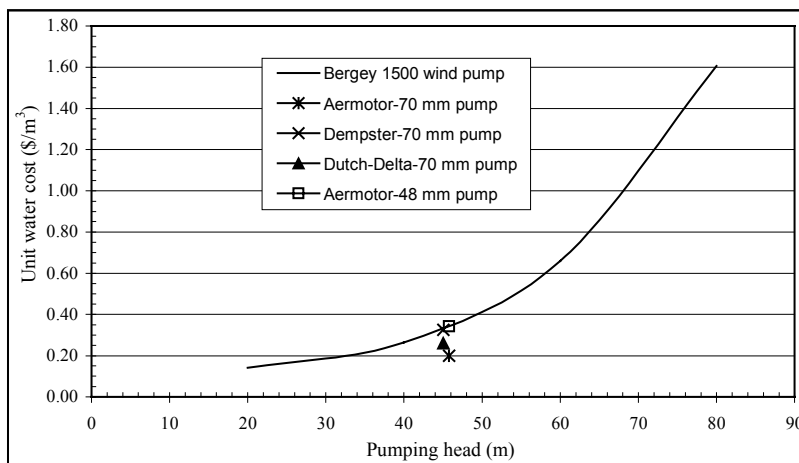
Figure 6-1. Unit water cost versus total pumping head using three types of mechanical pumps and two types of electrical wind pumps at an average wind speed of 5.65 m/s.
