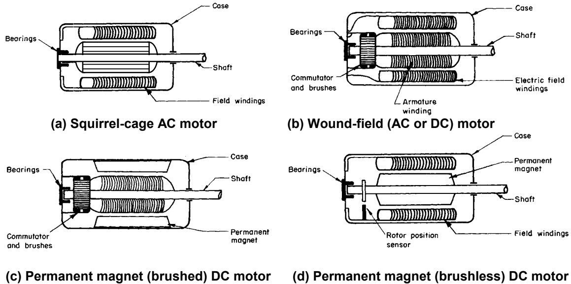
Figure 4-3. Schematic diagrams of the four main types of electric motors.
