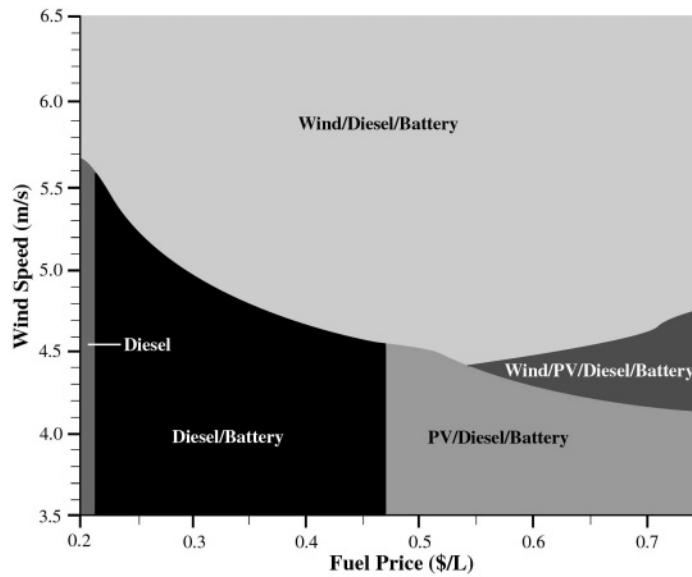
Figure 5-11. Sensitivity analysis of hybrid systems at an average daily load of 20 kWh. The load can be any kind from simple lighting to integrated power supply purpose. This graph is made using a hybrid optimization model for electric renewables (Homer).
