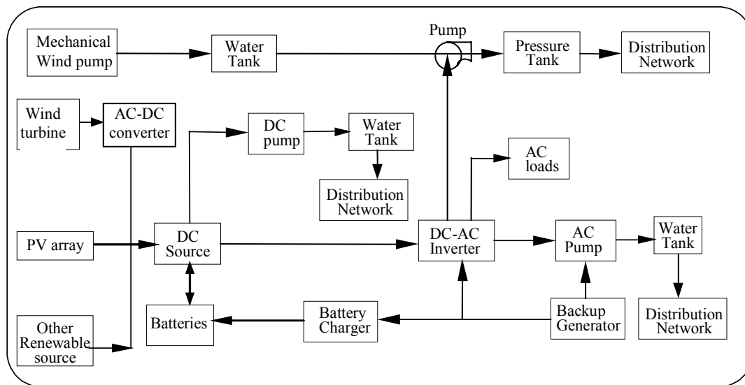
Figure 5-9. Schematic presentation of stand-alone hybrid power sources with a backup generator for water pumping applications.
