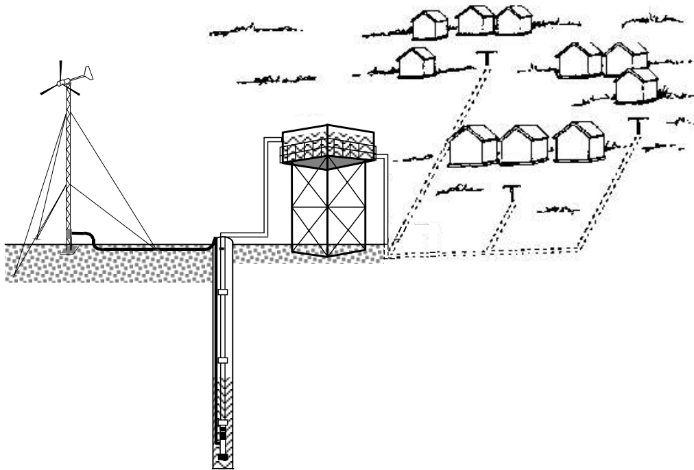
Figure 2-2. Schematic diagram of a village water supply powered by an electrical wind turbine with a typical water distribution network.
