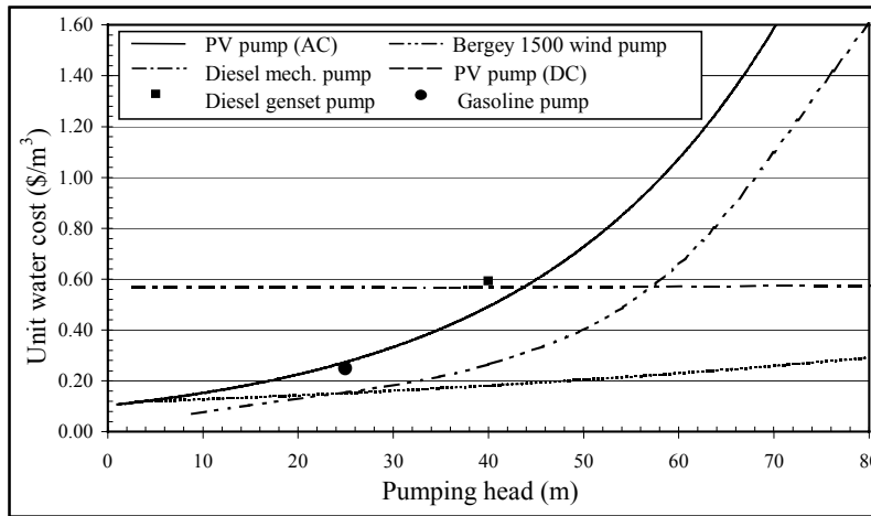
Figure 6-5. Economic comparison of wind, PV, and diesel/gasoline pumping systems.
