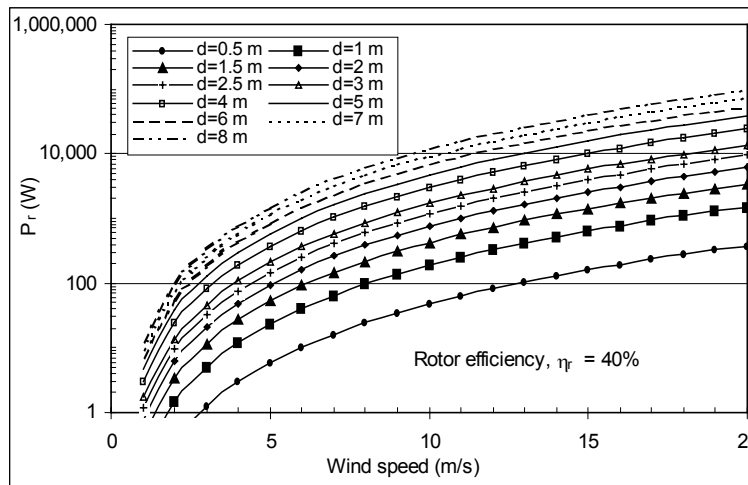
Figure 5-15 Power in the rotor at various wind speeds and rotor diameters, and for rotor efficiency of 40%.
