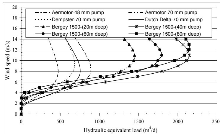
Figure 6-7. Hydraulic equivalent load of electrical and mechanical wind pumps at various average wind speeds using Weibull distribution coefficient of k = 2 .
