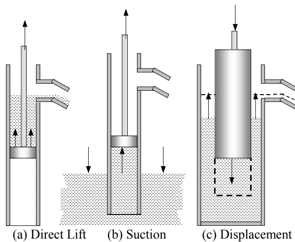
Figure 4-2. Basic operating principles of positive displacement pumps.
