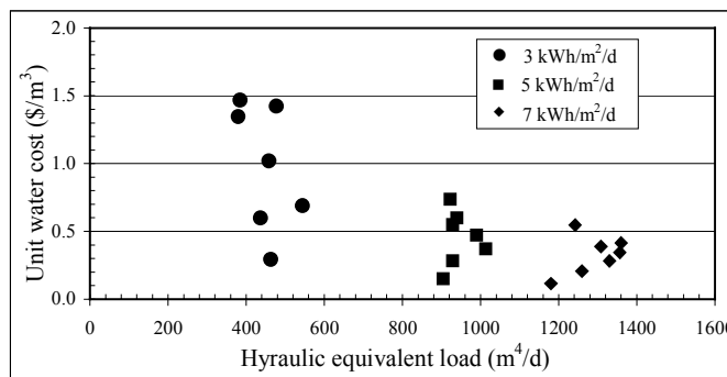
Figure 6-4. Hydraulic equivalent load limits at annual average solar radiation energy levels of 3, 5, and 7 kWh/m 2 /d.
