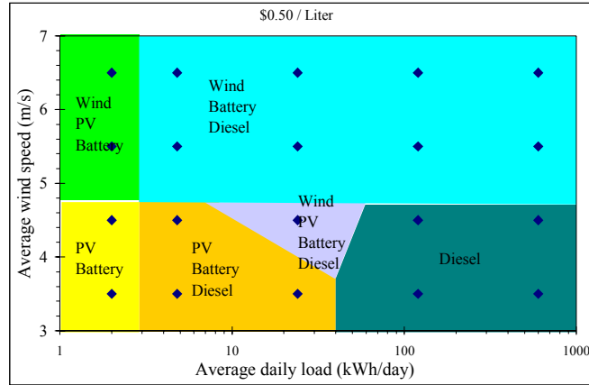
Figure 5-12. Sensitivity analysis of hybrid systems based on a fuel cost of $0.50/L. This graph is made using a hybrid optimization model for electric renewables (Homer).
