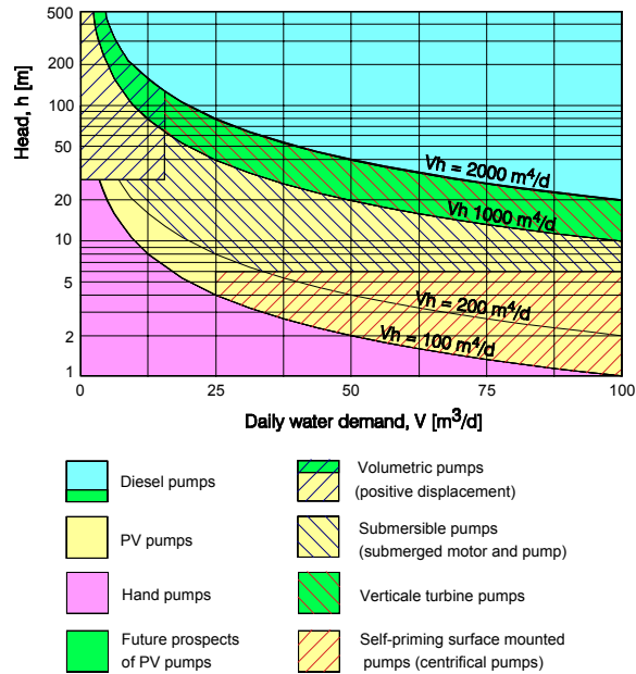
Figure 4-1. Types of pump sets for different ranges of head and flow rates.
