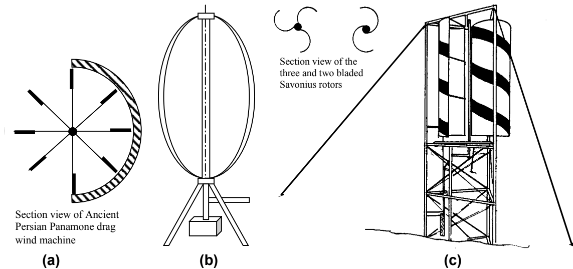
Figure 5-2. Typical vertical axis wind machines: (a) Panemone, (b) Darrieus, and (c) Savonius
