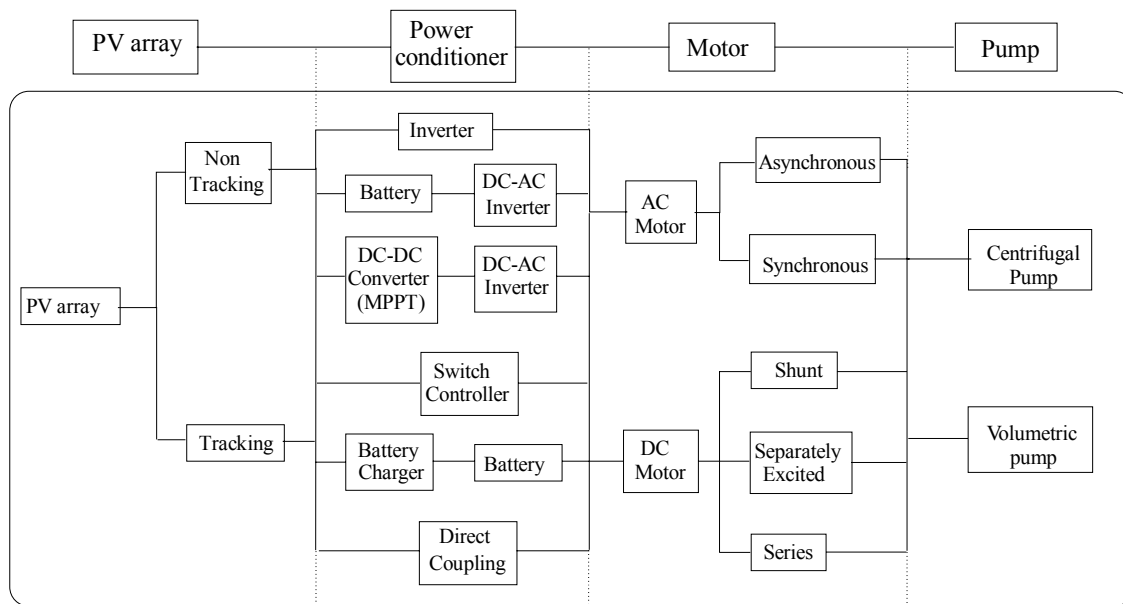
Figure 5-6. The most common components of PV pumping systems.
