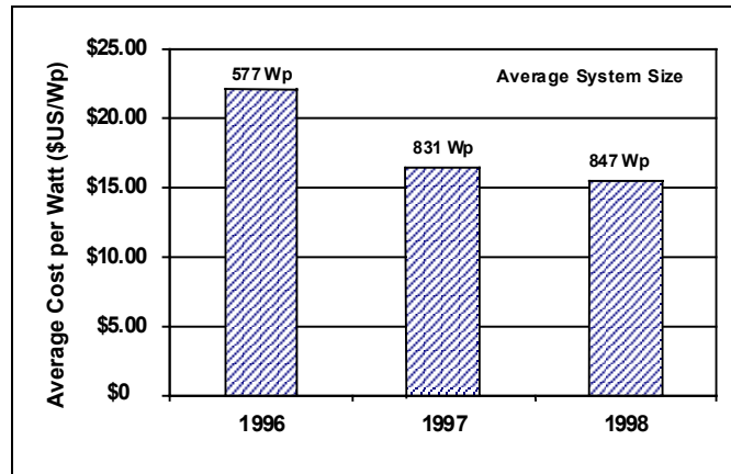
Figure 8-4. Average declining cost trends per installed watt for 41 pilot PV water pumping systems in Mexico implemented by the Chihuahua Renewable Energy Working Group with SNL.
