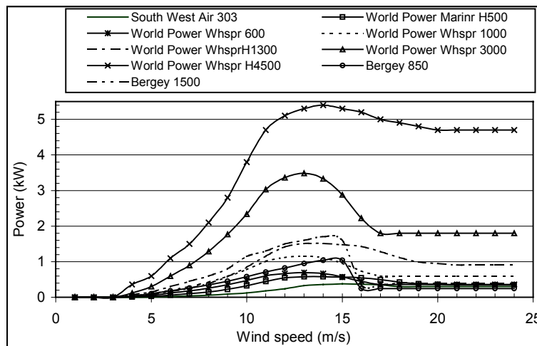
Figure 5-10. Selected wind turbine power curves.
