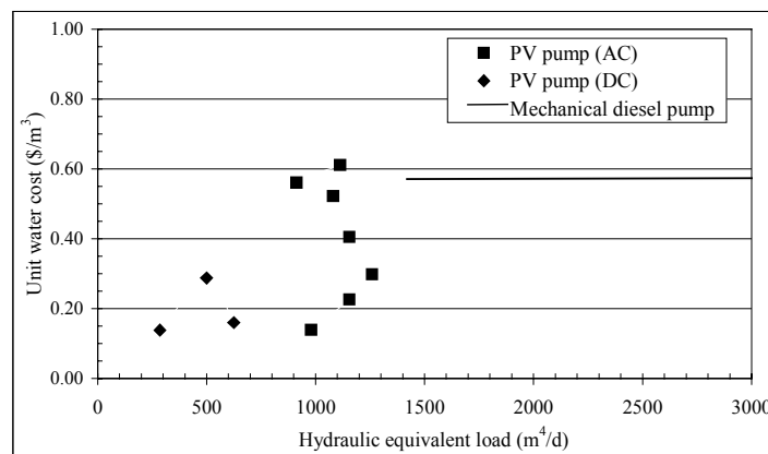
Figure 6-6. Hydraulic equivalent load limits of PV pumps (DC and AC systems) and diesel-driven mechanical pumps (mono).
