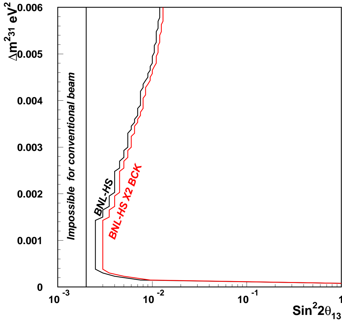
Figure 19: Expected 90% confidence level upper limit on \text{sin}^2 2\theta_{13} versus \Delta m^2_{31} for the BNL-to-Homestake experiment. The two curves are with the background as predicted in Fig. 15 (the left hand curve) and assuming the neutral current background to be a factor of two larger (the curve to the right).
