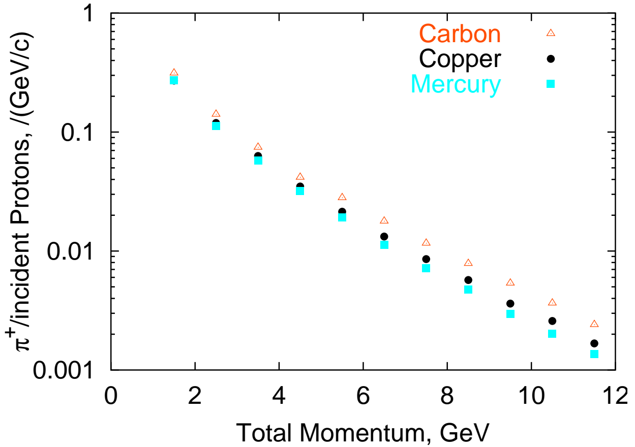
Figure 47: The number of \pi^+ per incident proton is shown as a function of its momentum for carbon, copper and mercury targets. The target is two interaction lengths long for each material.
