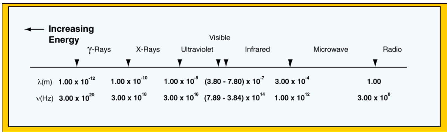
Electromagnetic Spectrum
