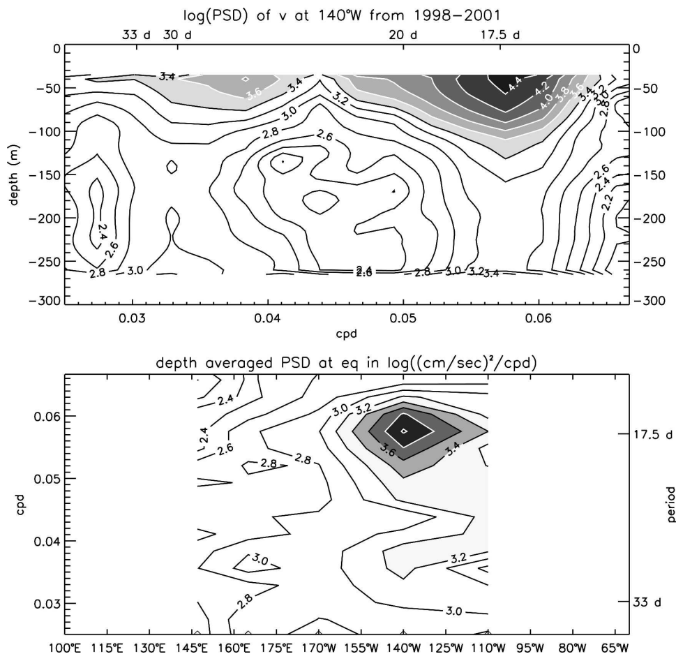
FIG. 4. PSD of filtered meridional velocity from the TAO mooring array at (top) 0^\circ , 140^\circ\text{W} . (bottom) Depth-averaged PSD of filtered velocity at the equator from the TAO mooring array. Diamonds in the bottom panel show mooring locations.
