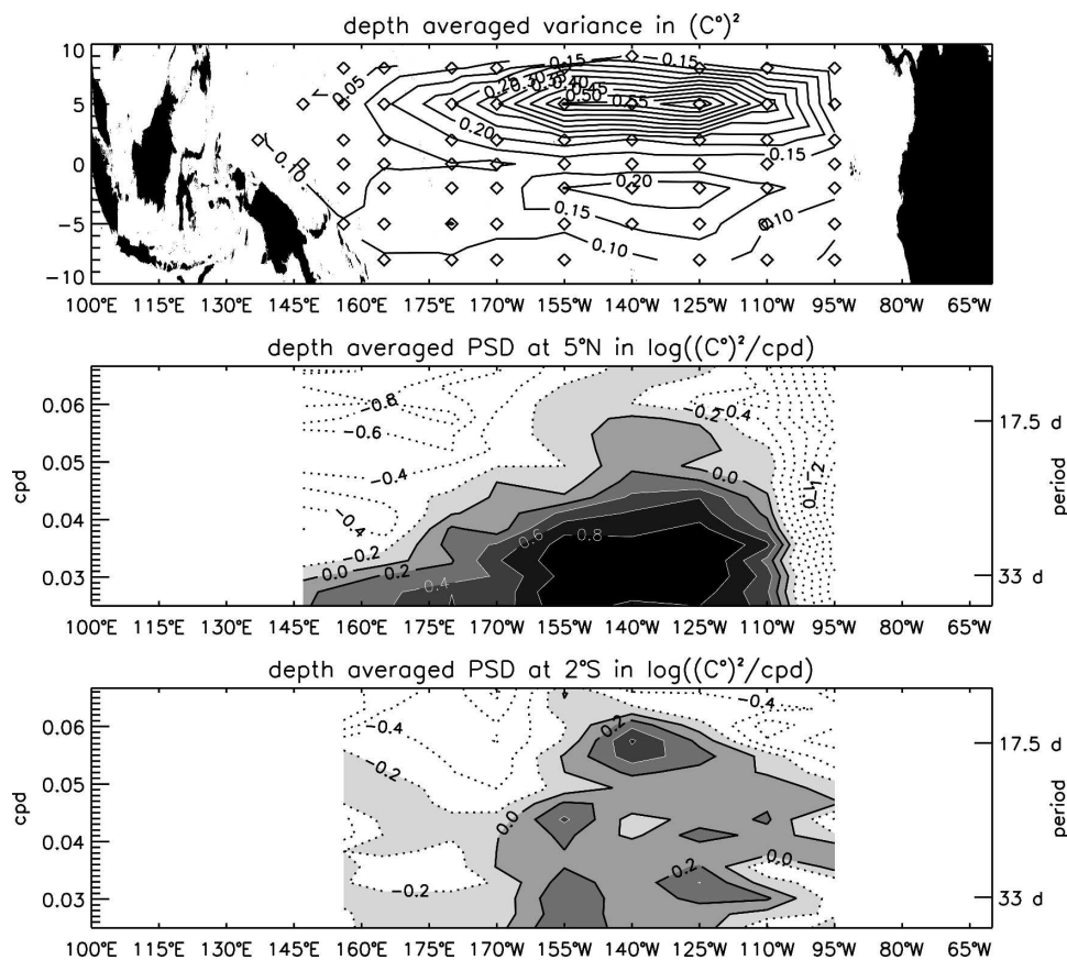
FIG. 2. Depth-averaged (top) variance of filtered temperature from the TAO mooring array and depth-averaged PSD at (middle) 5°N and (bottom) 2°S. Variance and spectra were computed over the same 3-yr period beginning in May 1998. Diamonds in the top panel show mooring locations.
