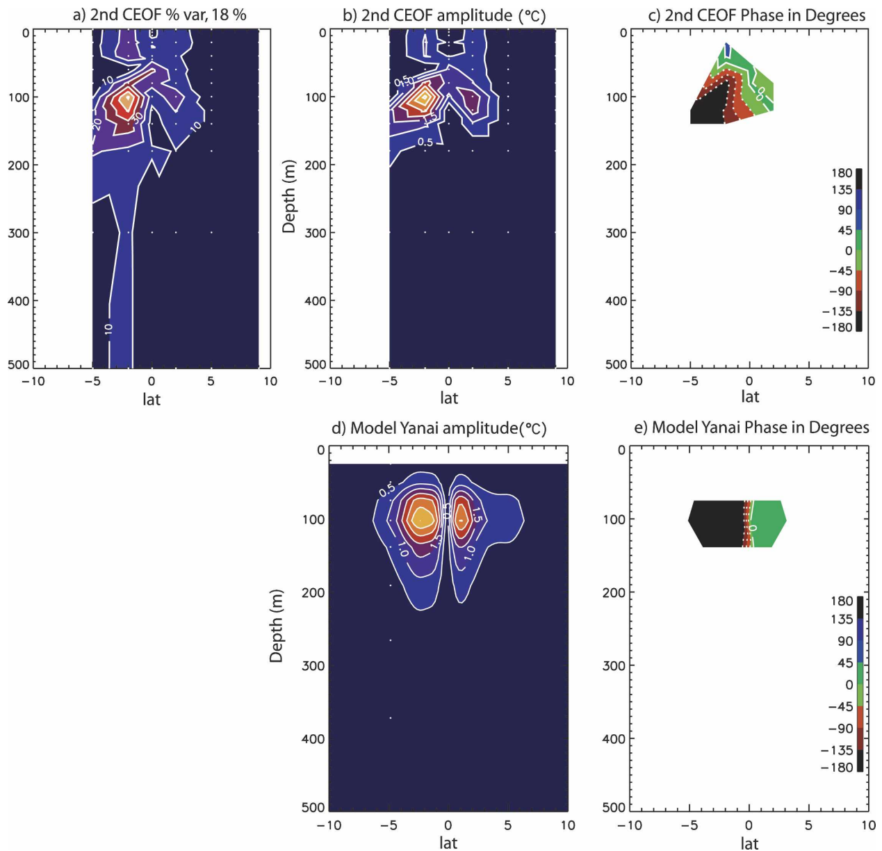
FIG. 14. As in Fig. 9 but for the (a)–(c) second CEOF spatial mode of temperature, and (d), (e) the temperature solution of the n = 1 Yanai wave computed using the Lyman et al. (2005) model with mean zonal currents. Here the model solution is stable and has a 17-day period and a 1320-km zonal wavelength. Model meridional and zonal velocities are shown in Fig. 16. To match the phase in both (c) and (e), the phase in (c) has been shifted by -144^\circ .
