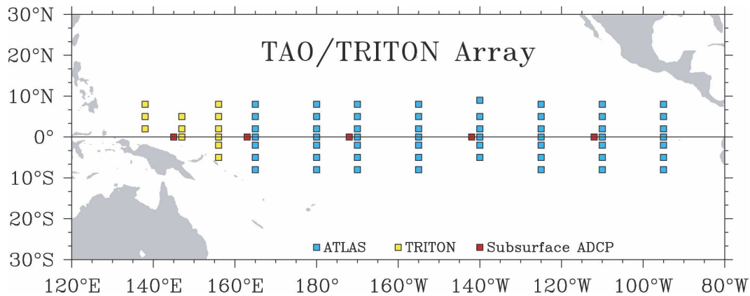
FIG. 1. TAO/TRITON Array mooring locations.
