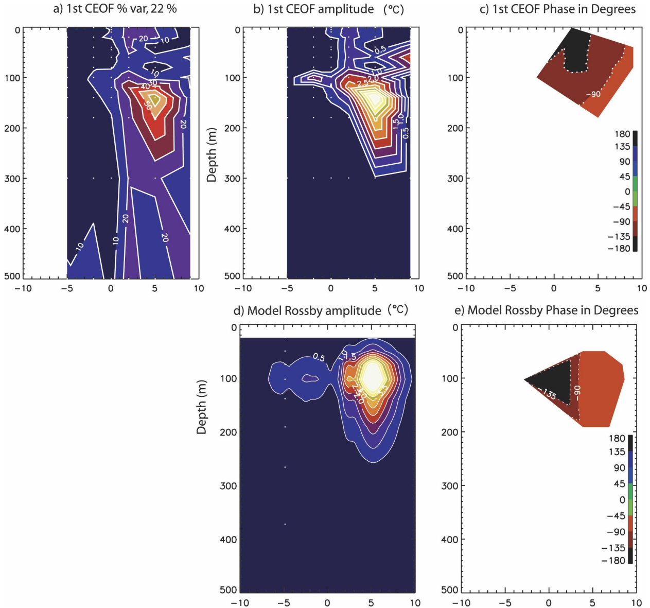
FIG. 9. (a)–(c) Depth–latitude plots for the first CEOF spatial mode of temperature at 140°W and (d), (e) the temperature solution for the n = 1, m = 1 unstable Rossby wave from the Lyman et al. (2005) model. Panel (a) shows percent variance explained; (b) shows the CEOF amplitude multiplied by the maxima of the amplitude time series, contoured where at least 10% of the variance is explained; (c) displays CEOF phase, contoured where the scaled CEOF amplitude exceeds 1°C are shown. The model solution has a 31-day period, a 1384-km wavelength, and a 68-day e -folding time. The amplitude and phase of temperature from the model are also shown in (d) and (e), respectively. Meridional and zonal velocities are not shown. The amplitude of the model has been scaled to match the CEOF amplitude in (b). To match the phase in both (c) and (e), the phase in (c) has been shifted by -85^\circ .
