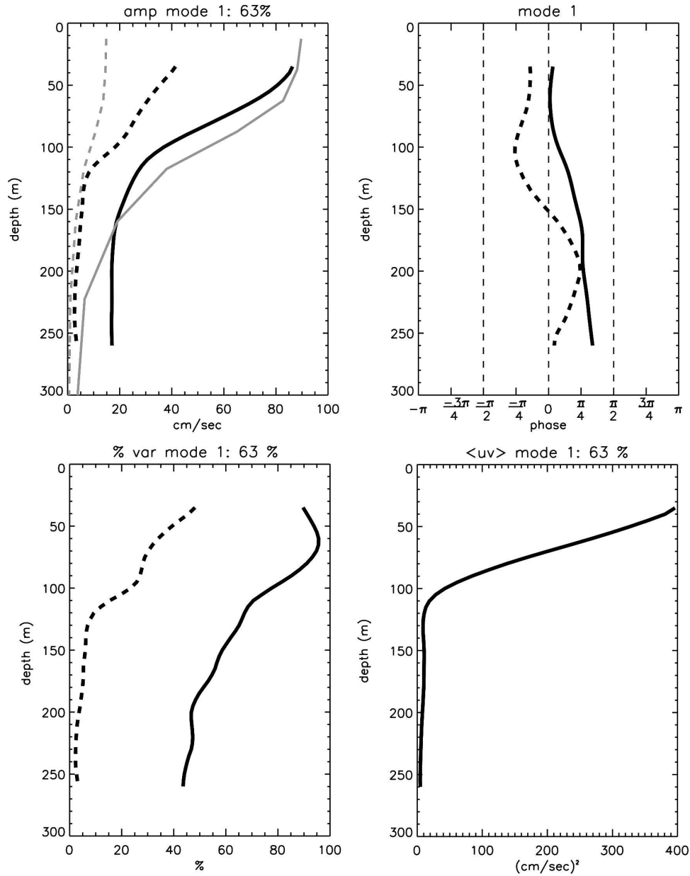
FIG. 13. First velocity CEOF (top left) spatial amplitude, (top right) phase, (bottom left) percent variance explained for meridional (thick solid lines) and zonal (thick dashed lines) velocities, and (bottom right) Reynolds stress. Meridional (thinner gray line in top-left panel) and zonal (thinner gray dashed line in top panel) velocity amplitude of the Yanai wave at the equator from the two-mode projection model scaled to the same order of magnitude as for the CEOF amplitude.
