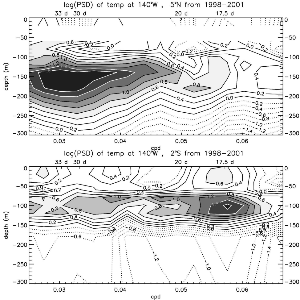
FIG. 3. PSD of filtered temperature vs depth from the TAO mooring array at (top) 5°N, 140°W and (bottom) 2°S, 140°W.
