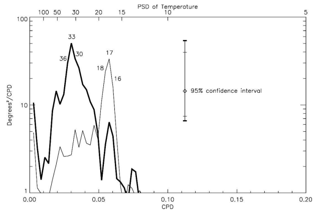
FIG. 8. Power spectral densities of the first (thick line) and second (thin line) temperature CEOFs from Fig. 7, computed according to section 2. Period (days) is plotted on the top x axis and noted on the curve for peaks. The larger error bars are for the first CEOF since the first year of that CEOF has a significant gap.
