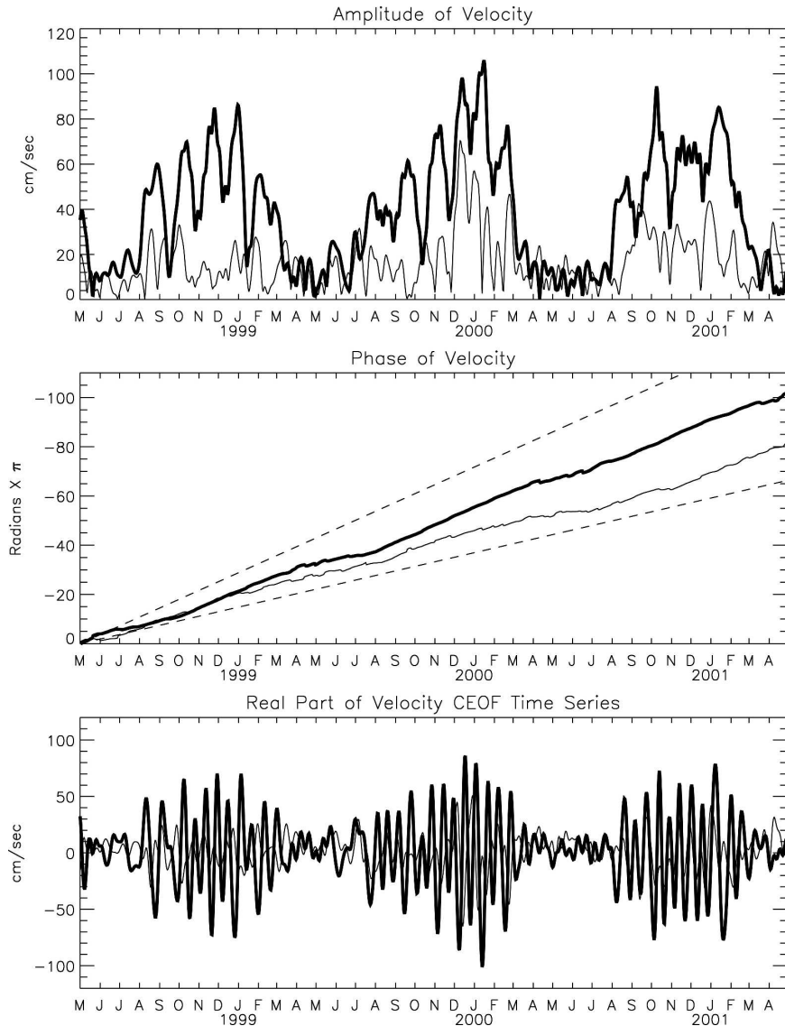
FIG. 11. CEOF analysis following that in Fig. 7 but for the first two combined meridional and zonal velocity CEOFs at 0^{\circ} , 140^{\circ}\text{W} . The first mode explains 63% of the total variance while the second mode explains 17%.
