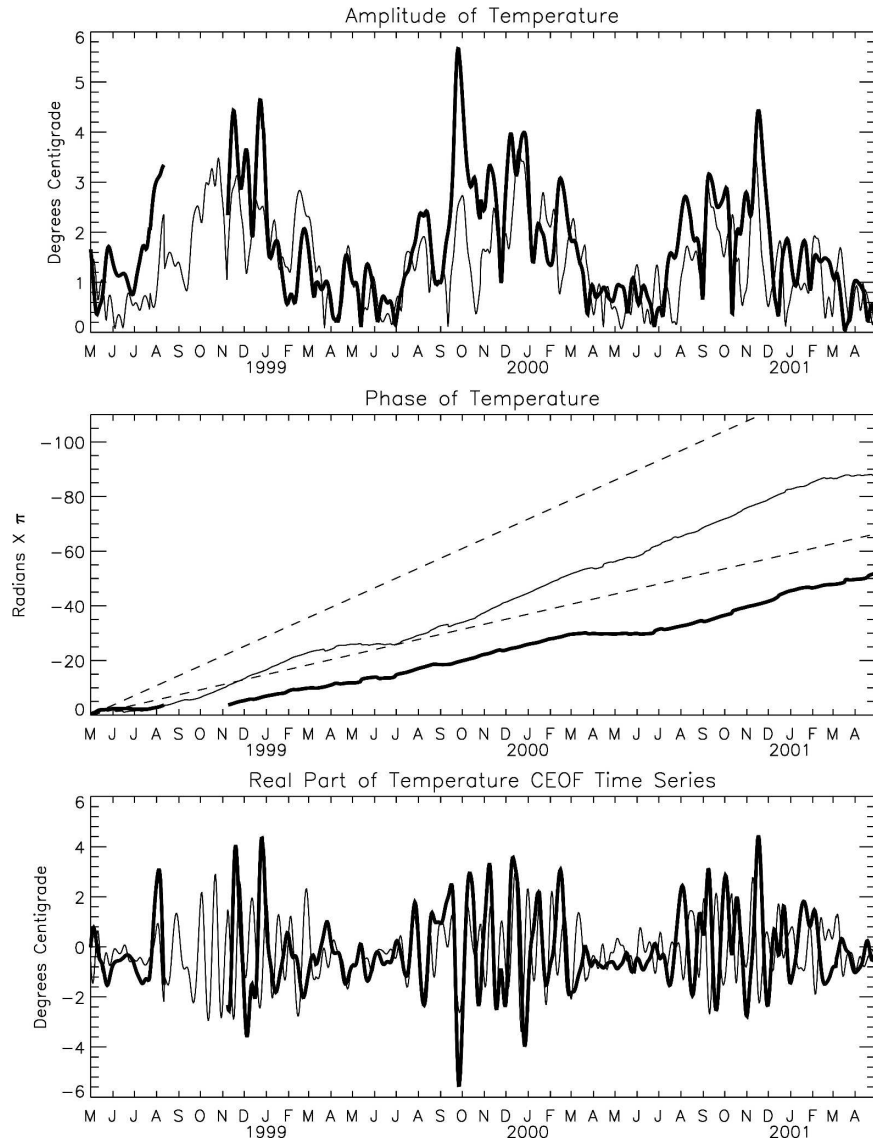
FIG. 7. (top) Amplitude, (middle) phase, and (bottom) real part of the time series for the first two temperature CEOFs along 140°W. The first mode (thick lines) explains 28% of the total variance while the second mode (thin lines) explains 13%. Amplitude and the real part of the time series are multiplied by their maximum spatial amplitudes. Dashed lines in the middle panel correspond to periods of 17 and 33 days. The missing section of the first-mode CEOF was excluded according to criteria described in section 2.
