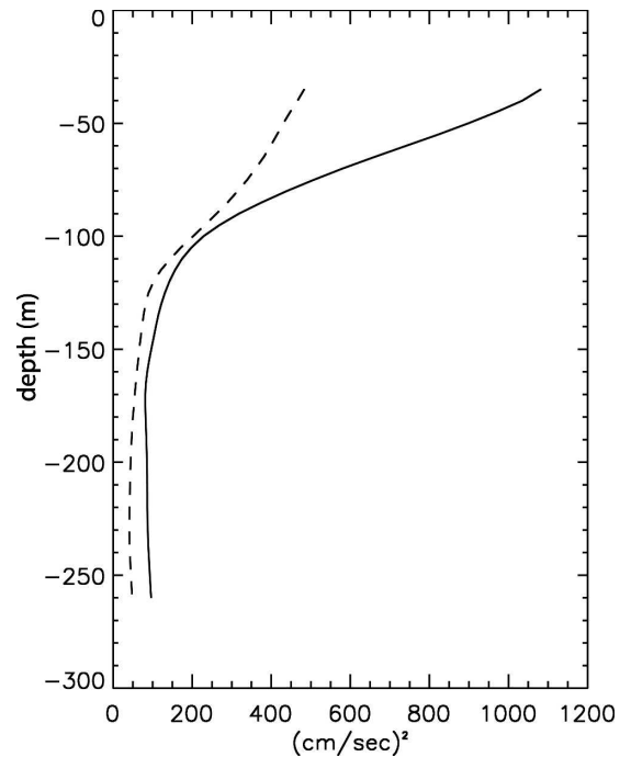
FIG. 10. Variance of bandpass-filtered meridional (solid line) and zonal (dashed line) velocities at 0°, 140°W over the 3-yr record beginning in May 1998.
