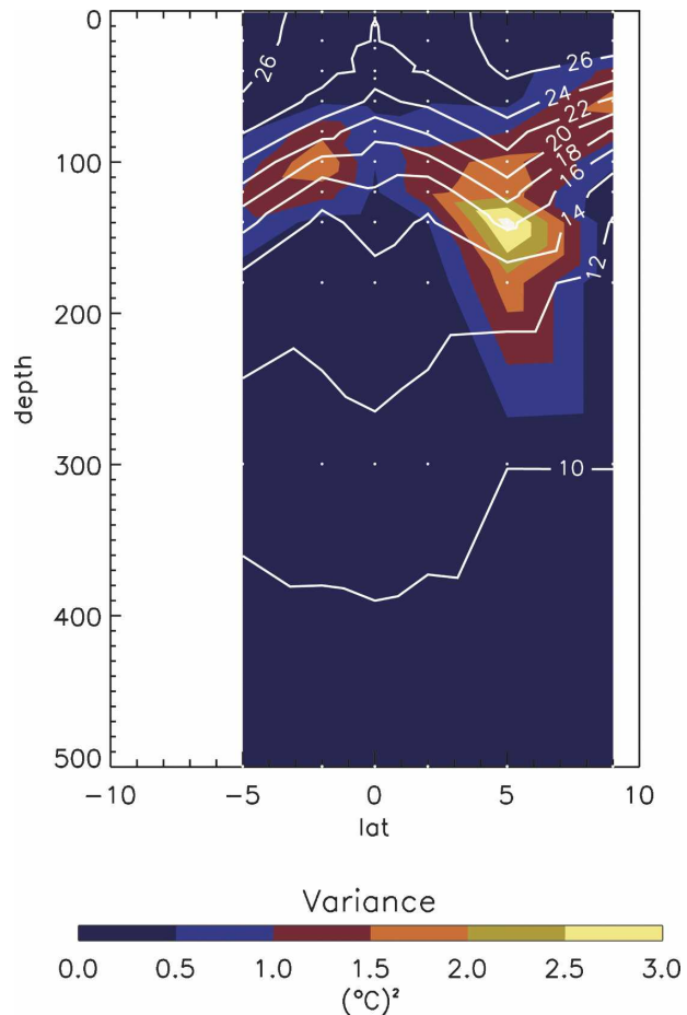
FIG. 6. Variance of bandpass-filtered temperature data at 140^\circ\text{W} over a 3-yr period beginning in May 1998. Mean isotherms (white lines) from the same time period are overlaid. White dots show the TAO thermistor locations.
