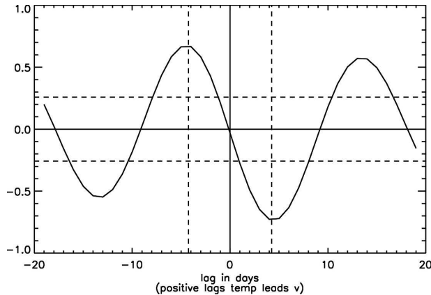
FIG. 15. Lagged cross correlation between real parts of the first CEOF time series for velocity and the second CEOF time series for temperature. For positive lags, temperature leads velocity. Dashed vertical lines show \pm 4.25 days and dashed horizontal lines show 95% confidence level.
