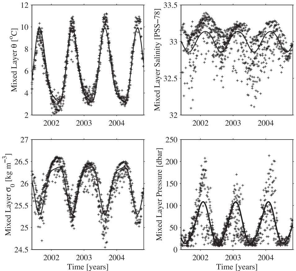
Figure 2. Mixed-layer potential temperature (top left), salinity (top right), potential density anomaly (bottom left), and pressure at the base of the mixed layer (bottom right) plotted versus time using the float CTD data (plusses) in the southeast Aleutian Basin (Fig. 1) with seasonal cycles (solid lines) estimated from annual and semiannual harmonics fit to these data.
