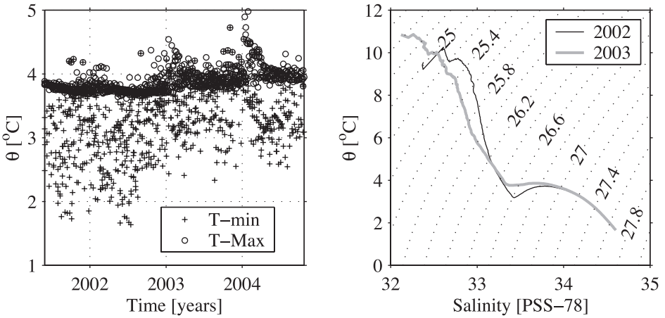
Figure 6. Potential temperature values of the T-min (pluses) from float CTD data in the southeast Aleutian Basin, as well as the T-max (circles) plotted versus time (left). Mean potential temperature-salinity ( \theta -S) relationships for 2002 (thin black line) and 2003 (thick grey line) in the region with potential density anomaly contours (dotted lines) overlaid at 0.2 \text{ kg m}^{-3} intervals (right).
