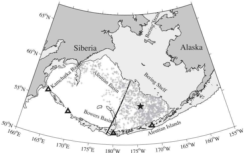
Figure 1. Bering Sea geography. Major connections between the deep basins of the Bering Sea and the North Pacific include (west to east, indicated by triangles) Kamchatka Strait, Near Strait, Amchitka Pass, and Amukta Pass. Float CTD profile locations (grey pluses) are indicated along with the mapping location (pentagram). Areas shallower than 1000 m are lightly shaded, with land more darkly shaded. The thick line separates data in the southeast Aleutian Basin from the rest of the deep Bering Sea.
