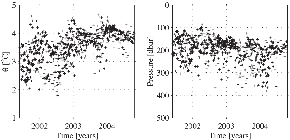
Figure 7. Values of potential temperature (left) and pressure (right) on \sigma_{\theta} = 26.6 \text{ kg m}^{-3} from float CTD data in the southeast Aleutian Basin (Fig. 1).
