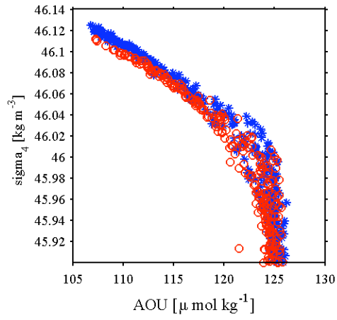
Figure 3. Apparent Oxygen Utilization (AOU) values from bottle data plotted versus \sigma_4 in the Australian-Antarctic Basin in 1994/5 (blue asterisks) and 2007 (red open circles).
