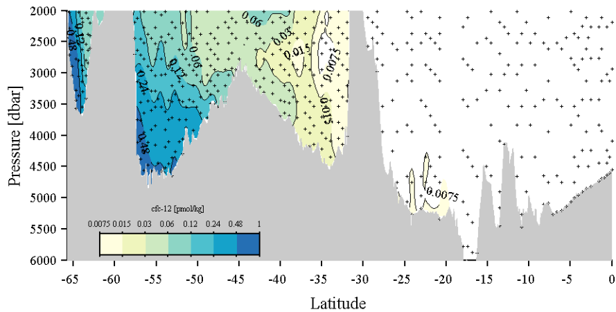
Figure 8. Concentrations of CFC-12 measured along I08S/I09N in 2007 for the portion of the section south of the equator from 2000–6000 dbar contoured at doubling intervals from 0.0075 to 0.48 \text{pmol kg}^{-1} ( 1 \text{ pmol} = 1 \times 10^{-12} \text{ mole} ). Data (plus signs denote locations) were objectively mapped assuming a Gaussian covariance function with correlation length scales of 1^\circ latitude and 500 dbar and a 0.1 noise to signal energy ratio. Color palette from www.colorbrewer.org , by Cynthia A. Brewer, Penn State University.
