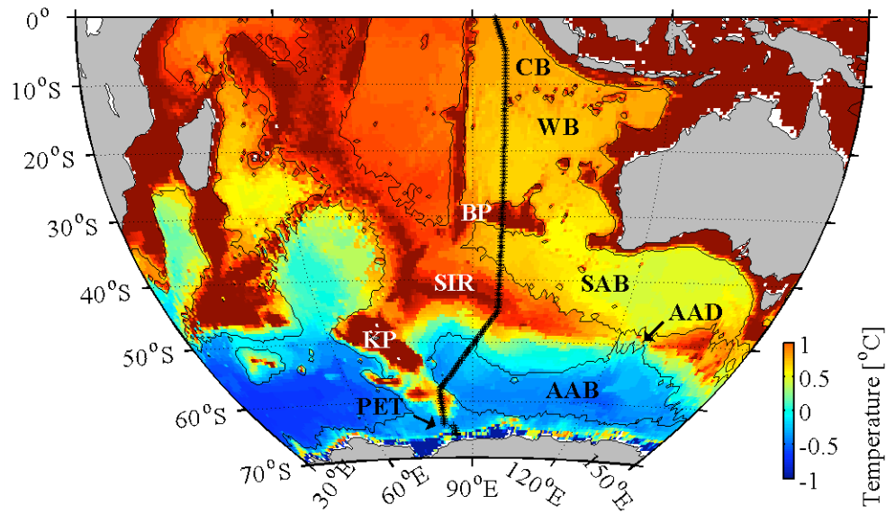
Figure 1. Station locations used from sections with WHP designators SR03, I08S (south of about 30°S), and I09N (north of about 30°S). Stations from the 1994/5 WOCE survey (plusses) and from the 2007 U.S. Repeat Hydrography Program survey (crosses) essentially overlie each other, except for a slight divergence south of 64°S. The 4000-m isobath (thin black line) is plotted over bottom potential temperature (colors) from the WOCE Global Hydrographic Climatology (Gouretski and Koltermann 2004). Land is shaded gray. Place names indicated with abbreviations include the Princess Elizabeth Trough (PET, with arrow), the Australian-Antarctic Basin (AAB), the Australian-Antarctic Discordance (AAD, with arrow), the Kerguelen Plateau (KP, white), the Southeast Indian Ridge (SIR0, white), the Broken Plateau (BP, white), the Wharton Basin (WB), and the Cocos Basin (CB).
