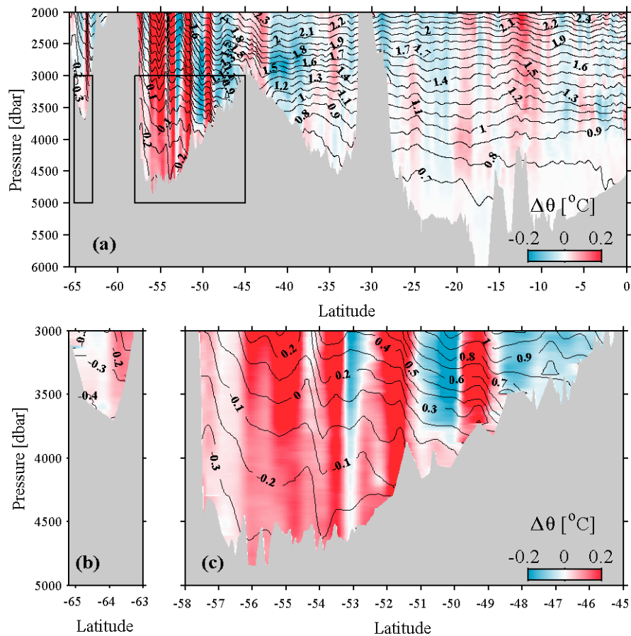
Figure 4. Mean potential temperature \theta [°C] isotherms (black, contoured at 0.1°C intervals) and differences \Delta\theta [°C] (colors) resulting from subtracting the 1994/5 from the 2007 data (gridded on isobars) along I08S/I09N. Red areas indicate warming and blue areas cooling with color saturation at \pm 0.2^\circ\text{C} . Panels show (a) the section south of the equator from 2000–6000 dbar, (b) the Princess Elizabeth Trough from 3000–5000 dbar, and (c) the Australian-Antarctic Basin from 3000–6000 dbar. The bottom bathymetry is shaded gray. The locations of panels (b) and (c) are outlined by black rectangles in panel (a).
