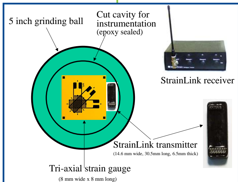
Instrumented Grinding Ball and Its Components
