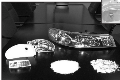
Argonne's froth flotation technology results in a high-quality ABS material that can be used to manufacture products such as the automotive lighting parts shown at right.
