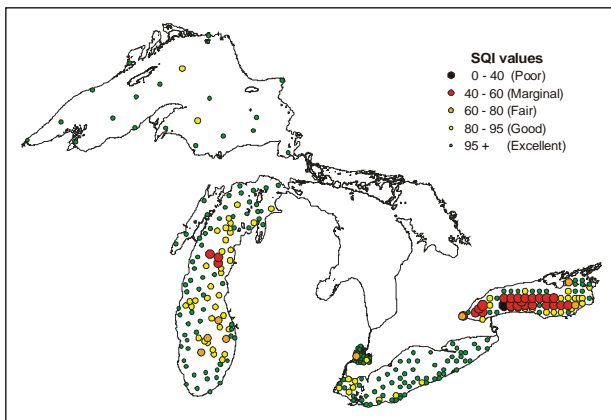
Figure 3. Site Sediment Quality Index (SQI) based on lead, zinc, copper, cadmium and mercury.
