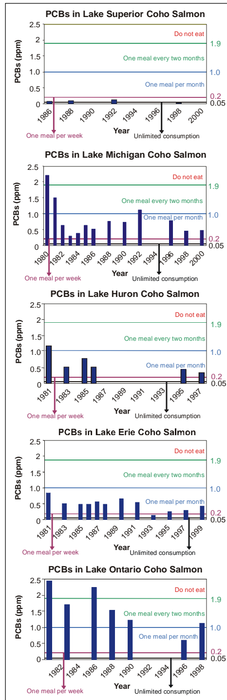
Figure 2. Results of a uniform fish advisory protocol applied to historical data (PCBs, coho salmon) in the Great Lakes. Blank indicates no sampling.
