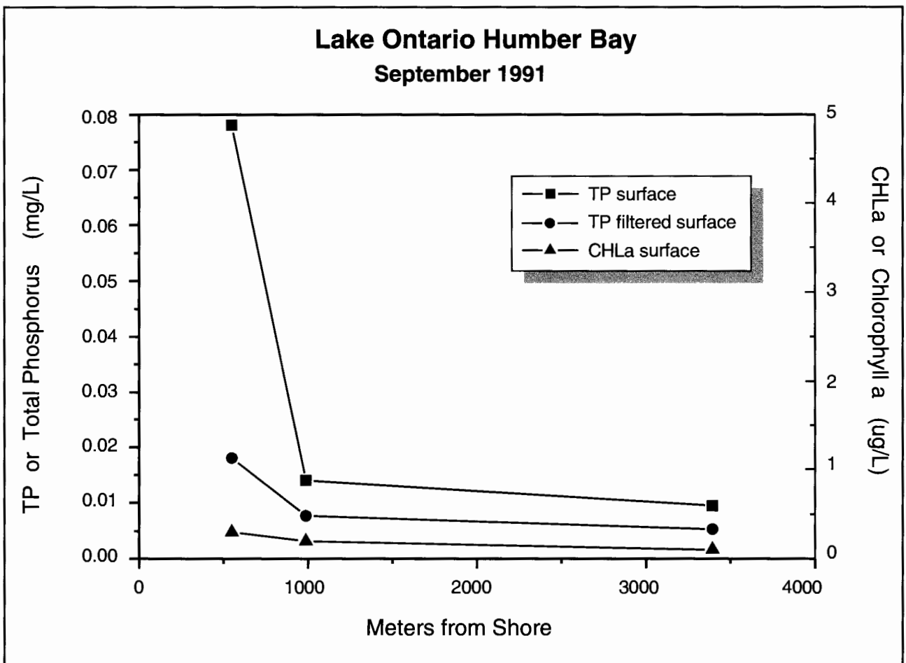
Figure 5. Phosphorus and Chlorophyll a Gradients in Lake Ontario Source: Edsall, T. and M. Charlton. 1997. Nearshore Waters of the Great Lakes . (SOLEC 96 Background Paper)
