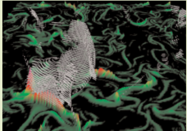
A rendering of the intermittency of a scalar field during turbulent mixing. A 2D surface shows a slice through the mixed volume. Representative 3D structures within the field are shown with gray isolines.
