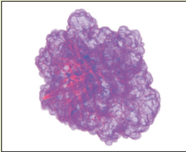
Volume rendering of an unstable flame front from a simulation of the deflagration phase of a Type Ia supernova. The flame was ignited as a spherical region slightly off-center in the white dwarf star and results in a rapidly rising reactive bubble.
