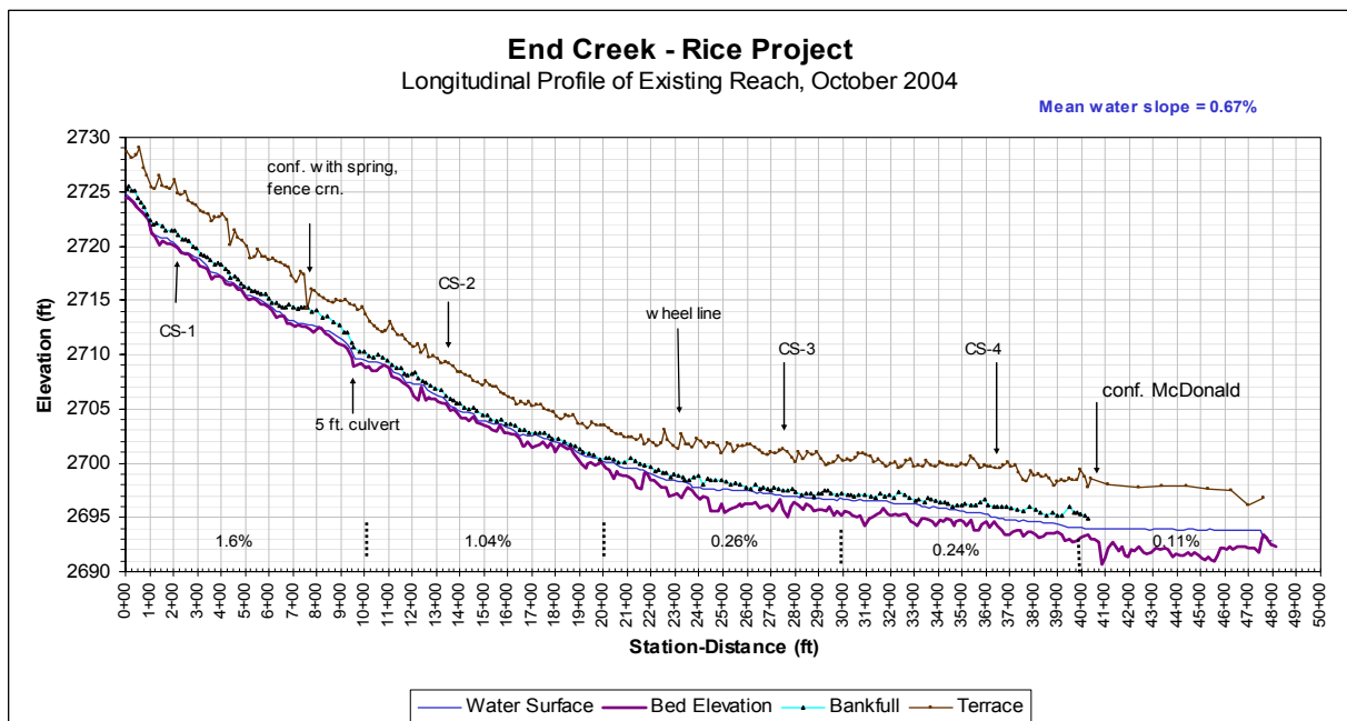
Figure 7 Longitudinal Profile of Lower End Creek
