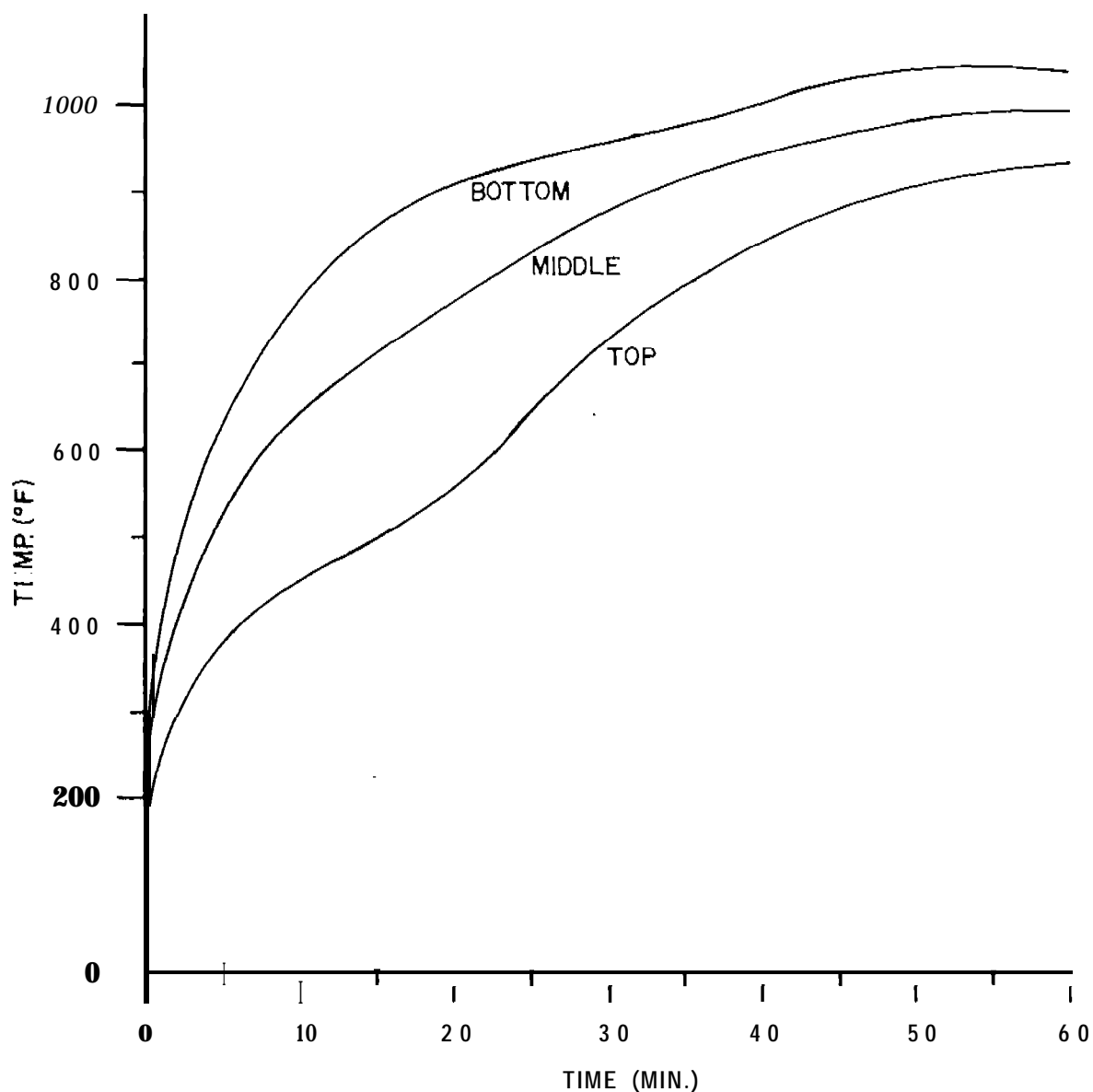
Figure 4. Flammable liquid test fire - average temperatures on surface of concrete block wall.
