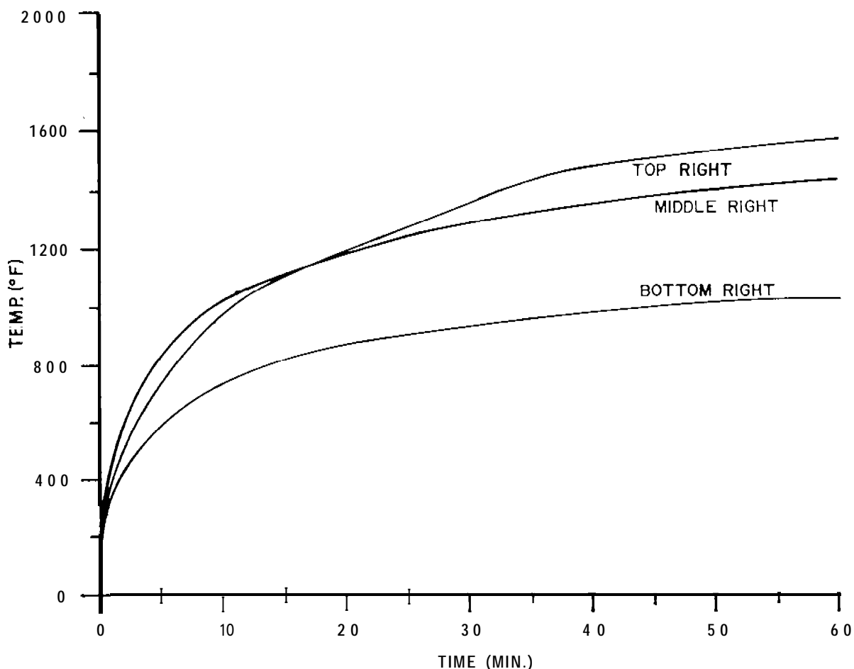
Figure 5. Flammable liquid test fire - temperatures on right side of concrete block wall.
