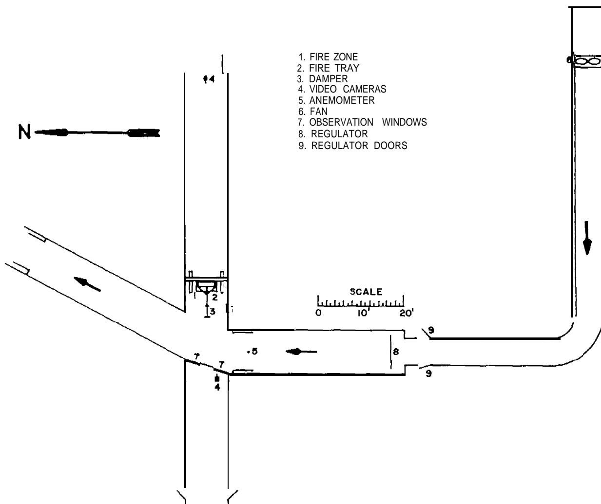
Figure 1. Plan view of fire gallery.
