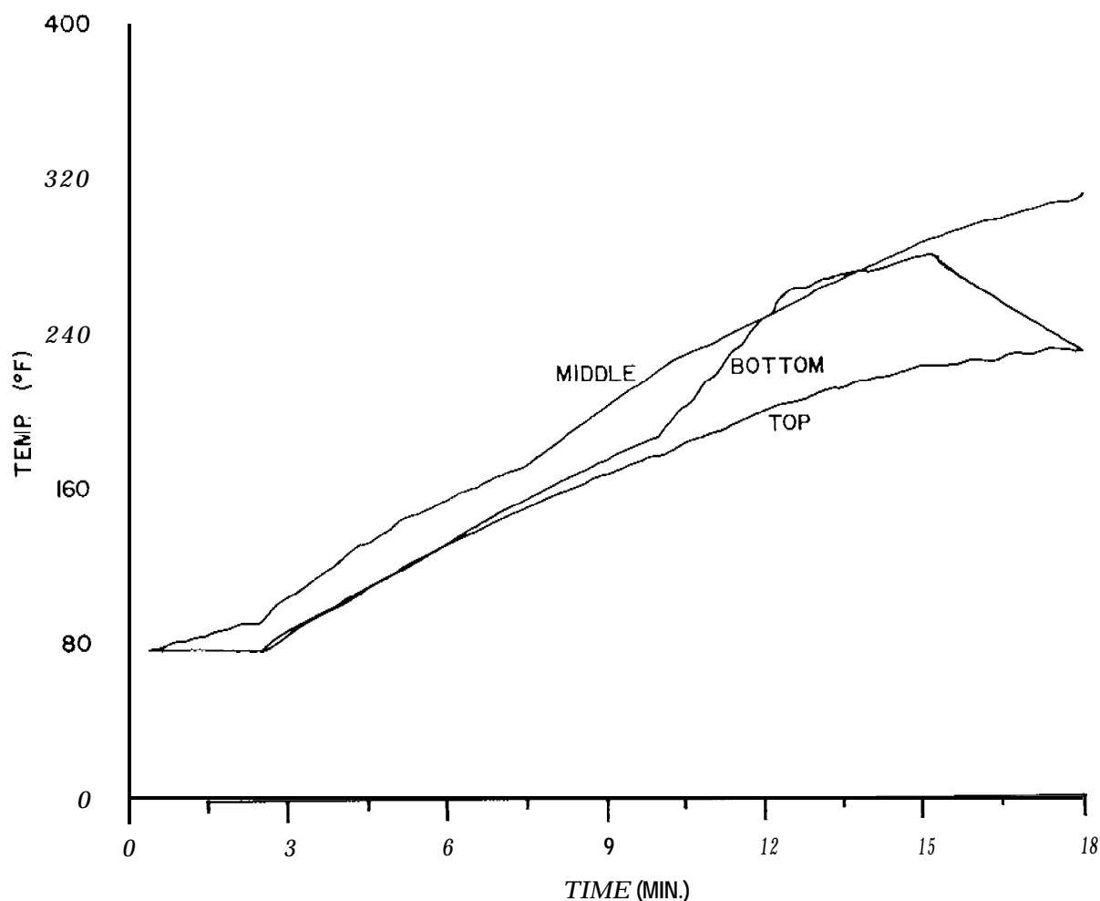
Figure 3. Wood crib test fire - average wall temperatures.
