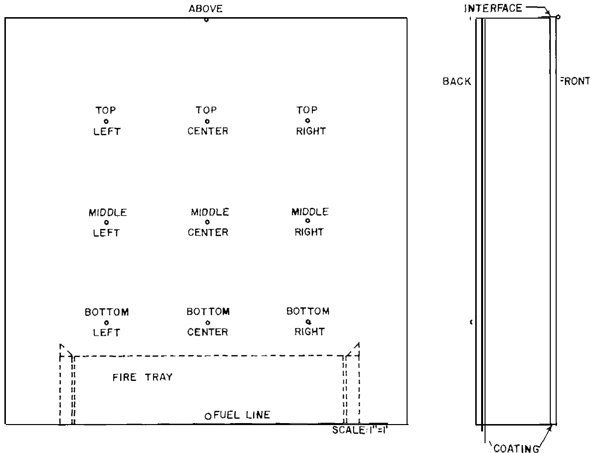
Figure 6. Test wall thermocouple locations.
