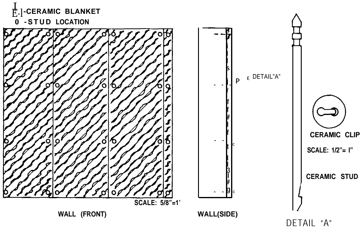
Figure 7. Ceramic blanket fastening system.
