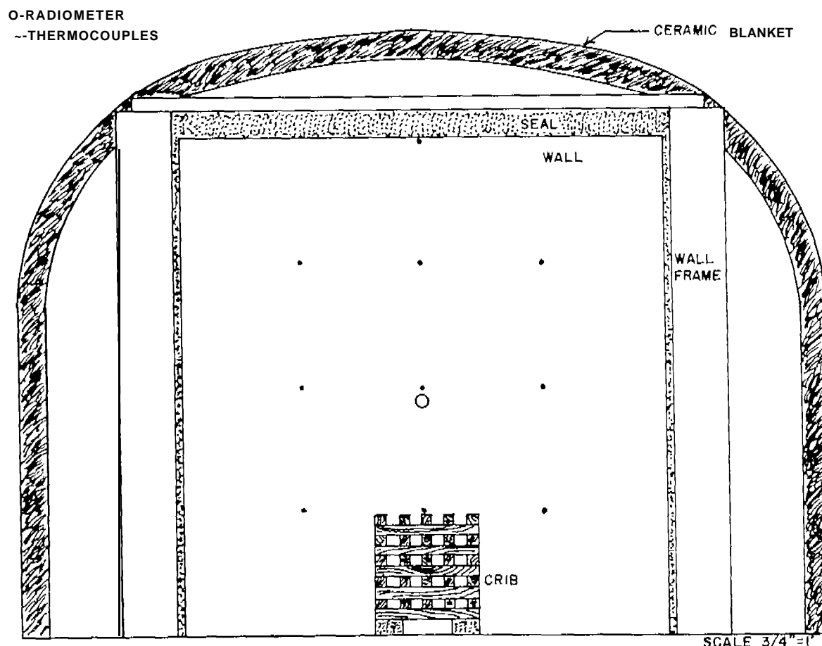
Figure 2. Fire zone instrumented with radiometer and thermocouples.
