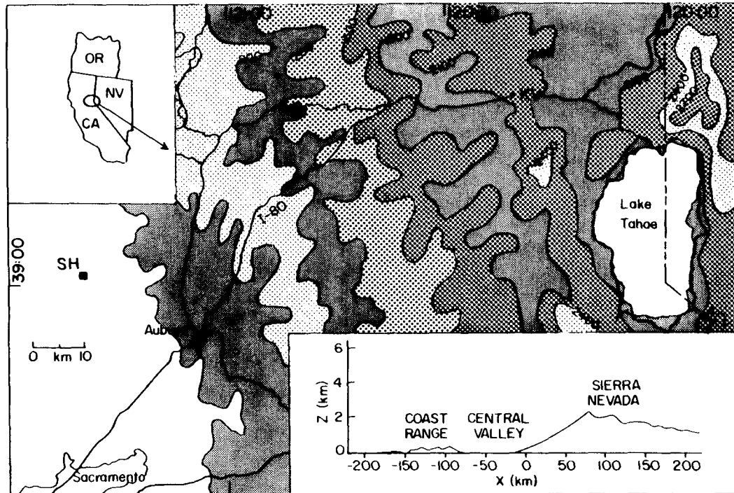
FIG. 1. Topographic map of the SPCP area (adapted from Rauber 1992), with a state map shown in the inset in the upper left, and a horizontal slice of topography used in simulation shown in the inset in the lower right.
