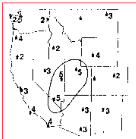
Figure 7—Haines Index map for 0600 MDT, August 2, 1989. Solid contour indicates a value of 5. (The Great Falls, MT, and Grand Junction, CO, data are missing for August 2, 1989.)
