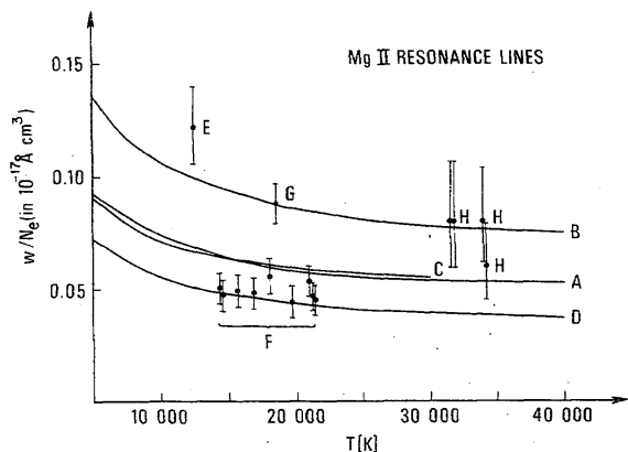
FIGURE 8. Measured and calculated (full) Stark halfwidths for the resonance lines of Mg II (2802.7 Å and 2795.5 Å), normalized to N_e = 10^{17} \text{ cm}^{-3} , as a function of temperature.
