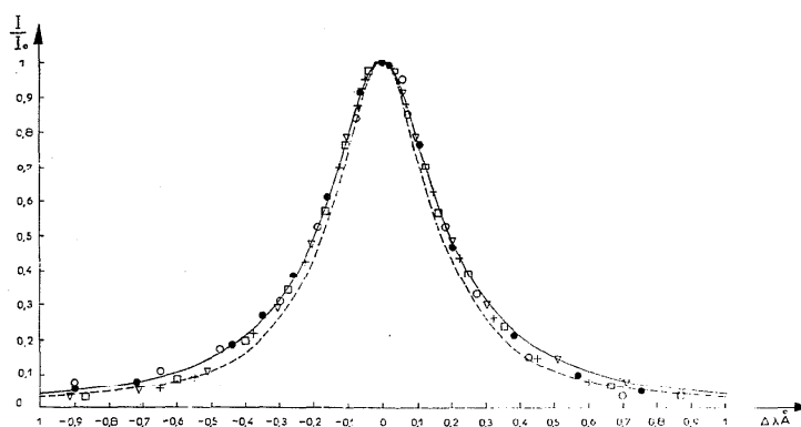
FIGURE 2. Stark profiles of five lines of the Ar II multiplet 4s^1P-4p^1D^o (+ 4330.18 Å, \nabla 4348.06 Å, \square 4331.20 Å, \circ 4379.67 Å, \bullet 4426.01 Å), from the measurements of Chapelle et al. [27]. The broken line is an (average) theoretical profile calculated according to a semiempirical theory by Griem [75].
