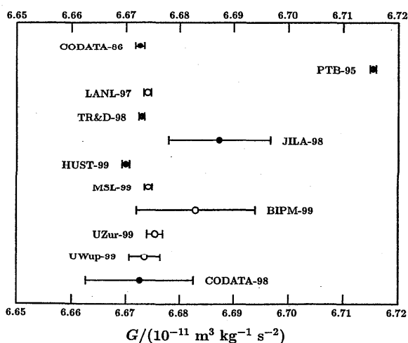
FIG. 1. Graphical comparison of the values of the Newtonian constant of gravitation G summarized in Table 13. An open circle indicates that the value is preliminary. (For the meanings of the identifying abbreviations in the figure, see the text.)
