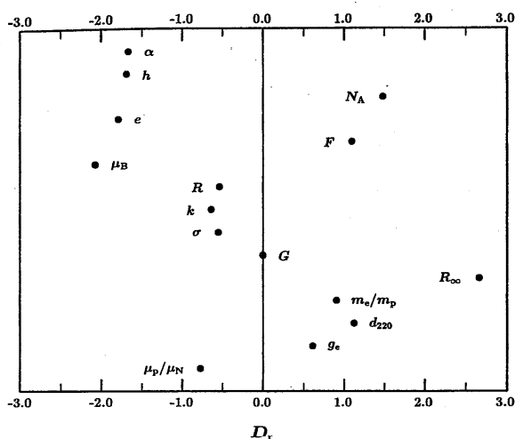
Fig. 5. Graphical comparison of the 1998 and 1986 CODATA recommended values of some of the constants listed in Table 31. As in that table, D_r is the 1998 value minus the 1986 value divided by the standard uncertainty u of the 1986 value (i.e., D_r is the change in the value of the constant from 1986 to 1998 relative to its 1986 standard uncertainty).
