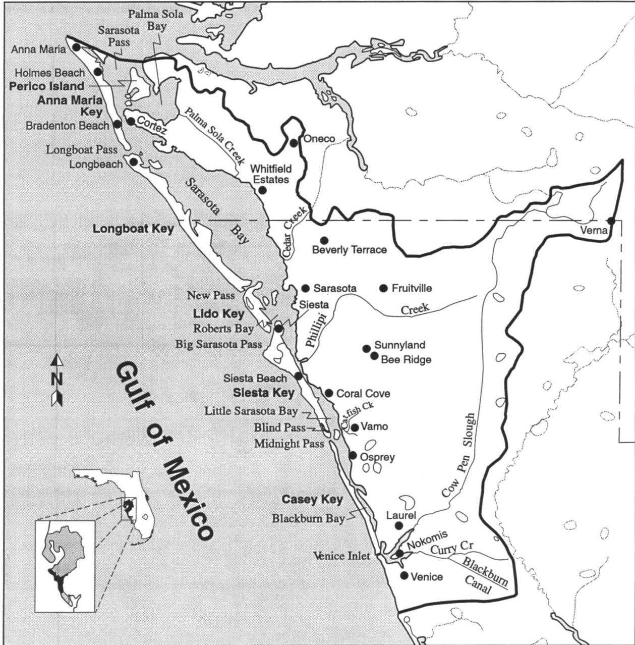
Figure 76. Upper Manasota coastal area drainage basin.
