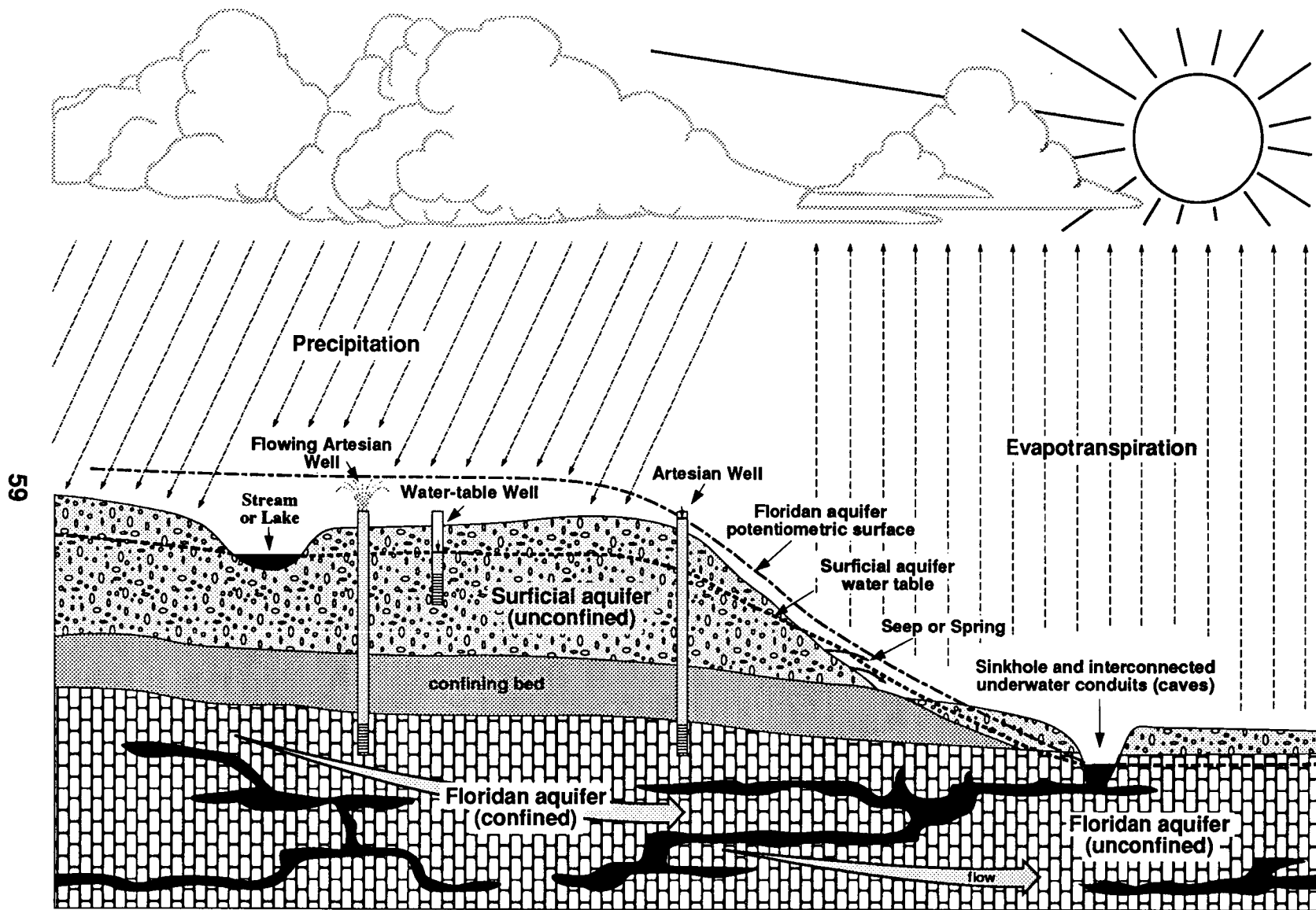
Figure 43. Generalized hydrogeologic relation between surficial and Floridan aquifers.
