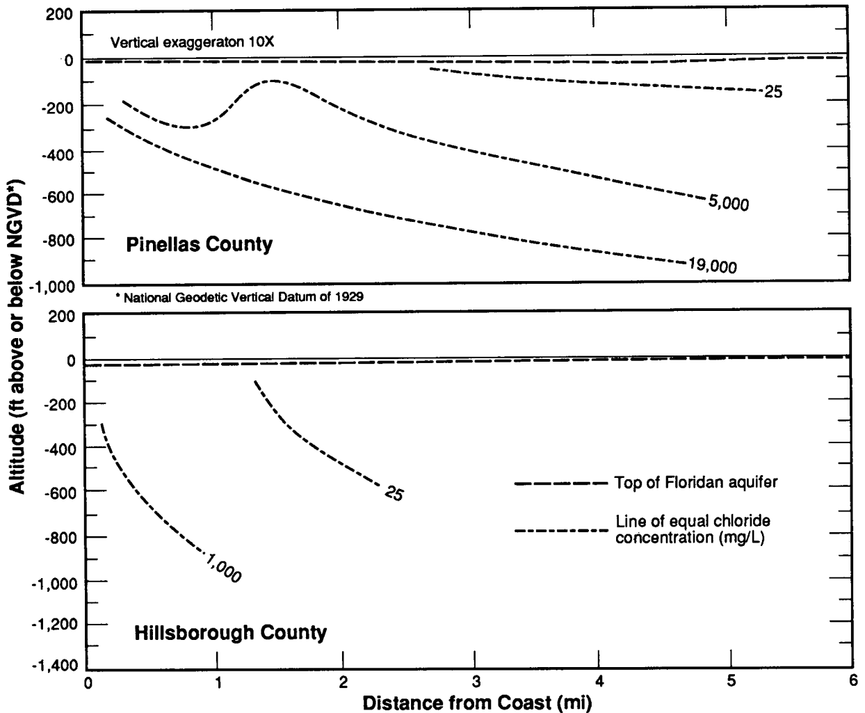
Figure 52. Section through Floridan aquifer showing chloride concentrations in the coastal margin of Pinellas and central Hillsborough County (after Causseaux and Fretwell 1983).
