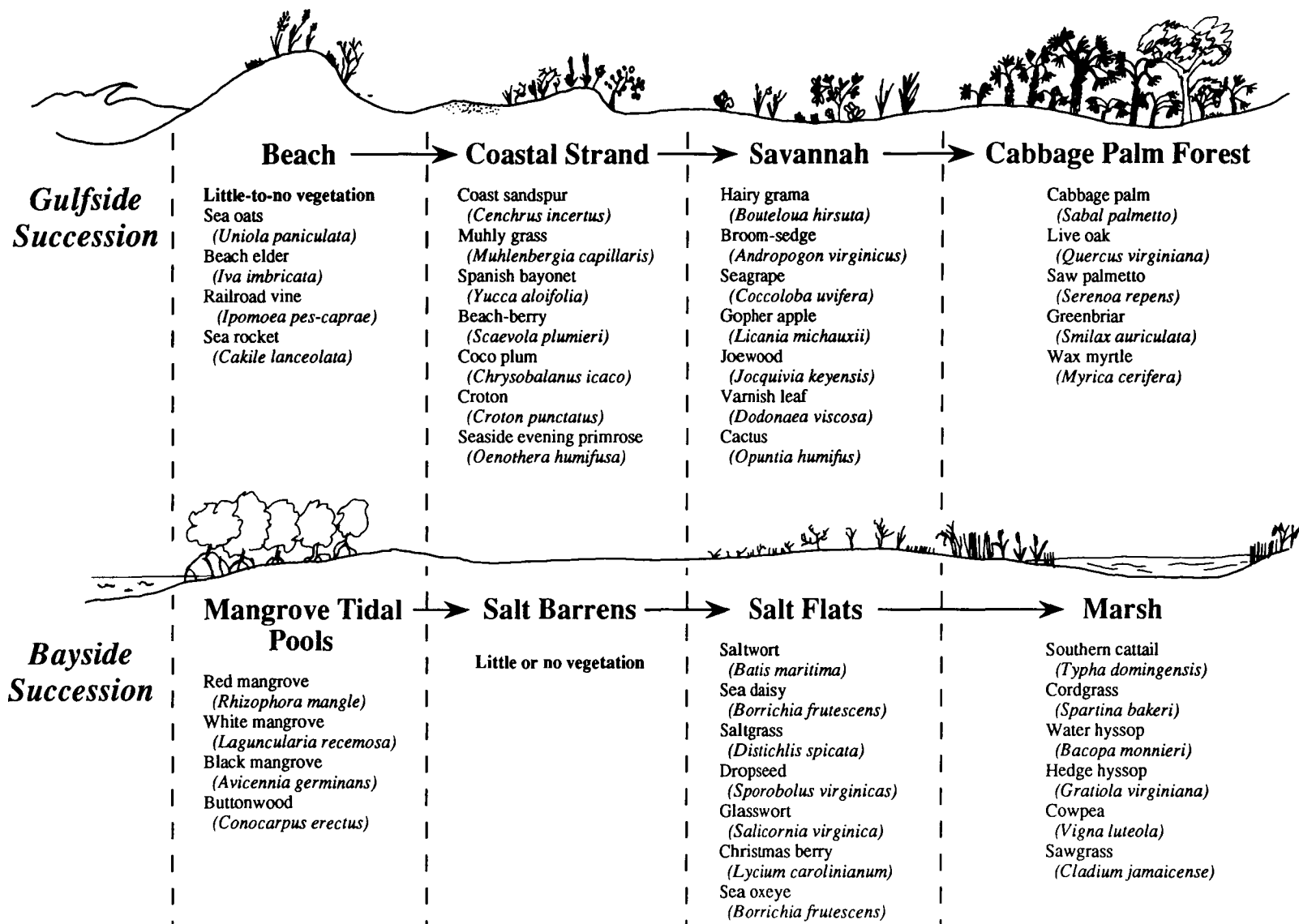
Figure 113. Two patterns of spatial succession of vegetation community types on west coast barrier islands.
