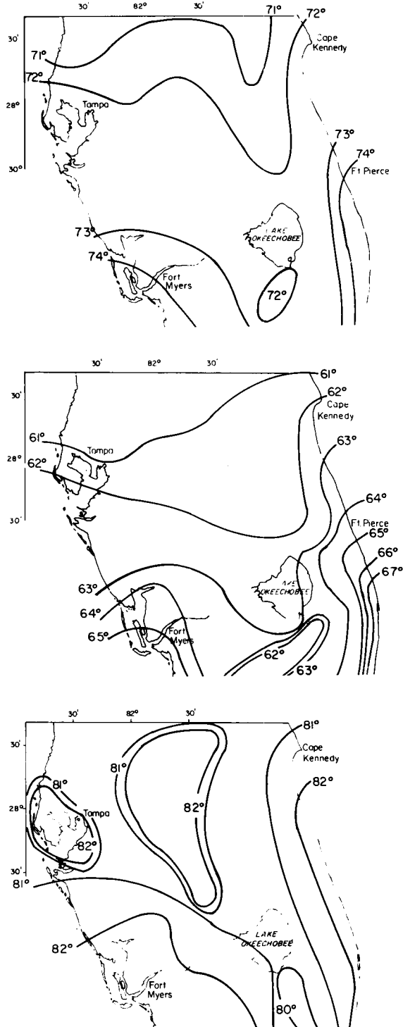
Figure 27. Annual, January, and August average temperatures ( ^{\circ}\text{F} ) in south-central Florida (after Thomas 1974).
