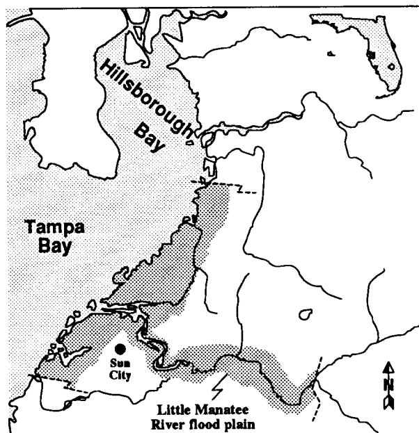
Figure 37. One-hundred-year hurricane flood surge in Little Manatee River (assuming mean annual river-discharge rate) (after Dames and Moore 1975).
