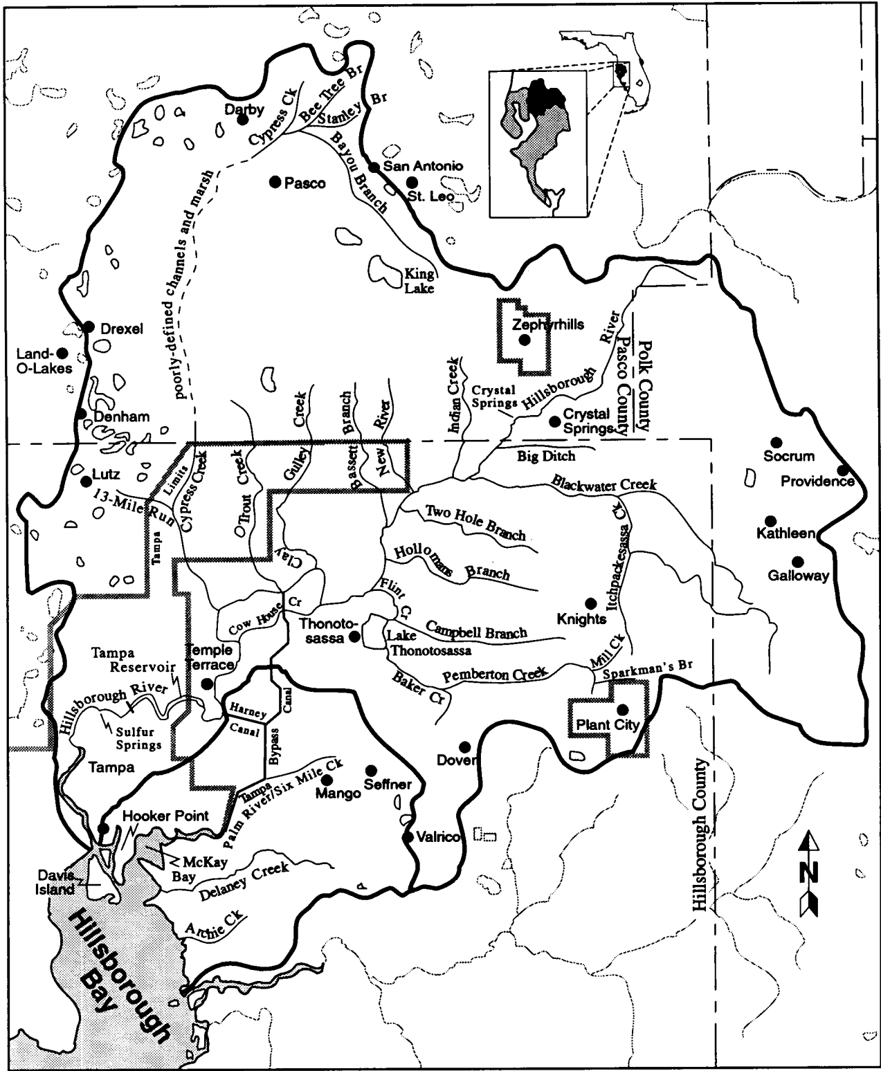
Figure 59. Hillsborough River and Tampa Bypass Canal drainage basins.
