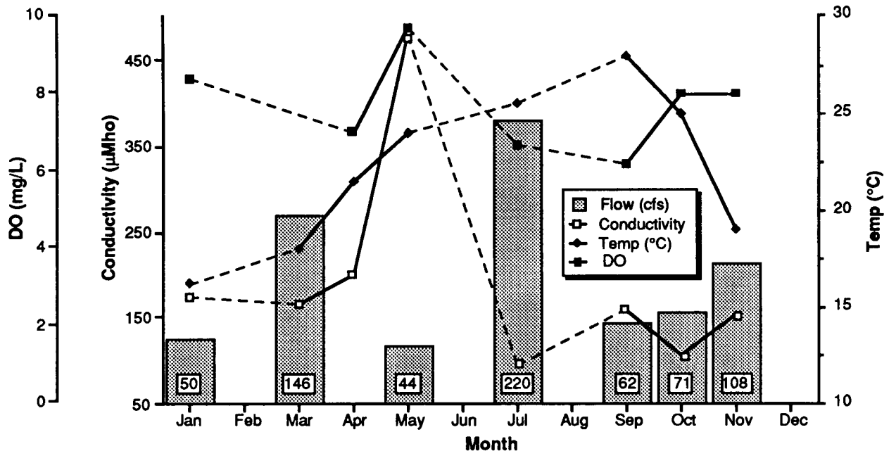
Figure 73. Seasonal water quality conditions in the Little Manatee River (after FDER 1982).
