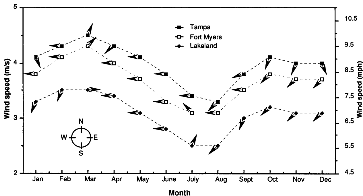
Figure 26. Prevailing wind speed and direction (data from Bradley 1974; TI 1978a).
