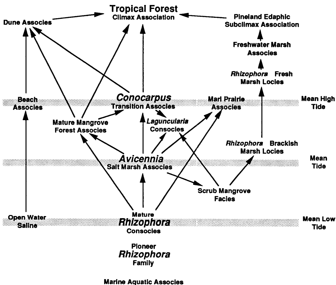
Figure 99. Successional relations of mangrove communities and some associated plant communities in relation to approximate tide levels (after Davis 1940).
