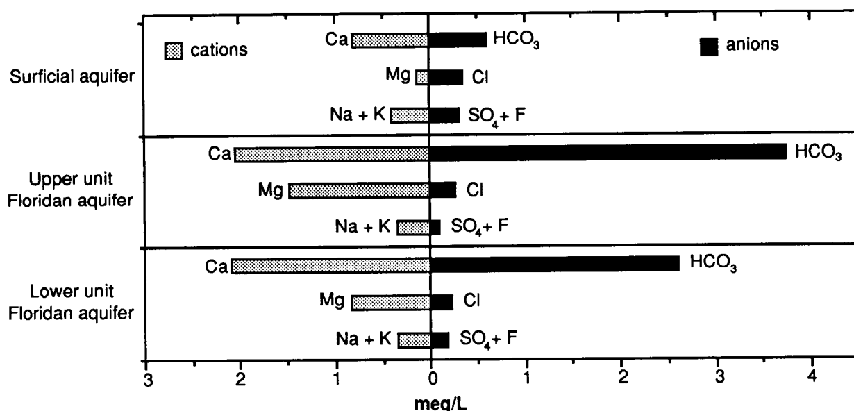
Figure 50. Median water quality in the surficial aquifer and upper and lower units of the Floridan aquifer (after Hutchinson 1978).
