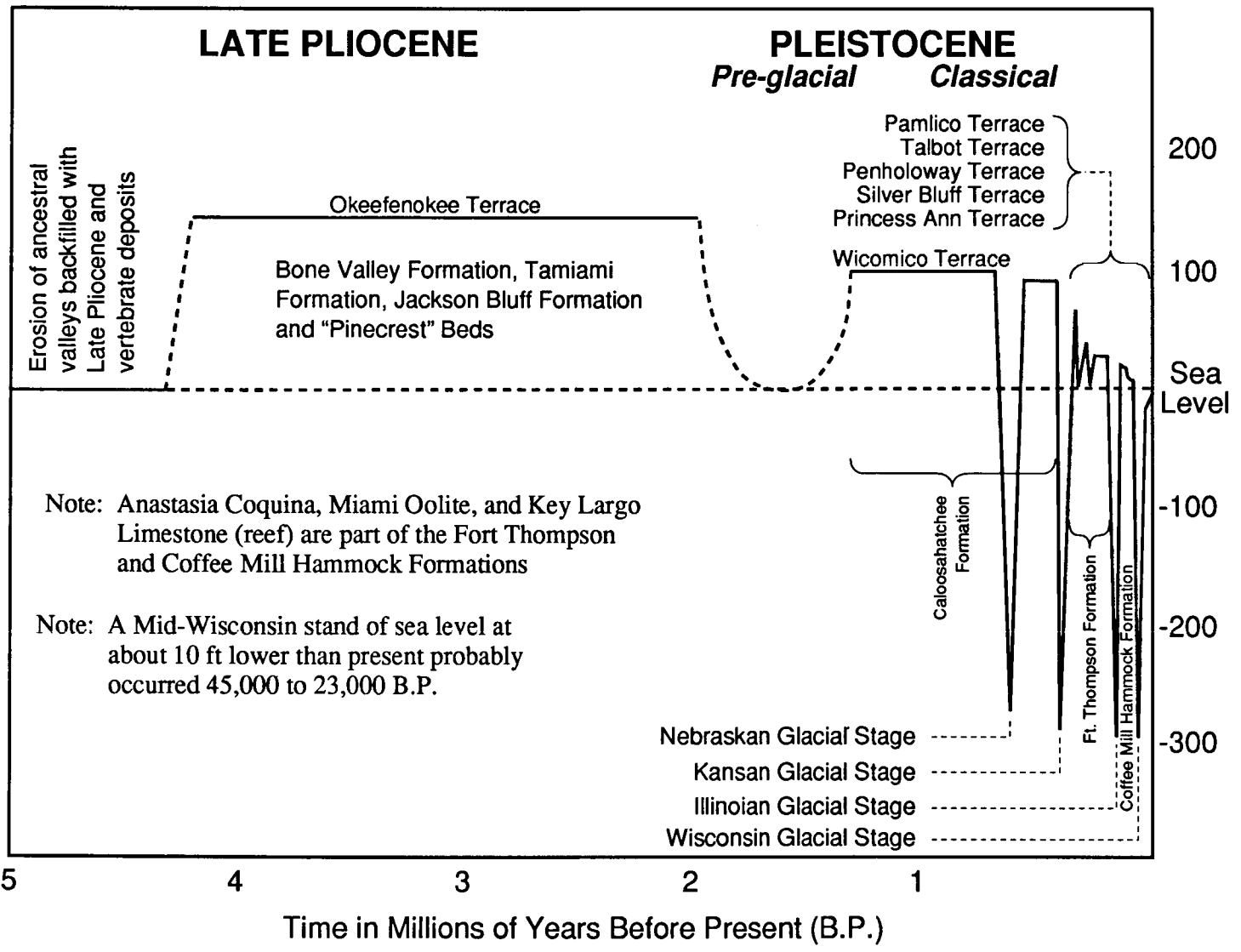
Figure 4. Glacial eustatic sea-level chronology for Florida (after Brooks 1968).
