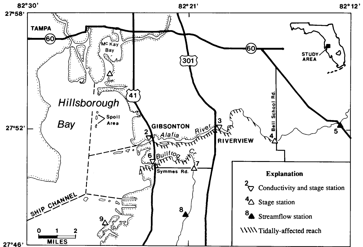
Figure 70. Conductivity, stage, and streamflow stations on Lower Alafia River and Bullfrog Creek (after Giovannelli 1981).
