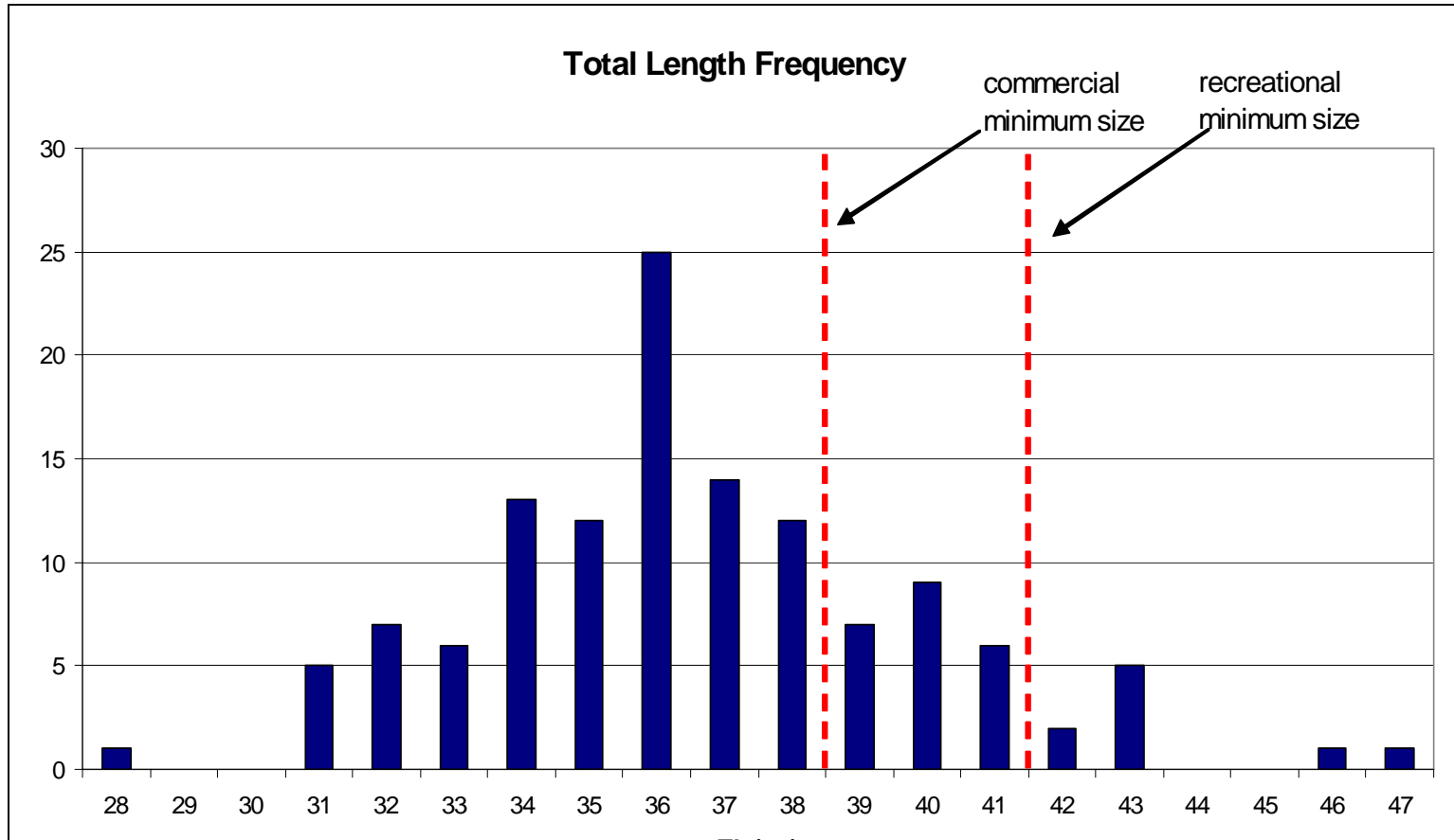
Figure 10. Histogram of the total length frequency of tagged red snapper (n=125).
