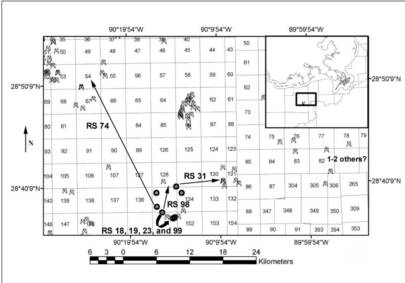
Figure 16. Map showing the starting and ending points for the seven red snapper that were recaptured at locations other than their release sites. The unconfirmed location where one or two other red snapper may have been recaptured and released east of the study area is also shown. RS 19 was last detected at ST135-M, but was ultimately recaptured at a different platform.
