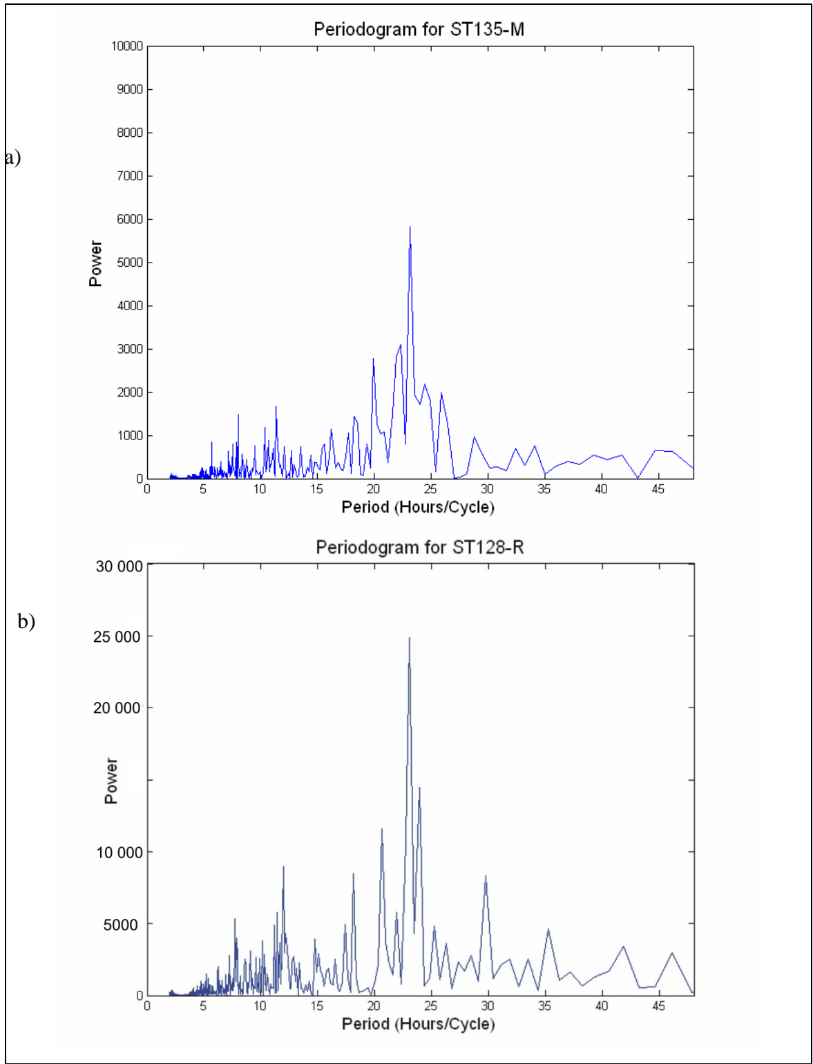
Figure 18. Periodograms for ST135-M (a) and ST128-R (b) showing the period and power of the sine functions describing red snapper movement away from the platforms.
