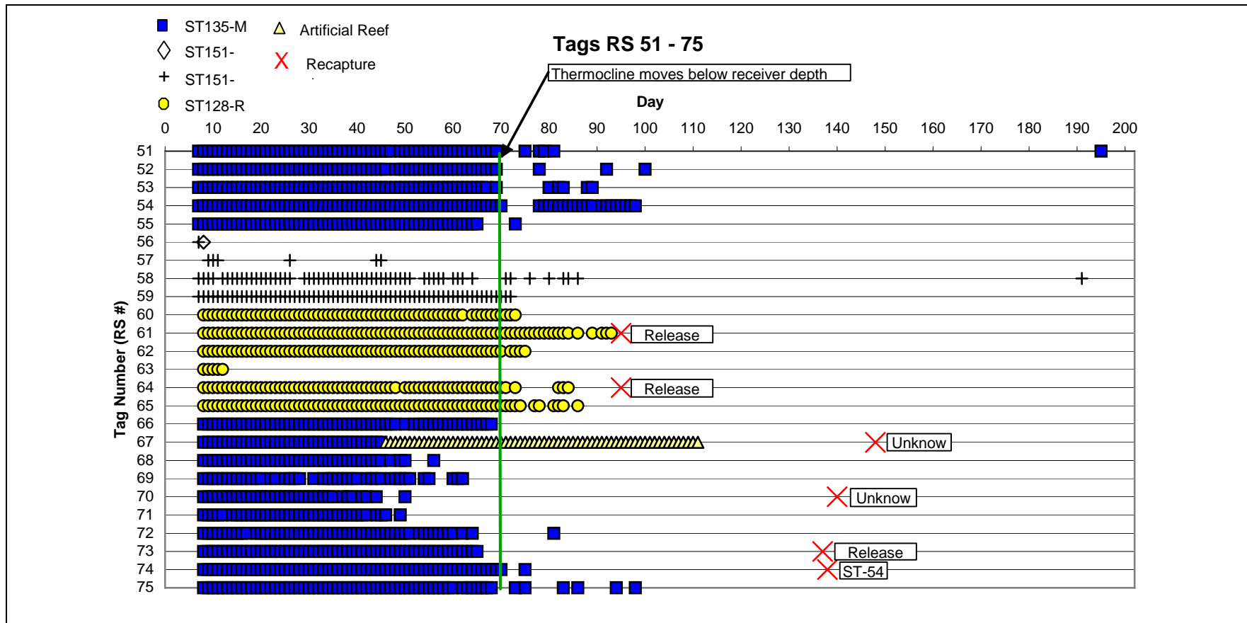
Figure 13. Daily locations of tagged red snapper RS 51 - 75. Different symbols represent different locations, dashed lines denote a period not covered by a receiver, X's and labels denote when and where a red snapper was recaptured, and the vertical line at day 70 denotes the suspected interference of the thermocline with ping detection.
