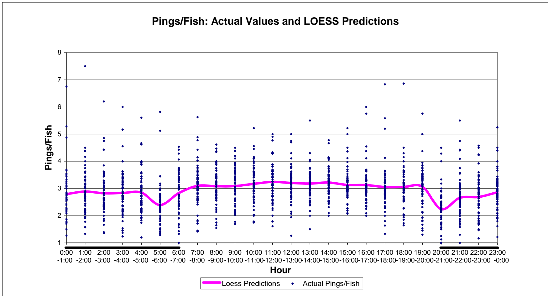
Figure 19. Actual values of pings/fish and LOESS predicted values of pings/fish for each hour of the day. The black bar below the x-axis denotes nighttime hours.
