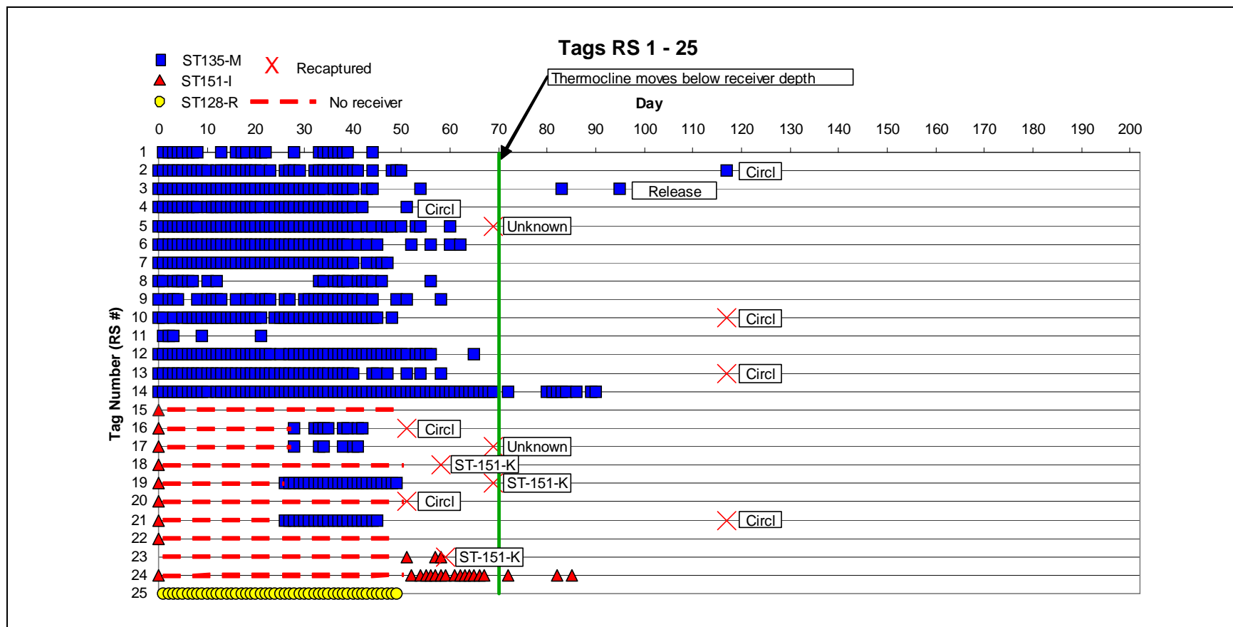
Figure 11. Daily locations of tagged red snapper RS 1 - 25. Different symbols represent different locations, dashed lines denote a period not covered by a receiver, X's and labels denote when and where a red snapper was recaptured, and the vertical line at day 70 denotes the suspected interference of the thermocline with ping detection.
