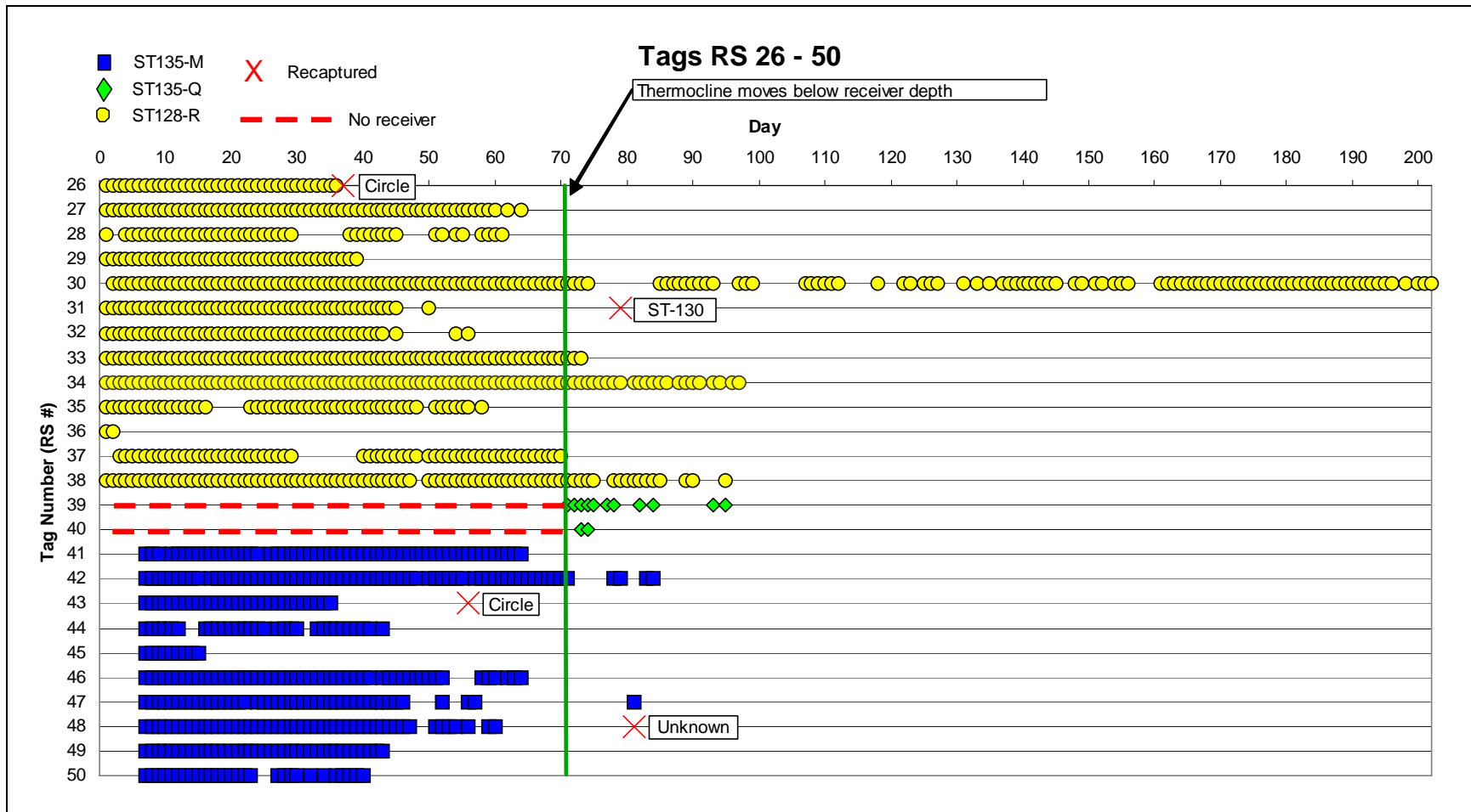
Figure 12. Daily locations of tagged red snapper RS 26 - 50. Different symbols represent different locations, dashed lines denote a period not covered by a receiver, X's and labels denote when and where a red snapper was recaptured, and the vertical line at day 70 denotes the suspected interference of the thermocline with ping detection.
