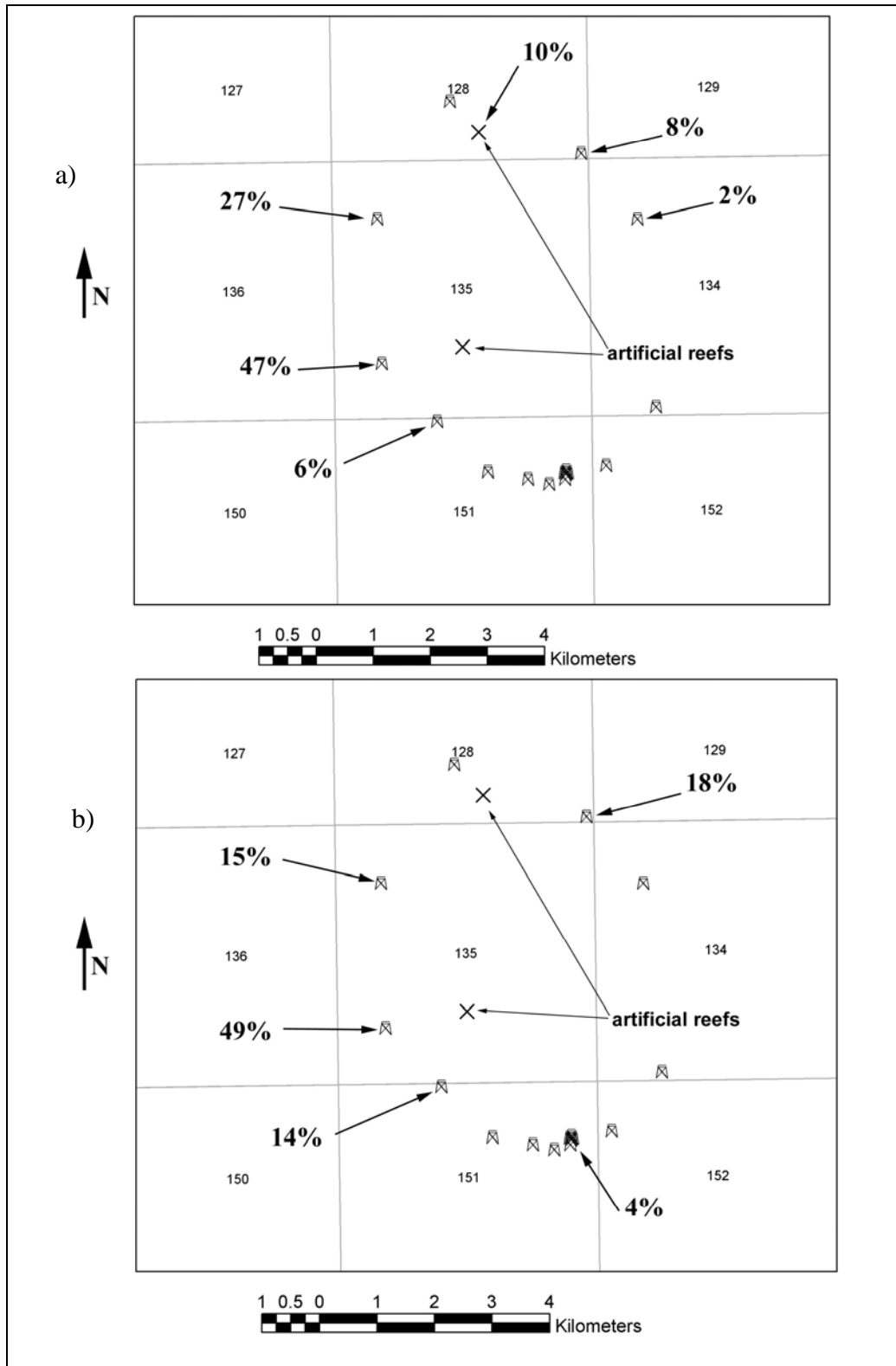
Figure 7. Capture (a) and release (b) locations for tagged red snapper are shown with the corresponding percent of total fish captured and released at each location.
