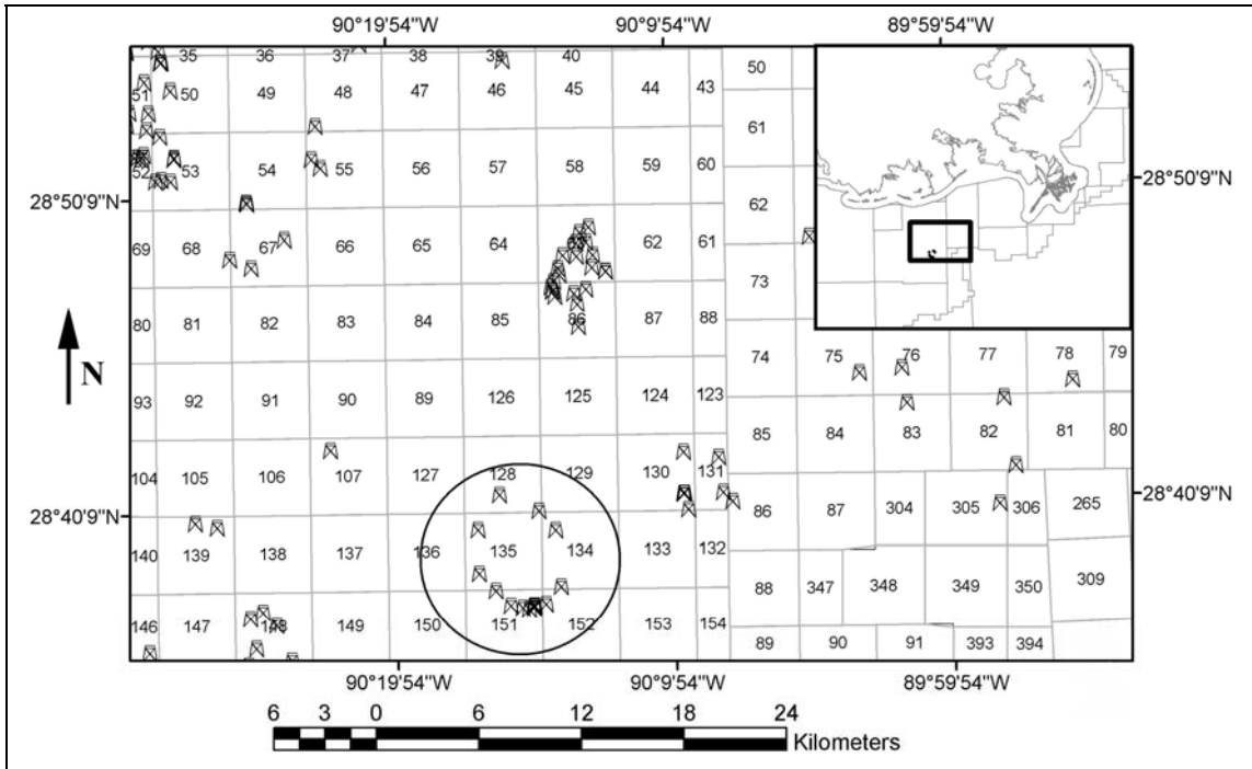
Figure 1. Map of the study area in the MMS South Timbalier Blocks 128, 134, 135, 151, and 152. The inset in the upper right corner shows the location of the study area with respect to the coast of Louisiana.
