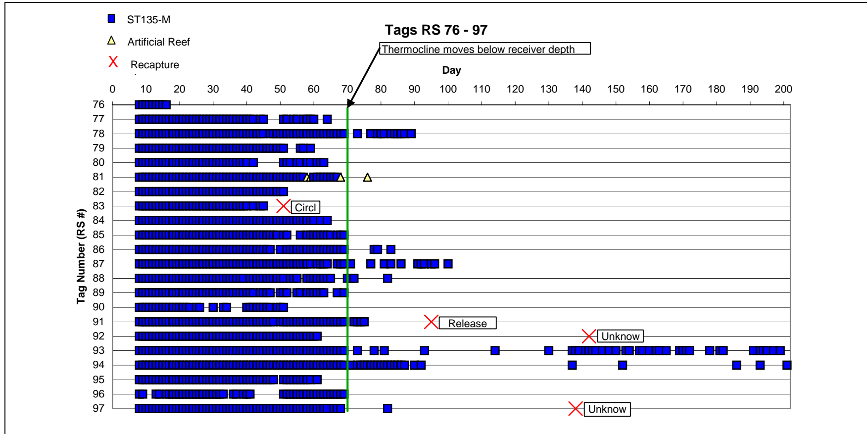
Figure 14. Daily locations of tagged red snapper RS 76 - 97. Different symbols represent different locations, dashed lines denote a period not covered by a receiver, X's and labels denote when and where a red snapper was recaptured, and the vertical line at day 70 denotes the suspected interference of the thermocline with ping detection.
