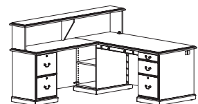
Footprint: 68" w x 79" d x 45" h
