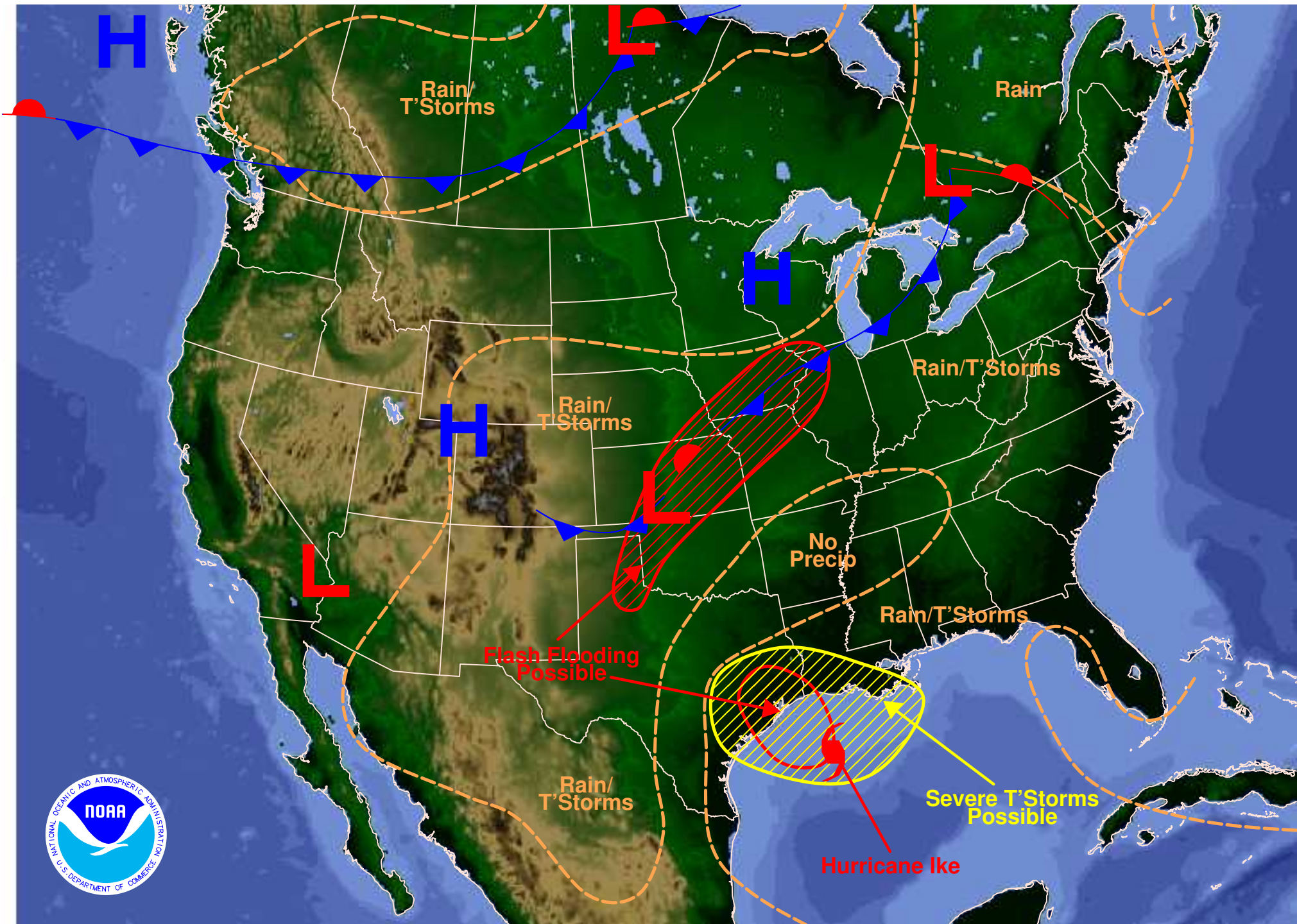
Weather Forecast for Friday, September 12, 2008 DOC/NOAA/NWS/NCEP/Hydrometeorological Prediction Center Prepared by Kost based on HPC, SPC, and TPC forecasts.
