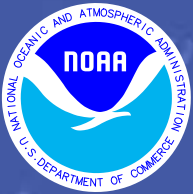
Weather Forecast for Thursday, September 04, 2008 DOC/NOAA/NWS/NCEP/Hydrometeorological Prediction Center Prepared by Kong based on HPC, SPC, and TPC forecasts.
