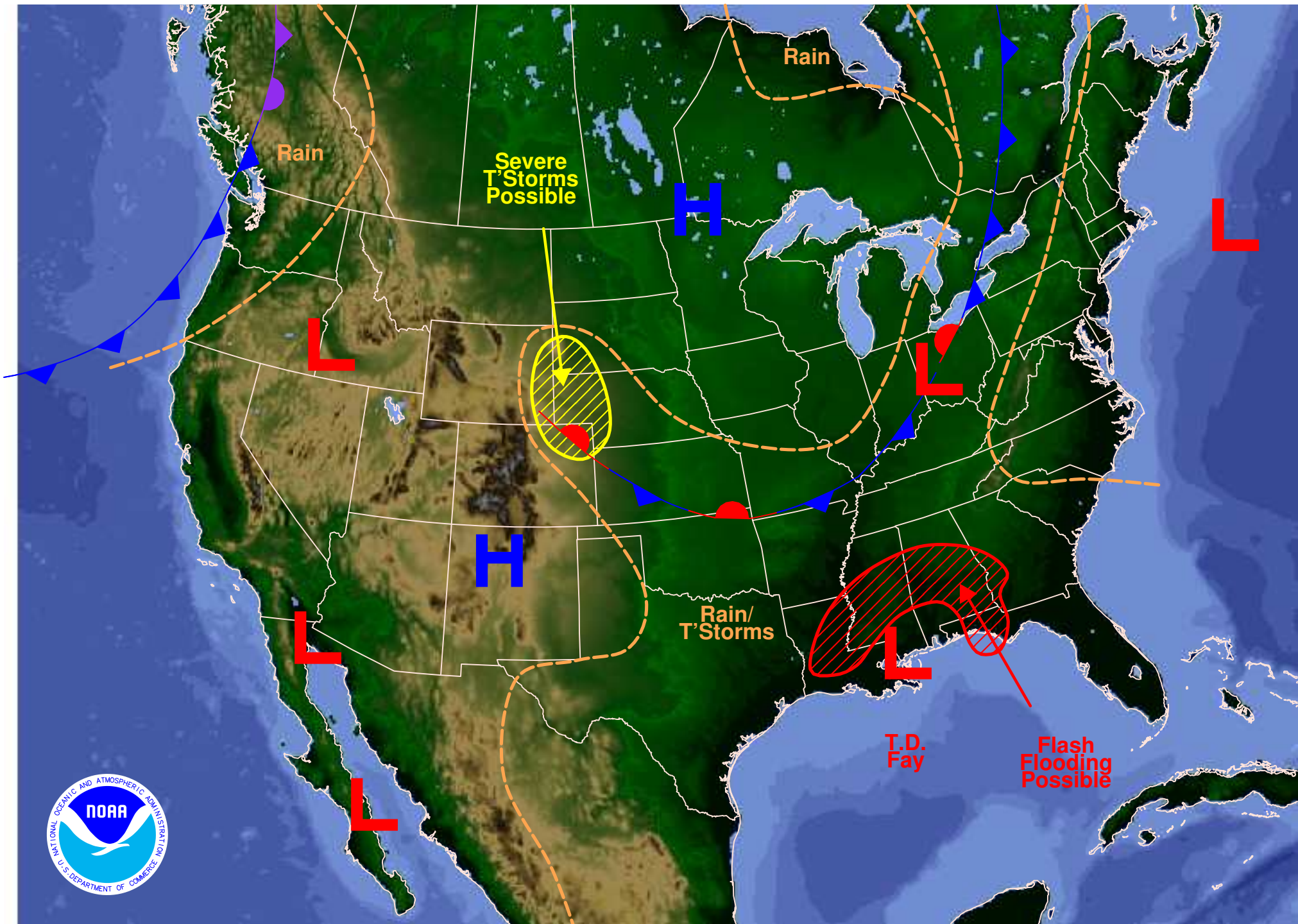
Weather Forecast for Sunday, August 24, 2008 DOC/NOAA/NWS/NCEP/Hydrometeorological Prediction Center Prepared by Fracasso based on HPC, SPC, and TPC forecasts.
